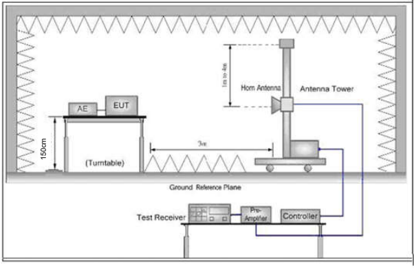
Figure 3. Above 1 GHz
