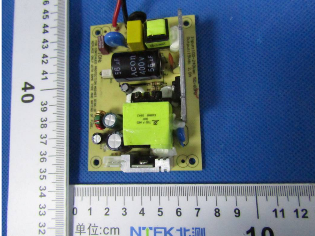
Photo 15 (1#Power board)
