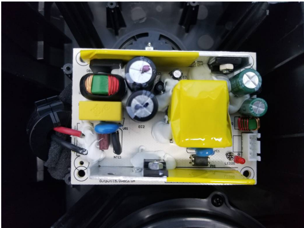
Photo 8 (2# Power board)
