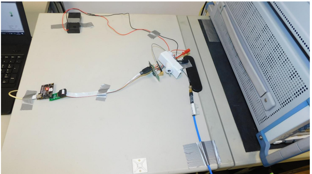
Picture 8: Conducted measurements
