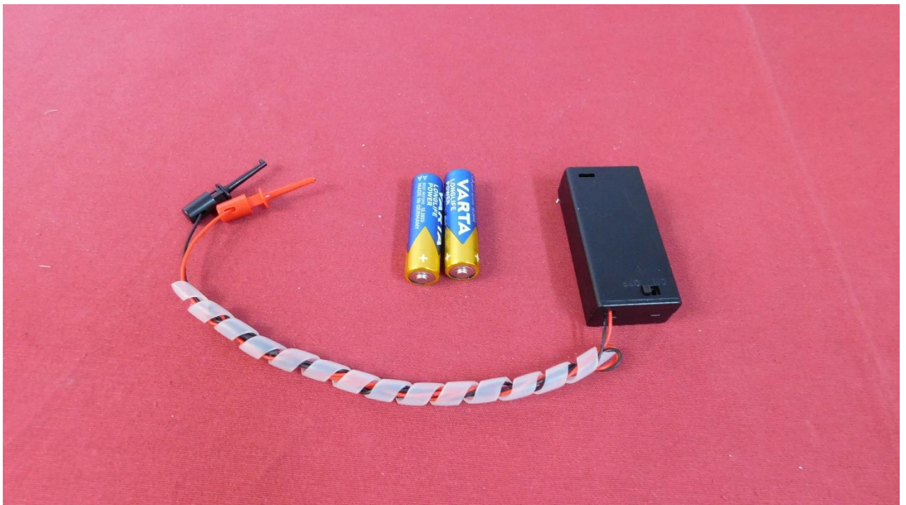
Picture 12: Power supply
