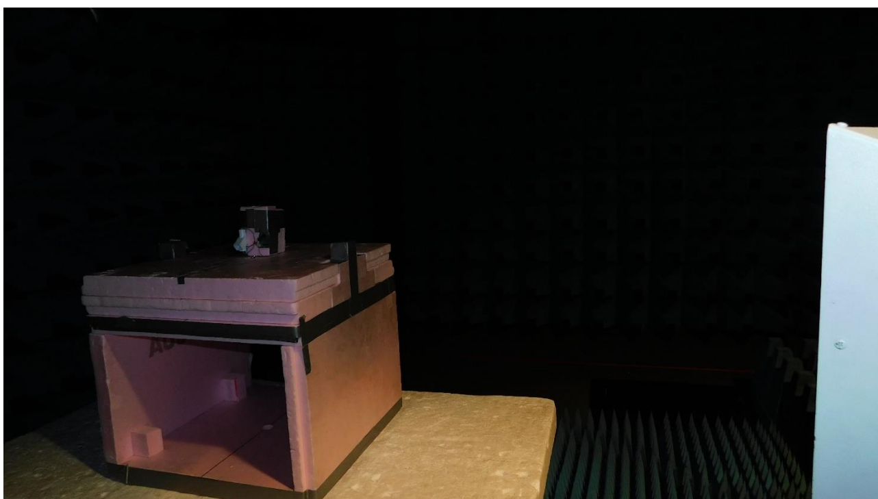
Picture 6: FS-SAC, radiated emission test 1 GHz – 17 GHz (rear view)
