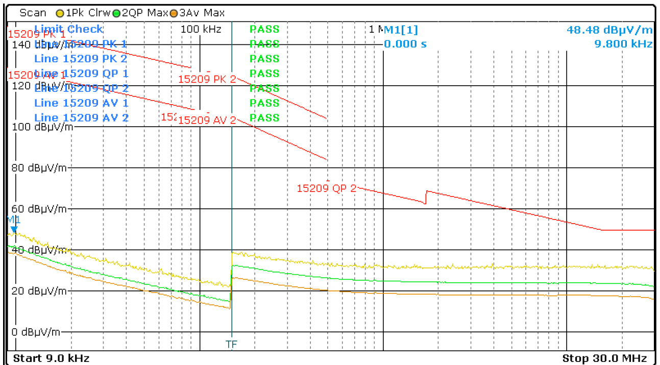
Figure 34: Chart of emissions test below 30 MHz on highest channel, EUT position X, antenna parallel
