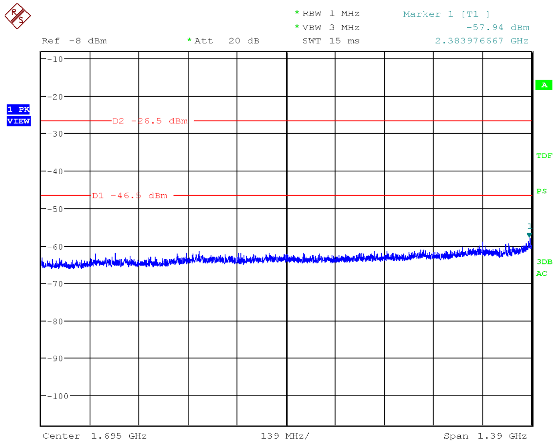
Figure 29: Chart of emissions test from 1 GHz to 2.39 GHz on highest channel, PK-detector
