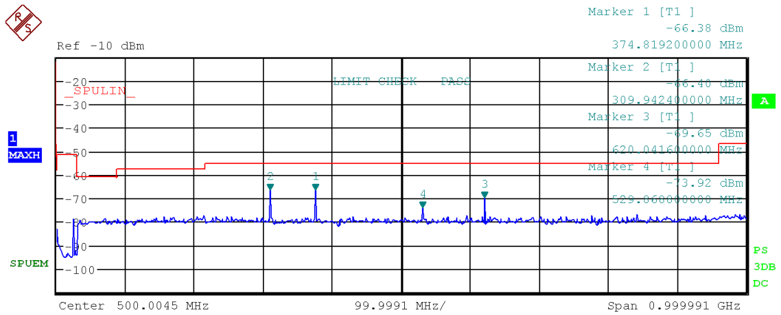
Figure 28: Chart of emissions test from 9 kHz to 1 GHz on highest channel, PK-detector
