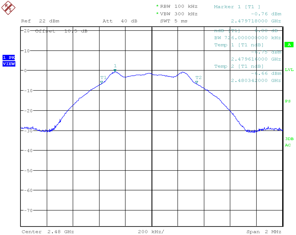
Figure 8: Chart of 6 dB bandwidth test on highest channel
