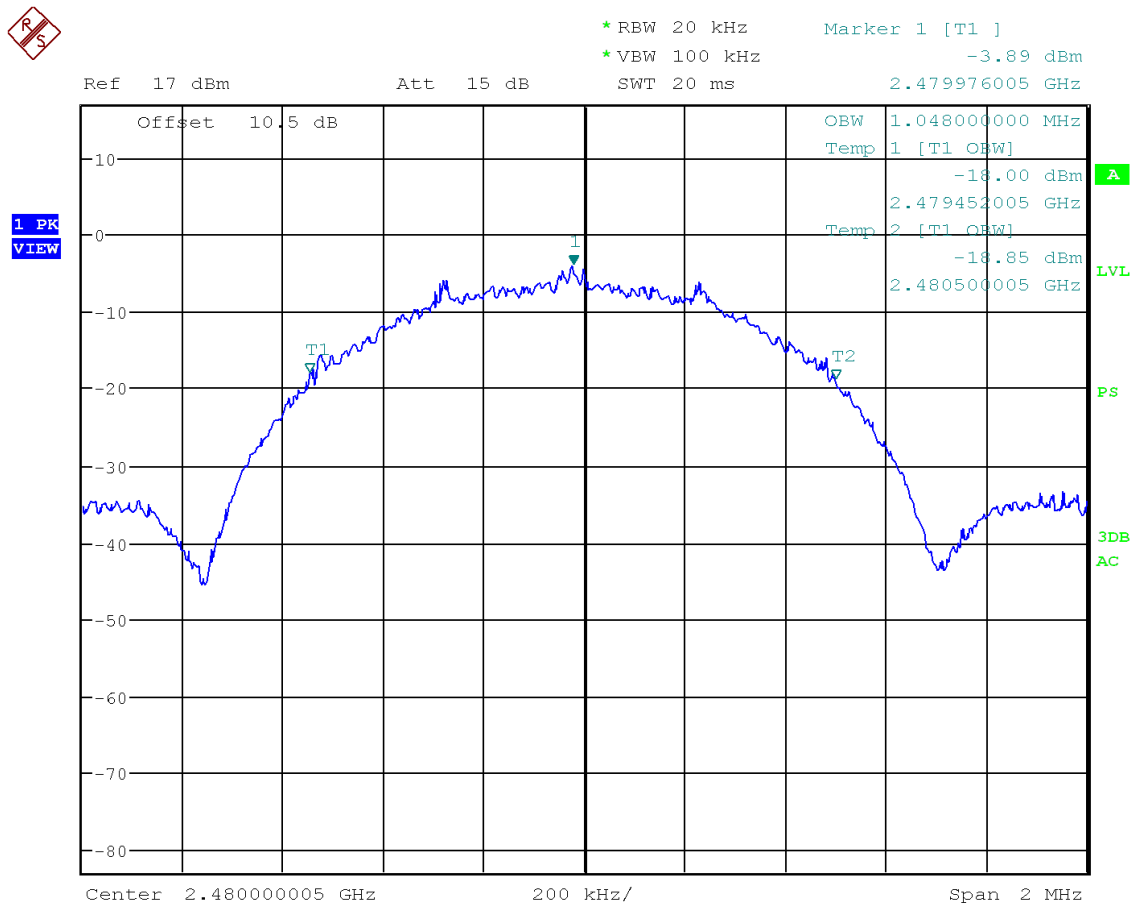
Figure 11: Chart of occupied bandwidth test on highest channel
