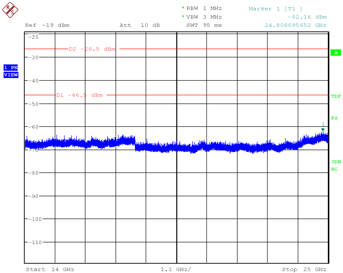
Figure 27: Chart of emissions test from 14 GHz to 25 GHz on middle channel, PK-detector
