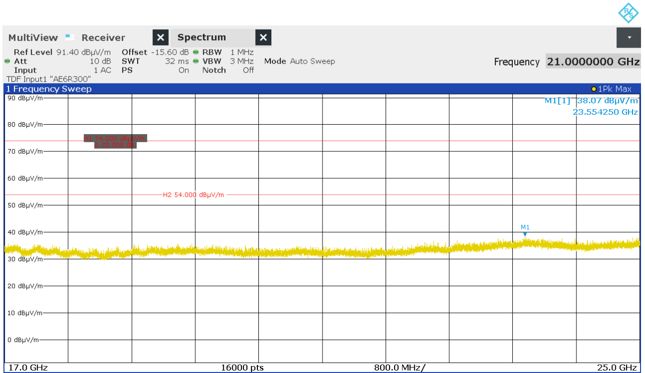
Figure 39: Chart of exploratory radiated emissions measurement from 17 GHz to 25 GHz on lowest channel, EUT position X, antenna polarization vertical
