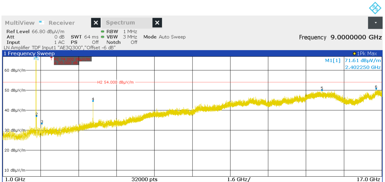
Figure 38: Chart of radiated emissions pre-measurement from 1 GHz to 17 GHz on lowest channel, EUT position Y, antenna polarization horizontal
