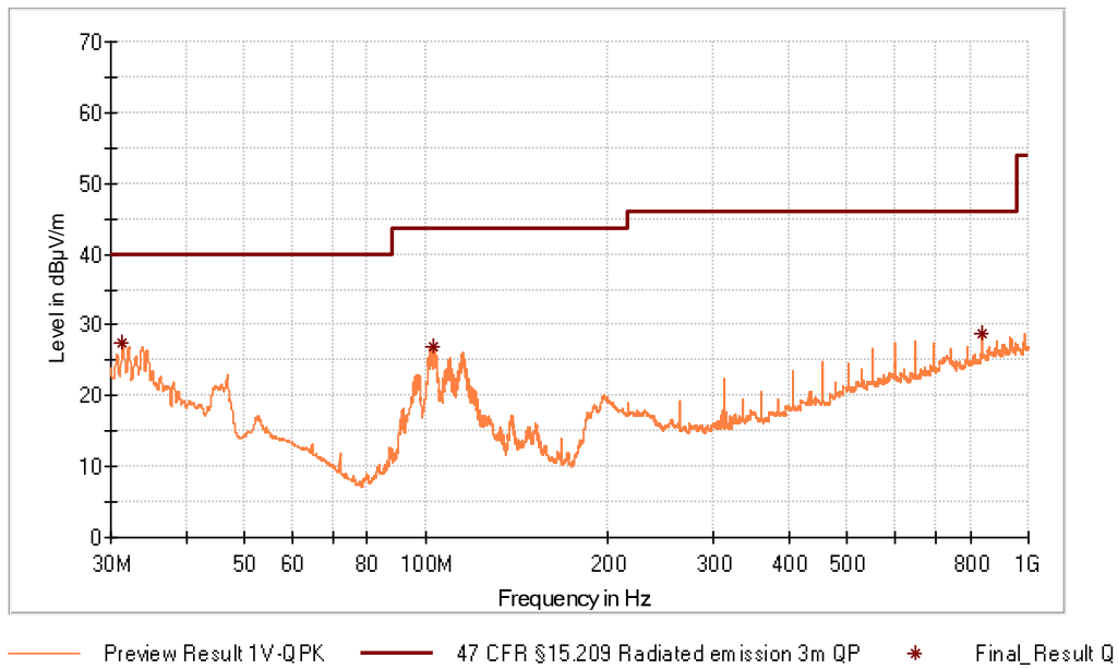
Figure 37: Chart of radiated emissions test from 30 MHz to 1 GHz on highest channel, EUT position X, antenna polarization vertical
