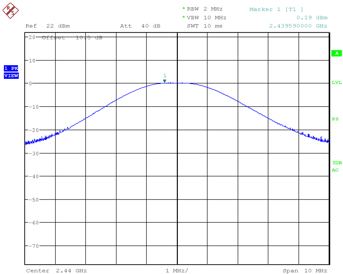
Figure 13: Chart of conducted output power on middle channel
