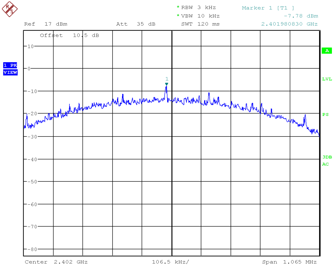
Figure 15: Chart of power spectral density on lowest channel
