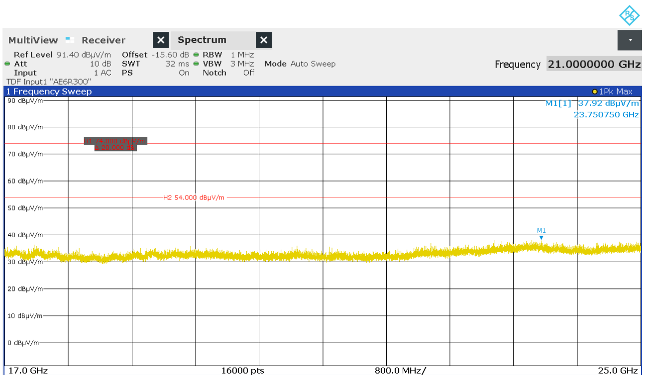
Figure 43: Chart of exploratory emission test from 17 GHz to 25 GHz on highest channel at 0.5 m, EUT position X, antenna polarization vertical
