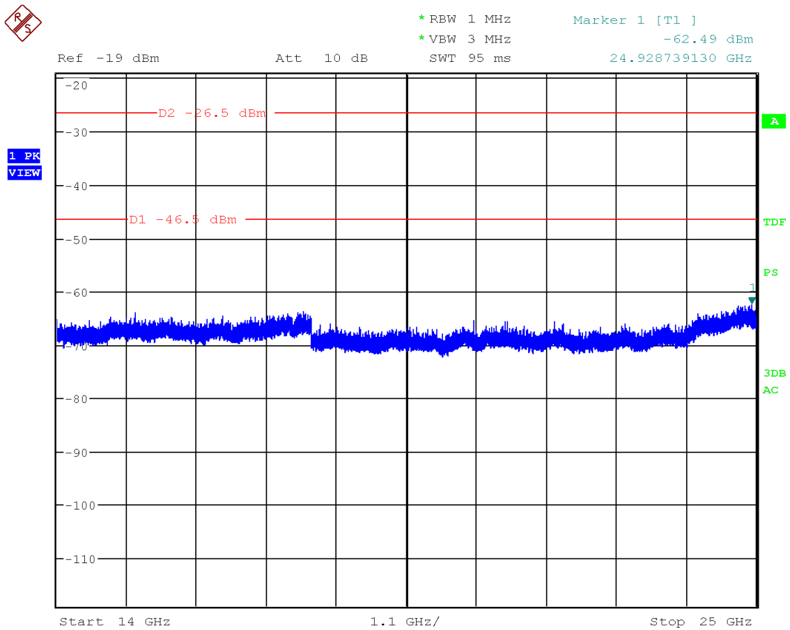
Figure 31: Chart of emissions test from 14 GHz to 25 GHz on highest channel, PK-detector
