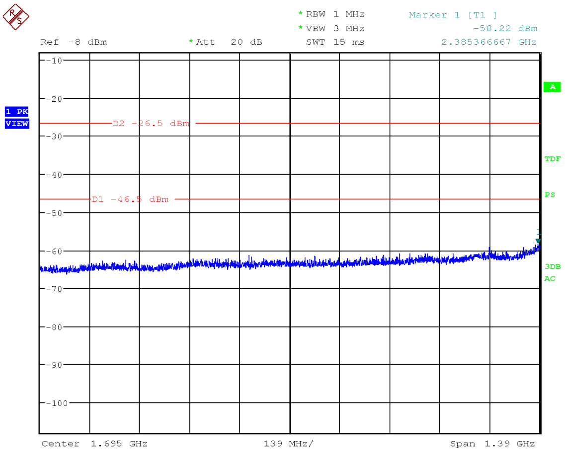
Figure 25: Chart of emissions test from 1 GHz to 2.39 GHz on middle channel, PK-detector
