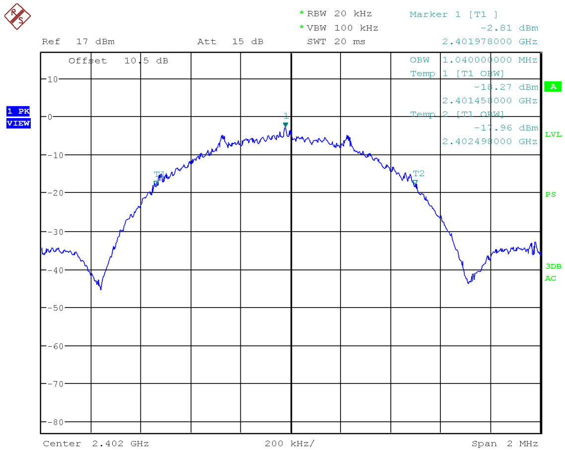
Figure 9: Chart of occupied bandwidth test on lowest channel
