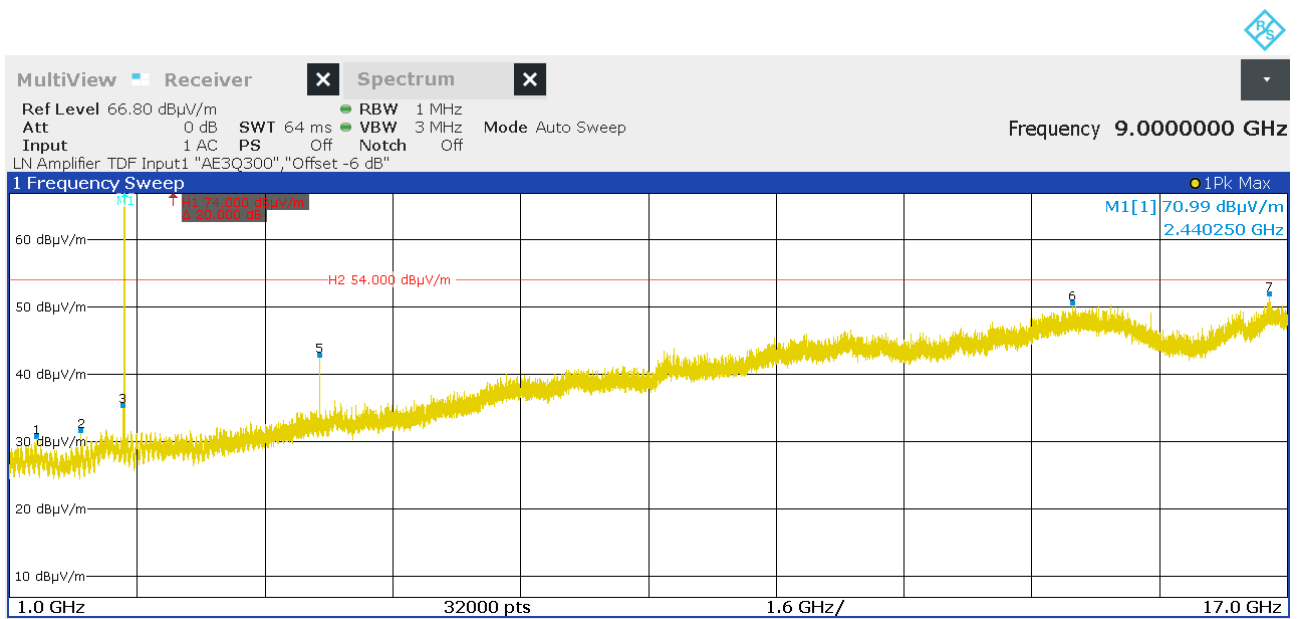
Figure 40: Chart of radiated emissions pre-measurement from 1 GHz to 17 GHz on middle channel, EUT position Y, antenna polarization horizontal
