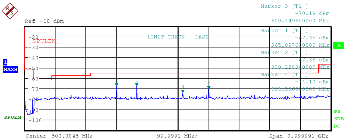
Figure 20: Chart of emissions test from 9 kHz to 1 GHz on lowest channel, PK-detector
