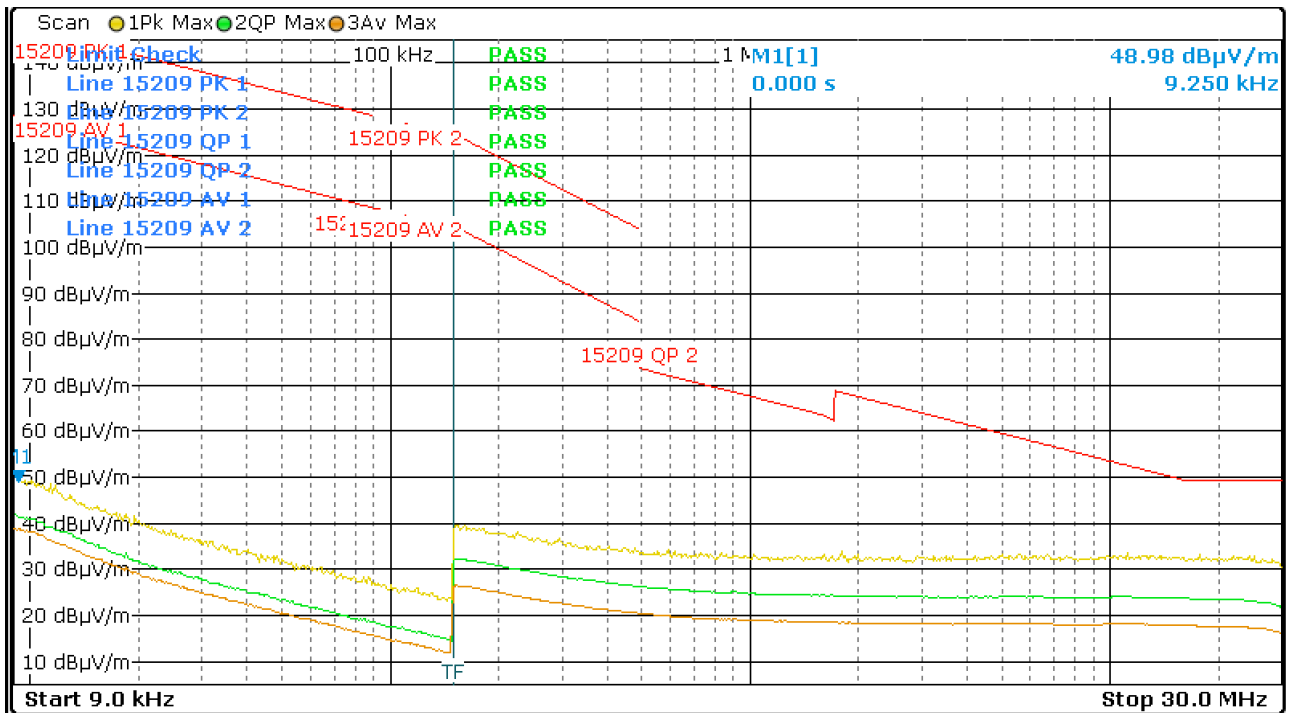
Figure 32: Chart of emissions test below 30 MHz on lowest channel, EUT position X, antenna parallel
