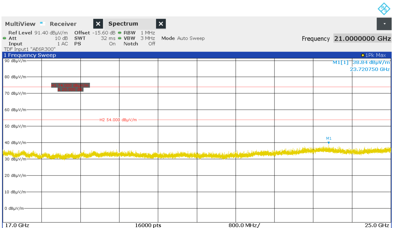
Figure 41: Chart of exploratory emissions measurement from 17 GHz to 25 GHz on middle channel, EUT position X, antenna polarization vertical
