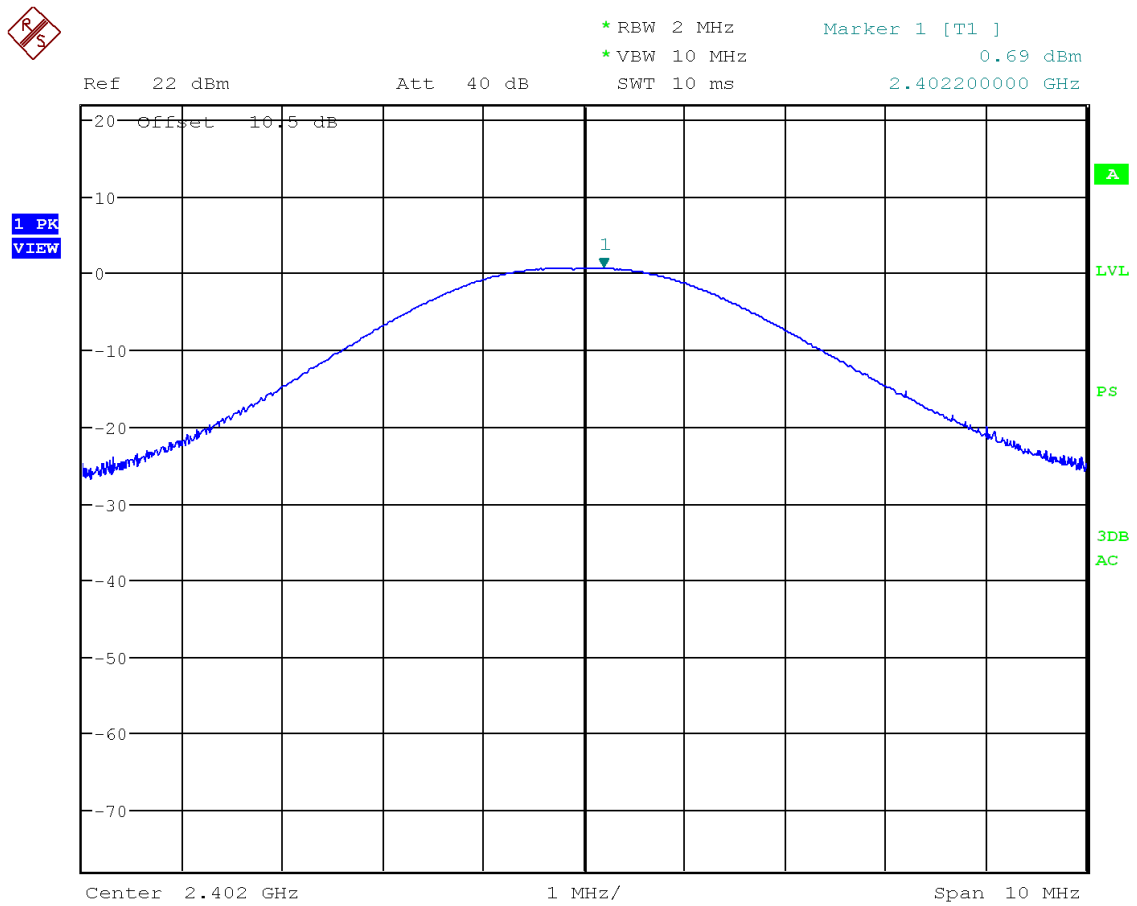
Figure 12: Chart of conducted output power on lowest channel
