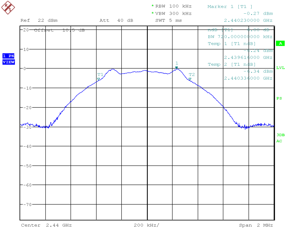
Figure 7: Chart of 6 dB bandwidth test on middle channel
