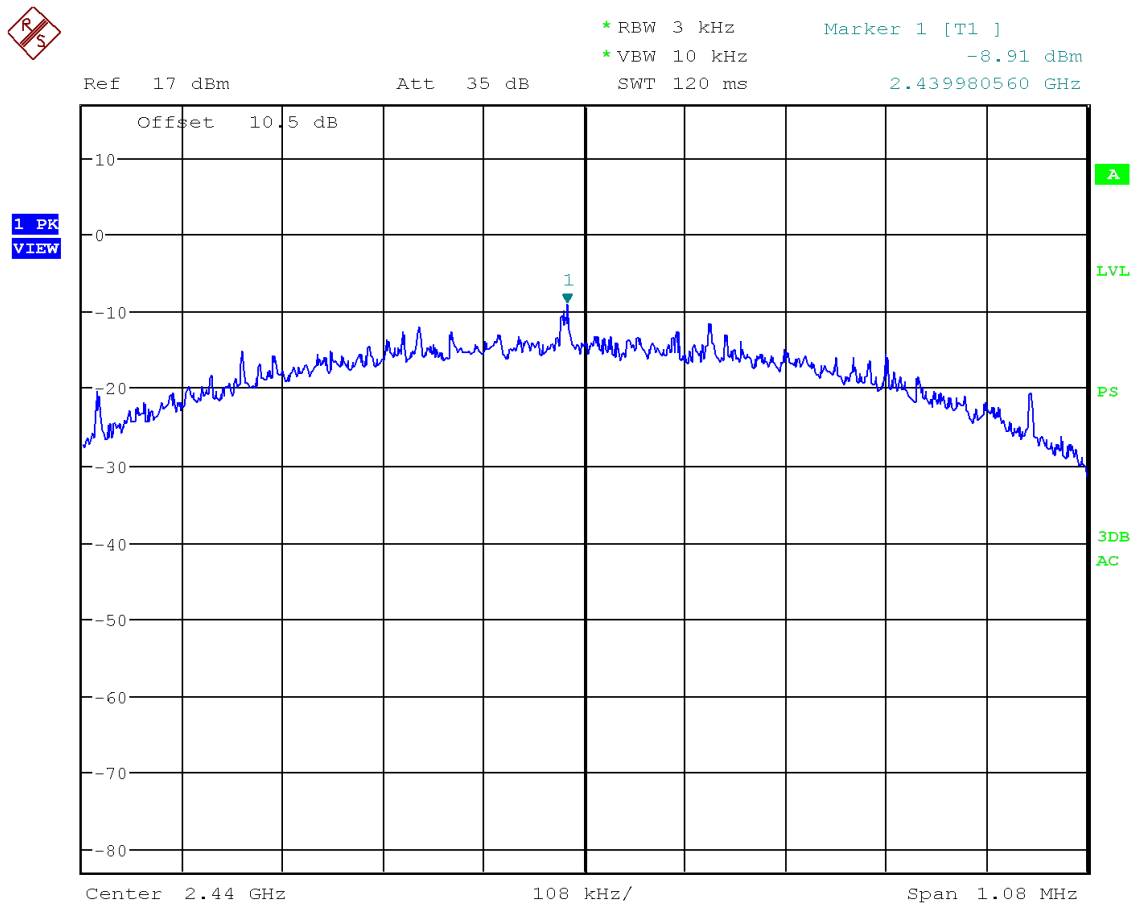
Figure 16: Chart of power spectral density on middle channel
