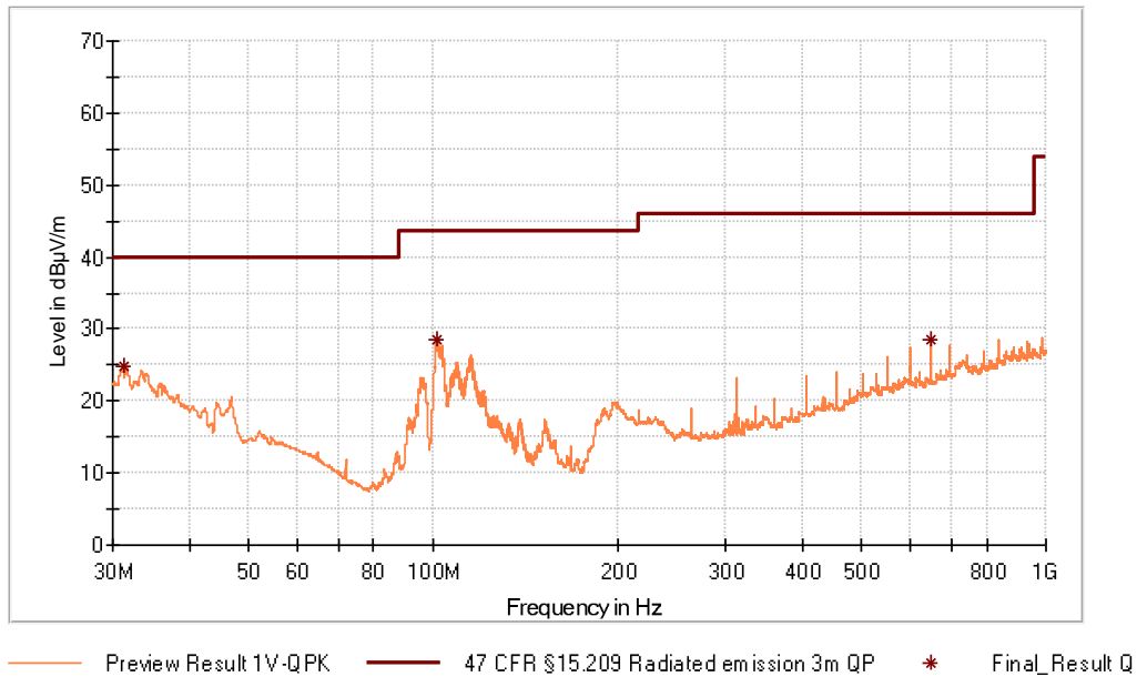
Figure 36: Chart of radiated emissions test from 30 MHz to 1 GHz on middle channel, EUT position X, antenna polarization vertical
