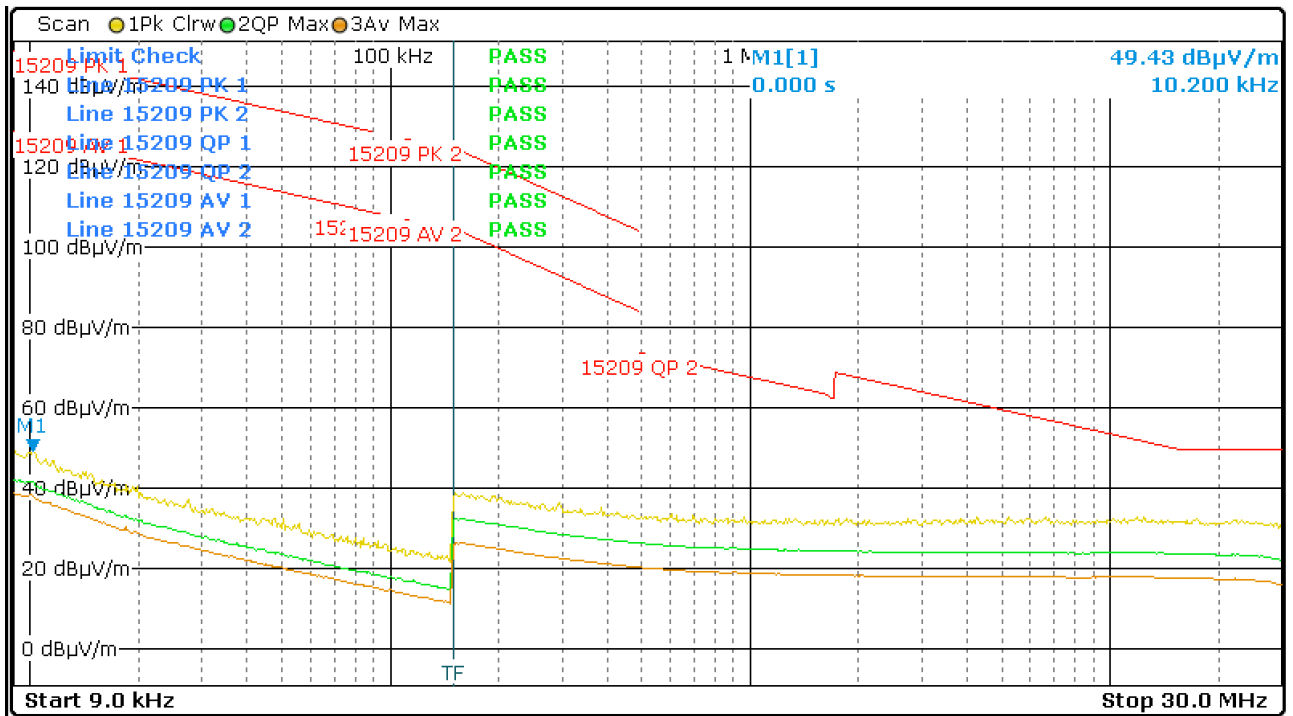
Figure 33: Chart of emissions test below 30 MHz on middle channel, EUT position X, antenna parallel
