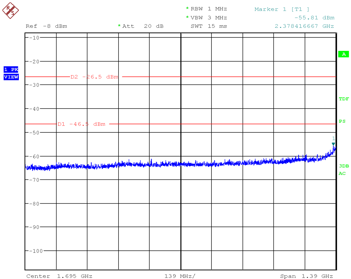
Figure 21: Chart of emissions test from 1 GHz to 2.39 GHz on lowest channel, PK-detector
