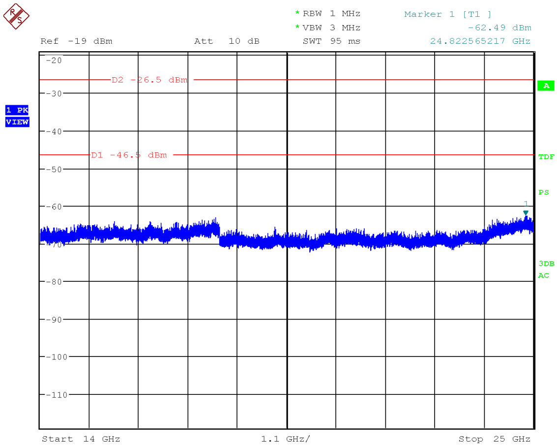
Figure 23: Chart of emissions test from 14 GHz to 25 GHz on lowest channel, PK-detector
