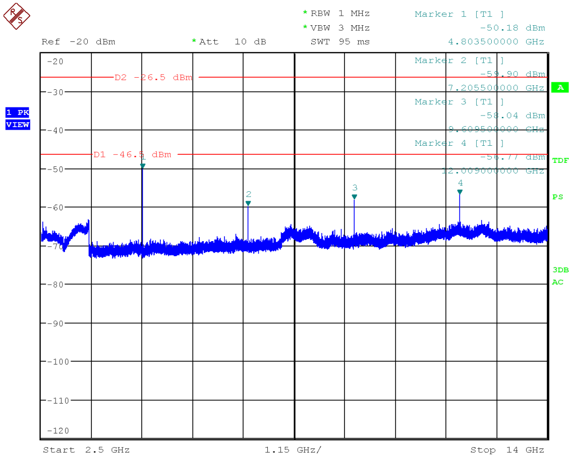
Figure 22: Chart of emissions test from 2.5 GHz to 14 GHz on lowest channel, PK-detector
