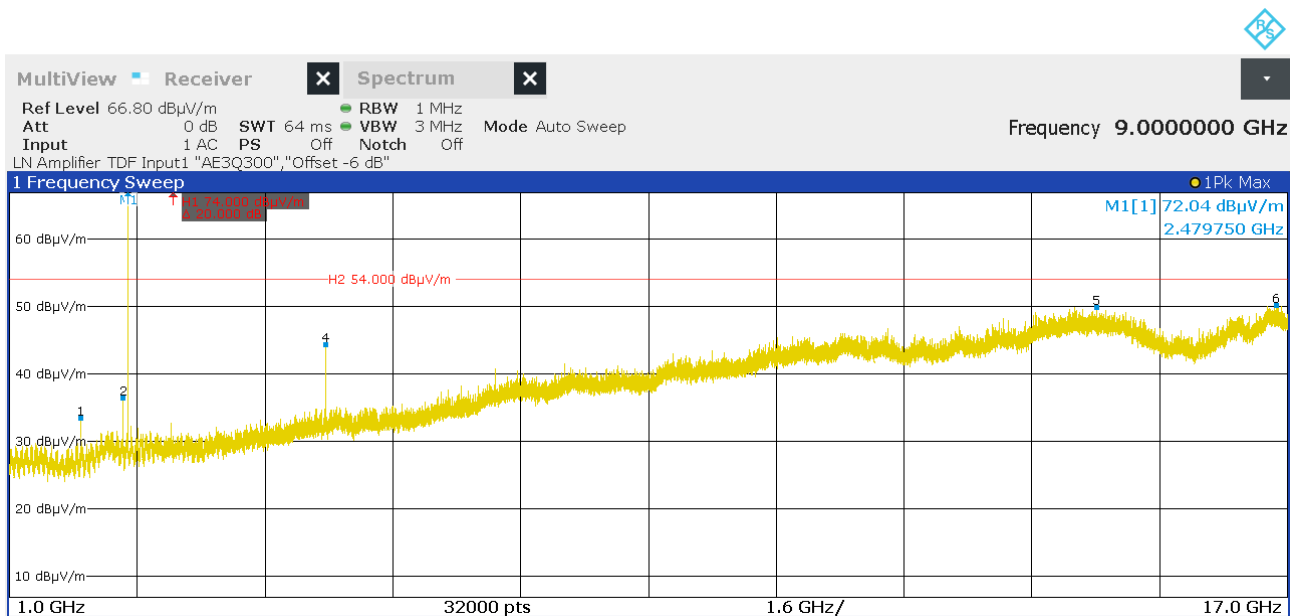
Figure 42: Chart of emissions test from 1 GHz to 17 GHz on highest channel, EUT position Y, antenna polarization horizontal
