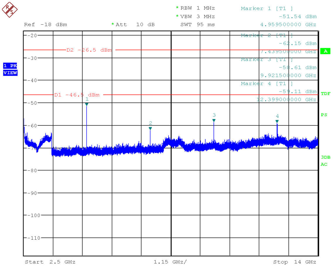
Figure 30: Chart of emissions test from 2.5 GHz to 14 GHz on highest channel, PK-detector
