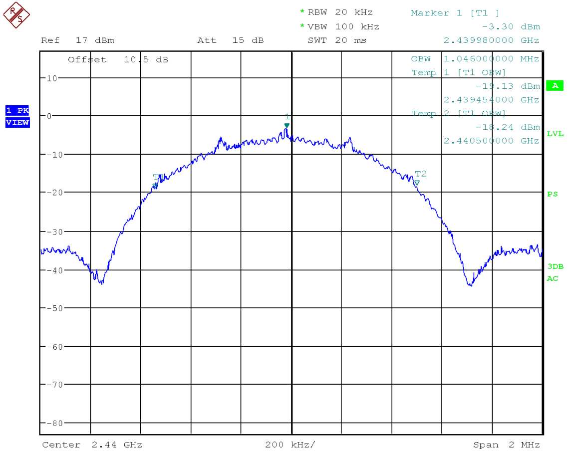
Figure 10: Chart of occupied bandwidth test on middle channel
