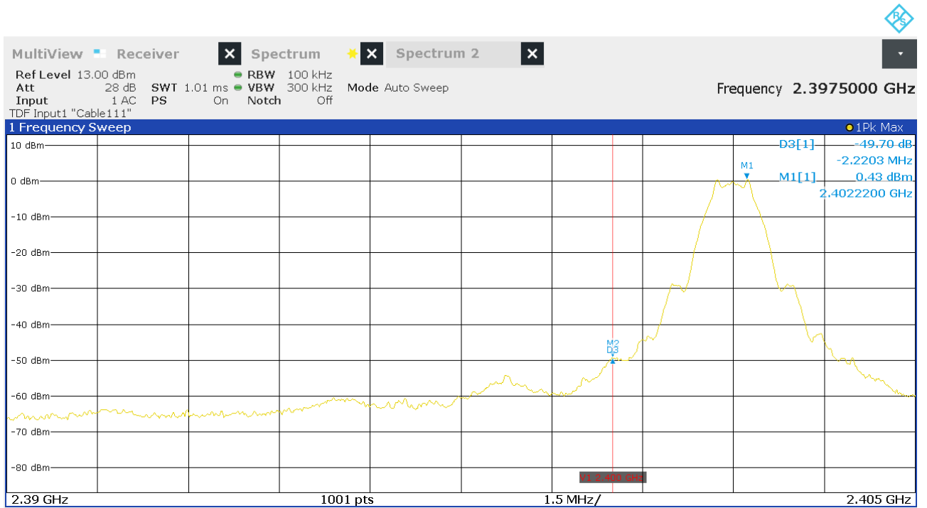
Figure 18: Chart of lower band-edge measurement on lowest channel
