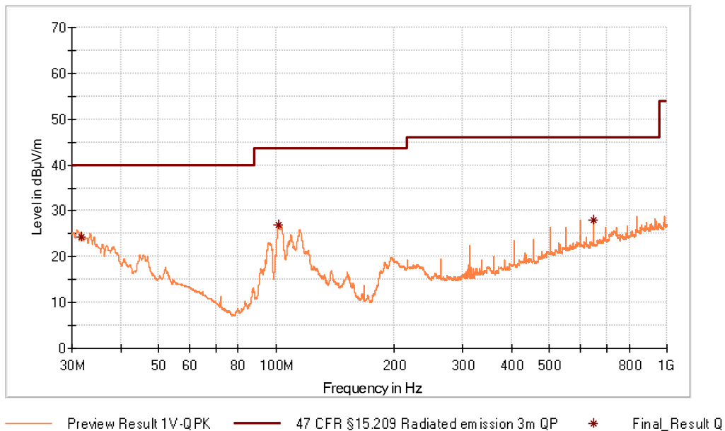
Figure 35: Chart of radiated emissions test from 30 MHz to 1 GHz on lowest channel, EUT position X, antenna polarization vertical
