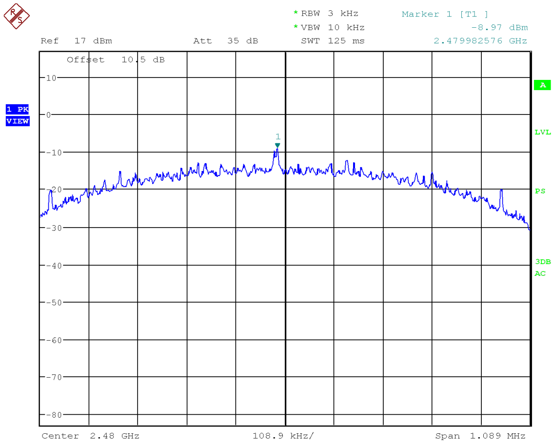
Figure 17: Chart of power spectral density on highest channel
