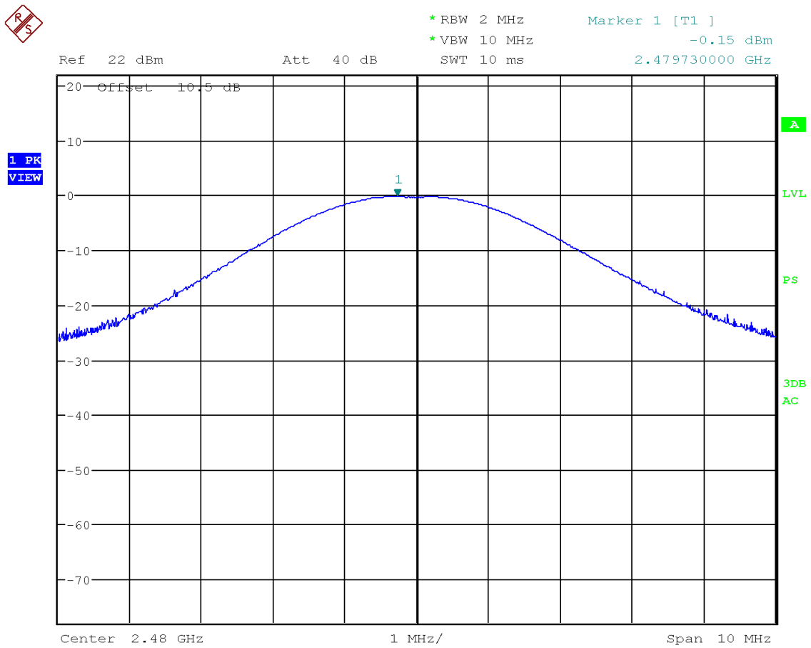
Figure 14: Chart of conducted output power on highest channel
