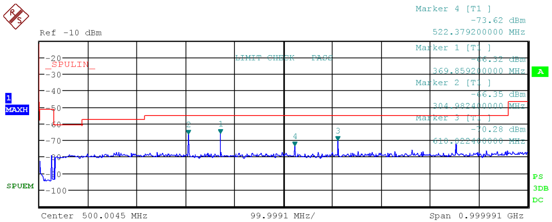
Figure 24: Chart of emissions test from 9 kHz to 1 GHz on middle channel, PK-detector
