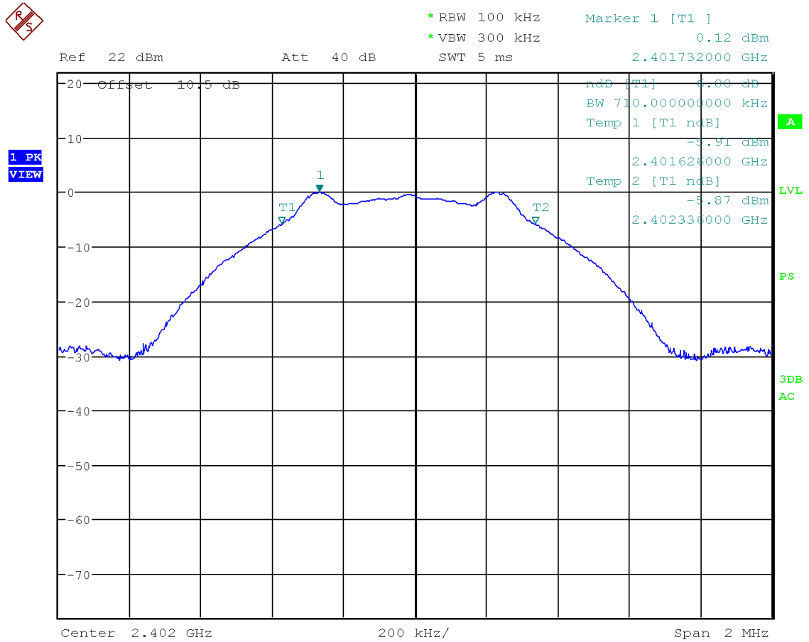
Figure 6: Chart of 6 dB bandwidth test on lowest channel
