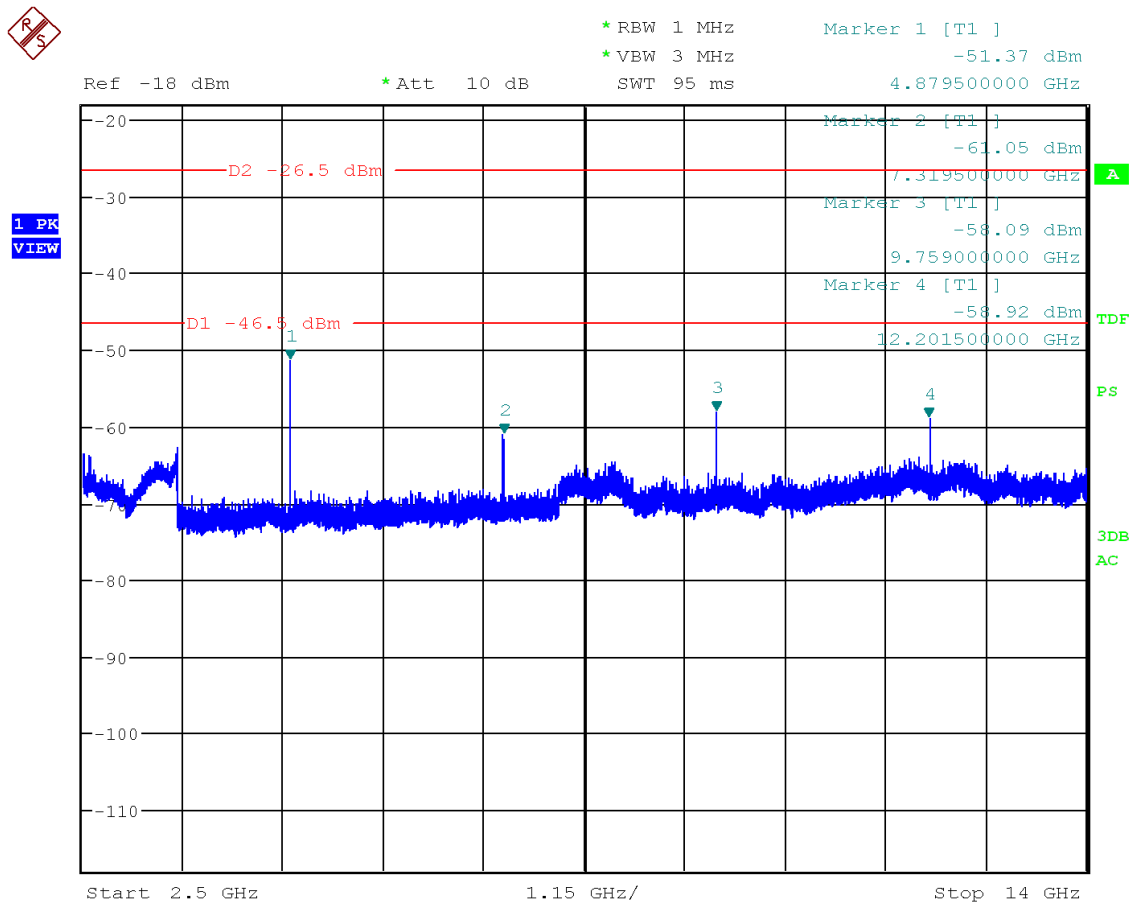
Figure 26: Chart of emissions test from 2.5 GHz to 14 GHz on middle channel, PK-detector
