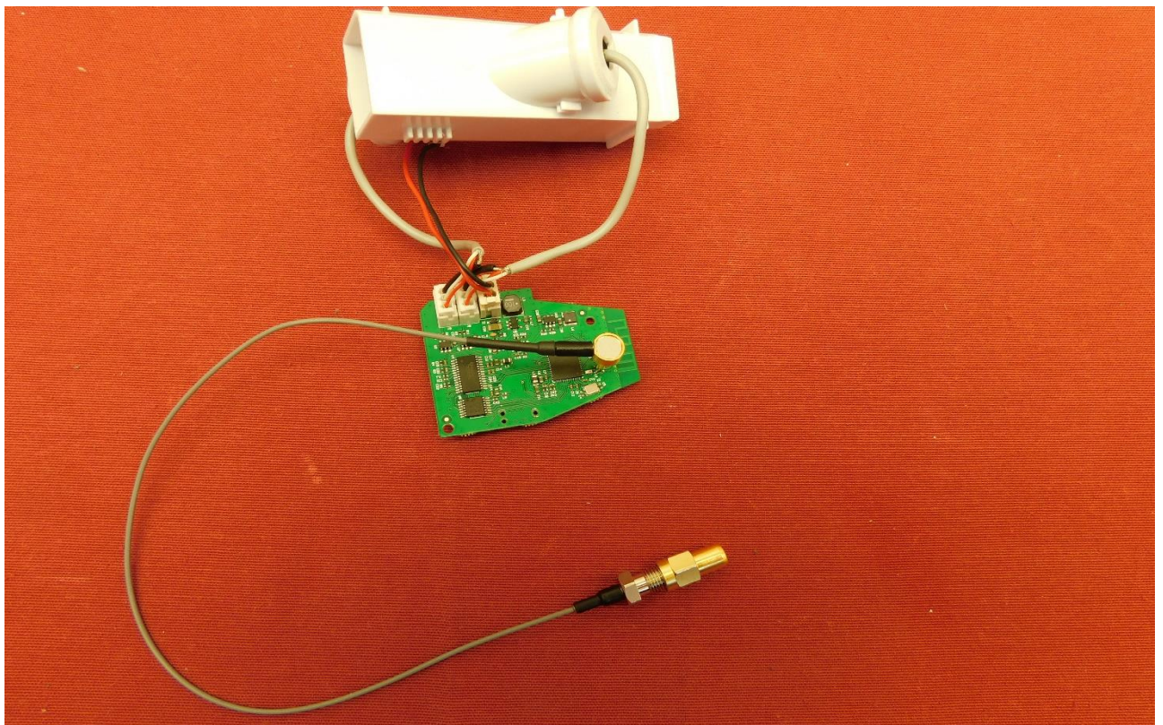
Picture 4: Front view of PCB connected with the battery socket and the sensor of the spirometer, with antenna cable connected to the switchable antenna socket
