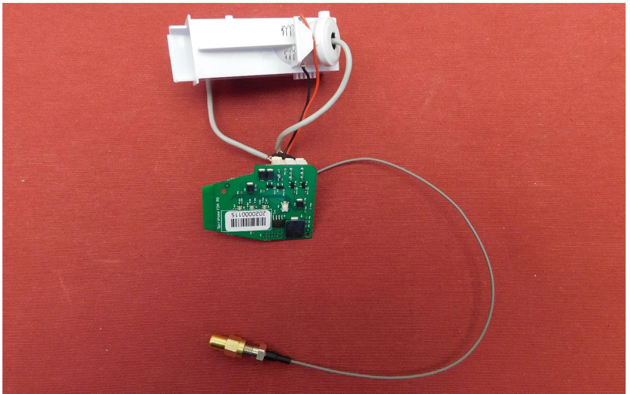
Picture 3: Rear view of PCB connected with the battery socket and the sensor of the spirometer, with antenna cable connected to the switchable antenna socket
