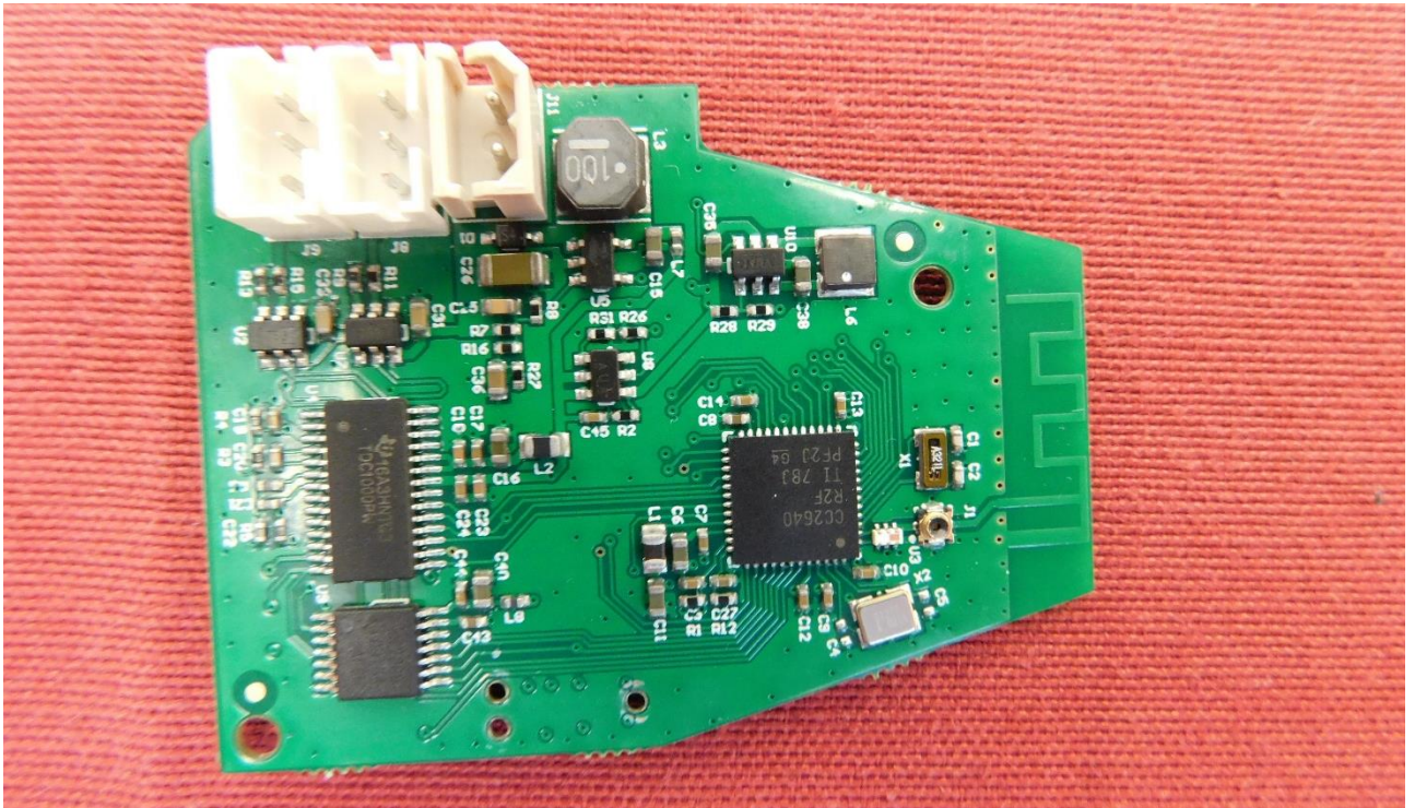
Picture 1: PCB - top side
