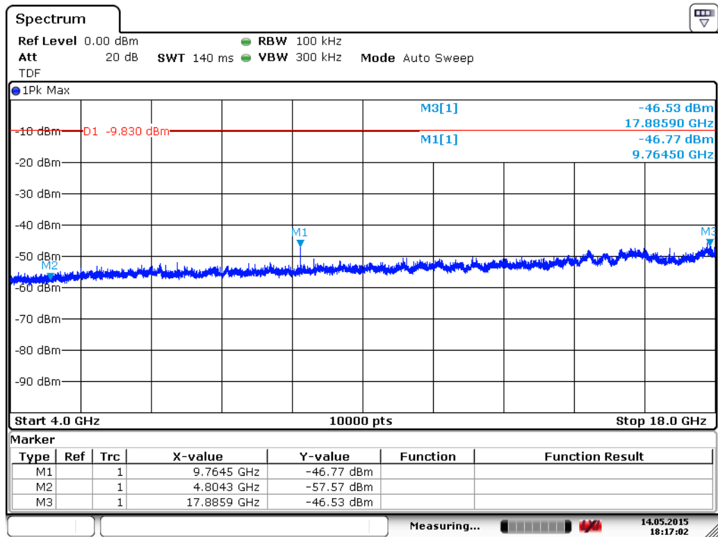
Figure 47. Low channel conducted emission 4 GHz to 18 GHz (2 Mbps).
