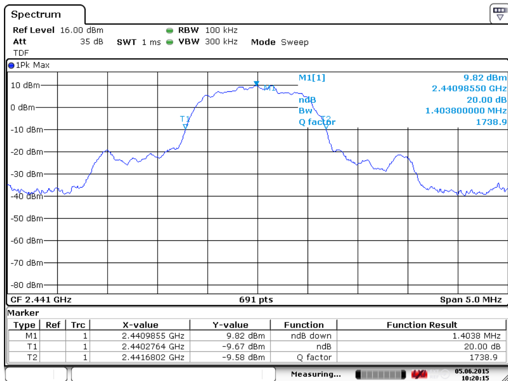
Figure 74. 20 dB channel BW. 3 Mbps Channel MID.
