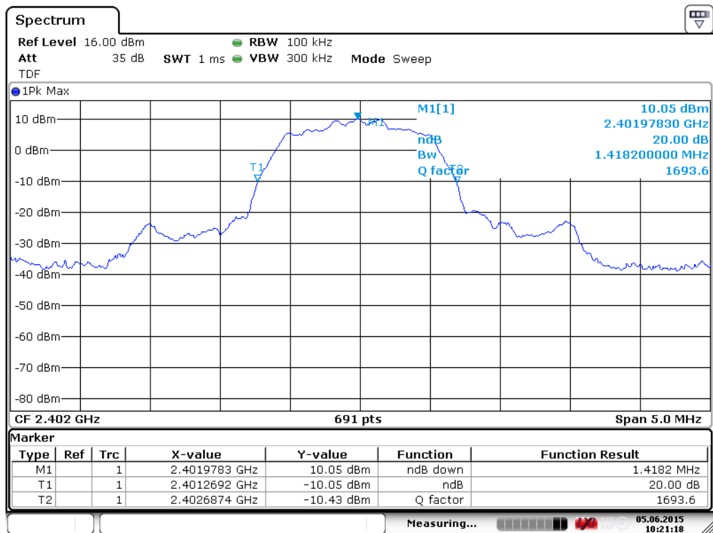
Figure 70. 20 dB channel BW. 2 Mbps Channel LOW.
