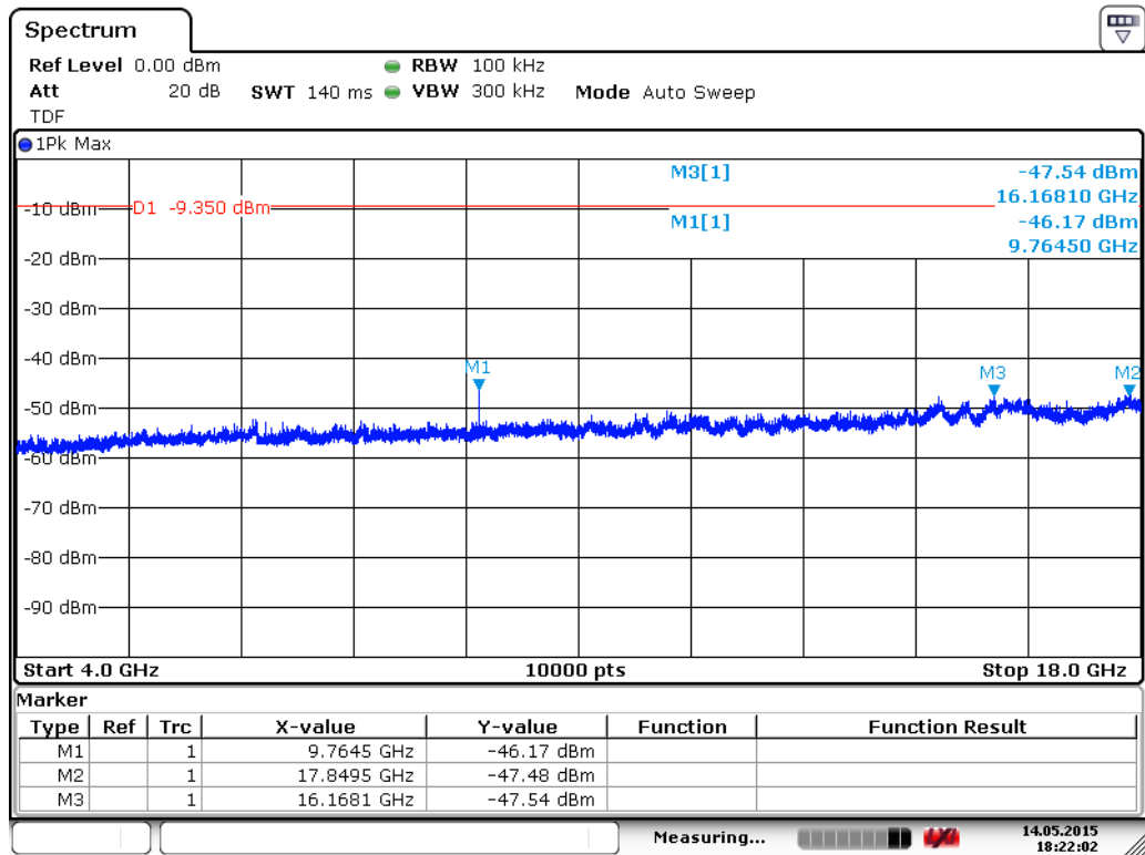
Figure 61. Low channel conducted emission 4 GHz to 18 GHz (3 Mbps).
