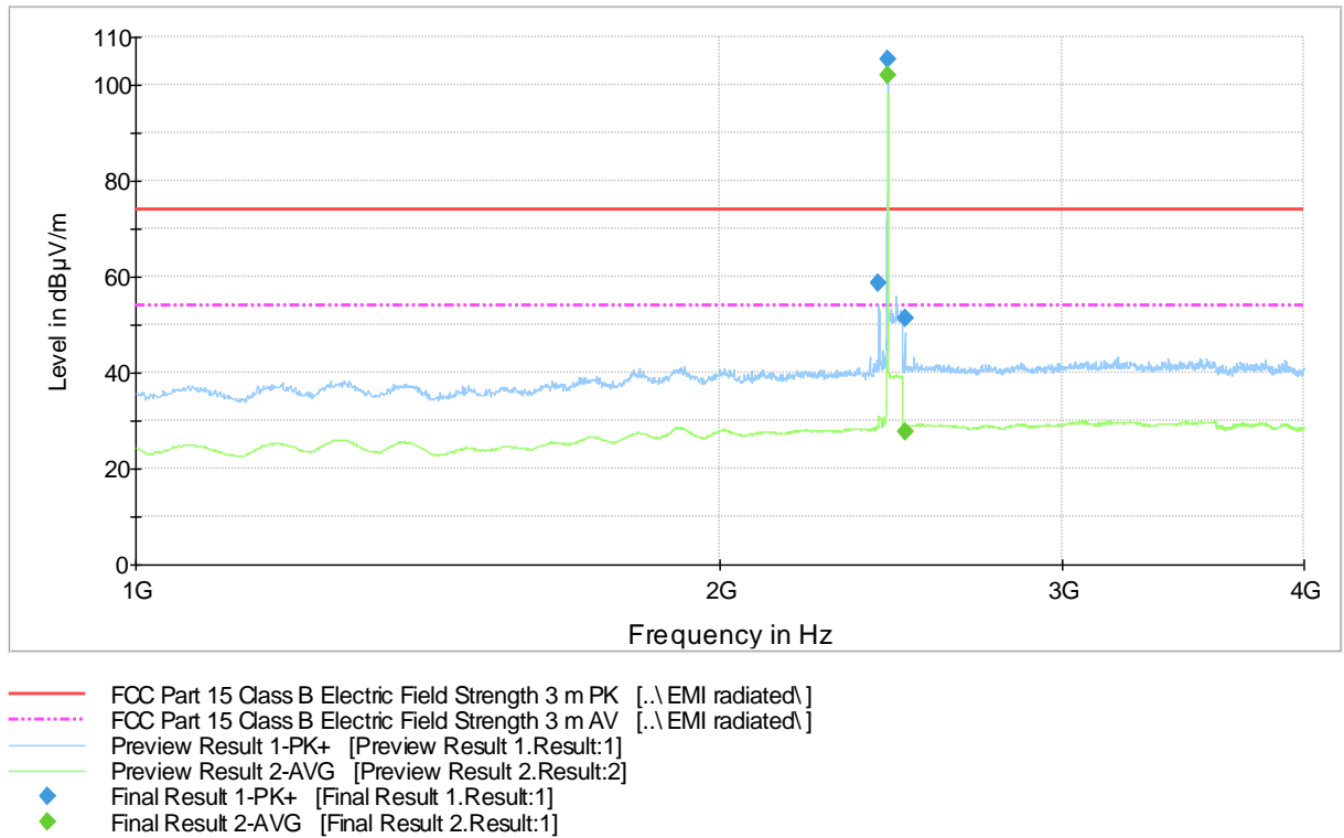
Figure 16. Measured curve with peak- and average detector. 1 Mbps Channel MID.
