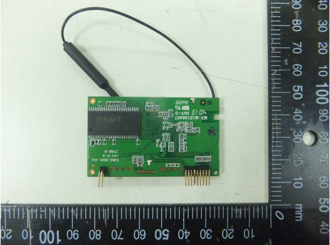
10 Antenna-R
