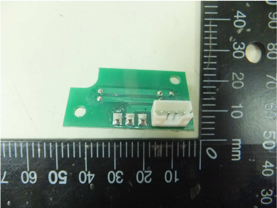
08 PCB2-R
