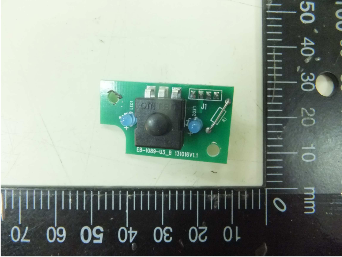
07 PCB2-F
