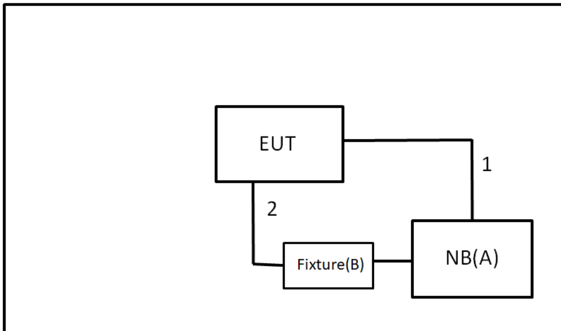
Radiated Emissions
