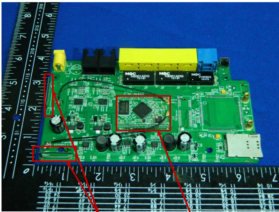
WIFI antenna
