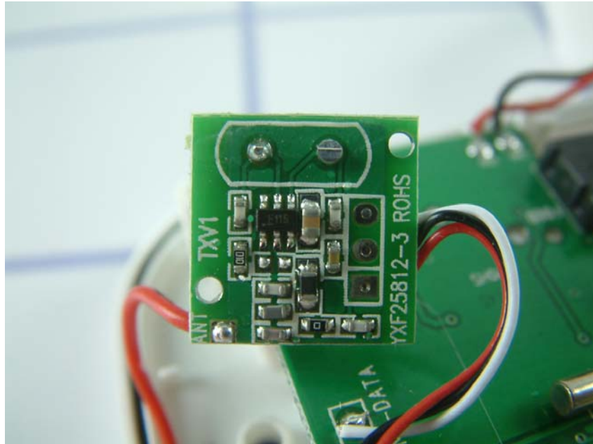
Oscillator 2 view
