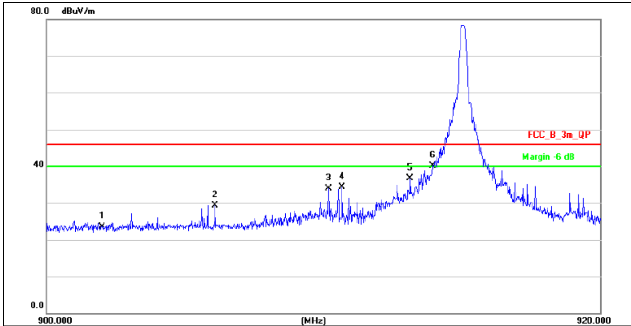
915 MHz Horizontal
