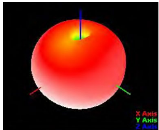
Typical Free Space 3D Radiation Pattern at 27MHz,0dBi
