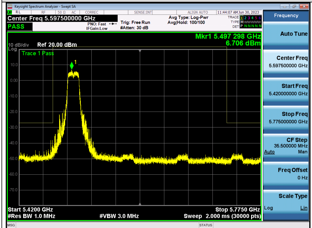
Test_Graph_802.11a_ANT2_5500_6Mbps_Frequency Band 3
