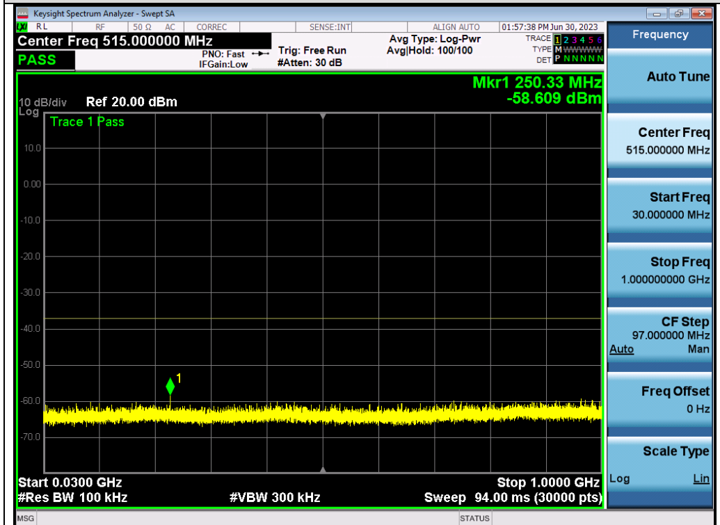
Test_Graph_802.11ax80_ANT2_5610_MCS9_Frequency Band 1
