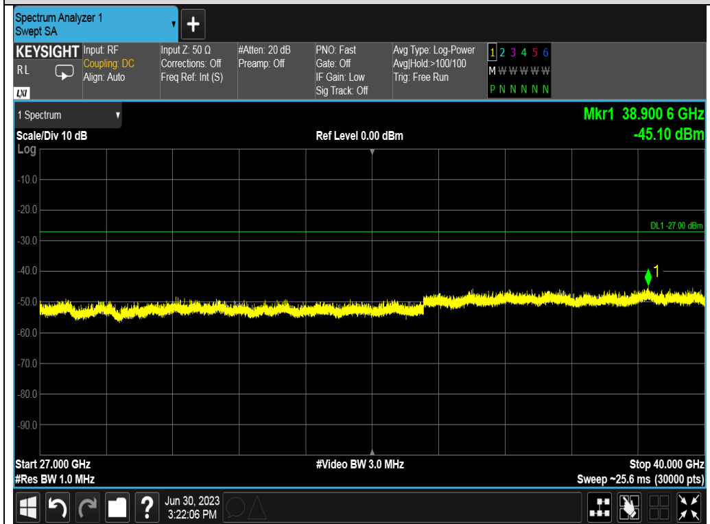
Test_Graph_802.11ax80_ANT2_5610_MCS9_Frequency Band 5
