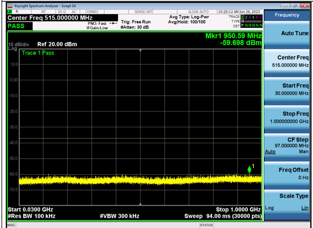
Test_Graph_802.11ax80_ANT1_5530_MCS9_Frequency Band 1
