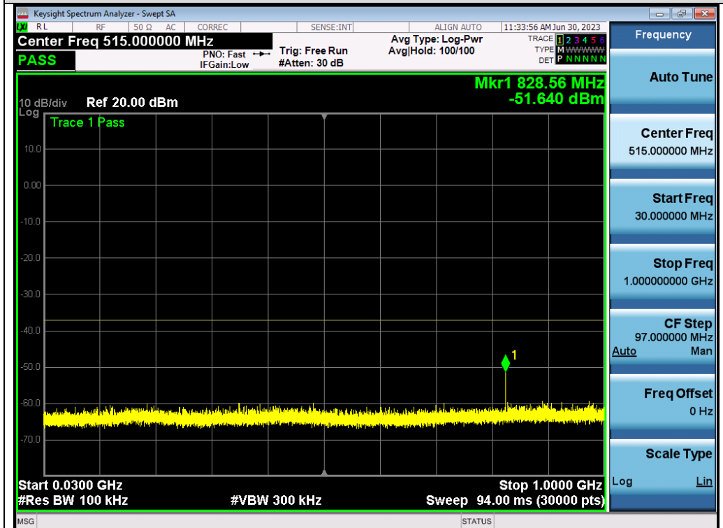
Test_Graph_802.11ax80_ANT2_5290_MCS0_Frequency Band 1
