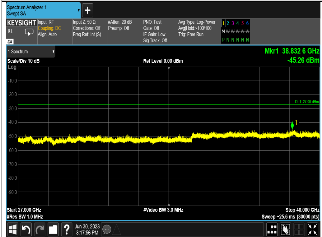
Test_Graph_802.11n40_ANT2_5510_MCS0_Frequency Band 5
