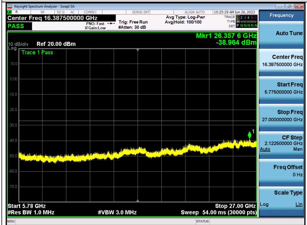
Test_Graph_802.11ax80_ANT1_5610_MCS9_Frequency Band 4
