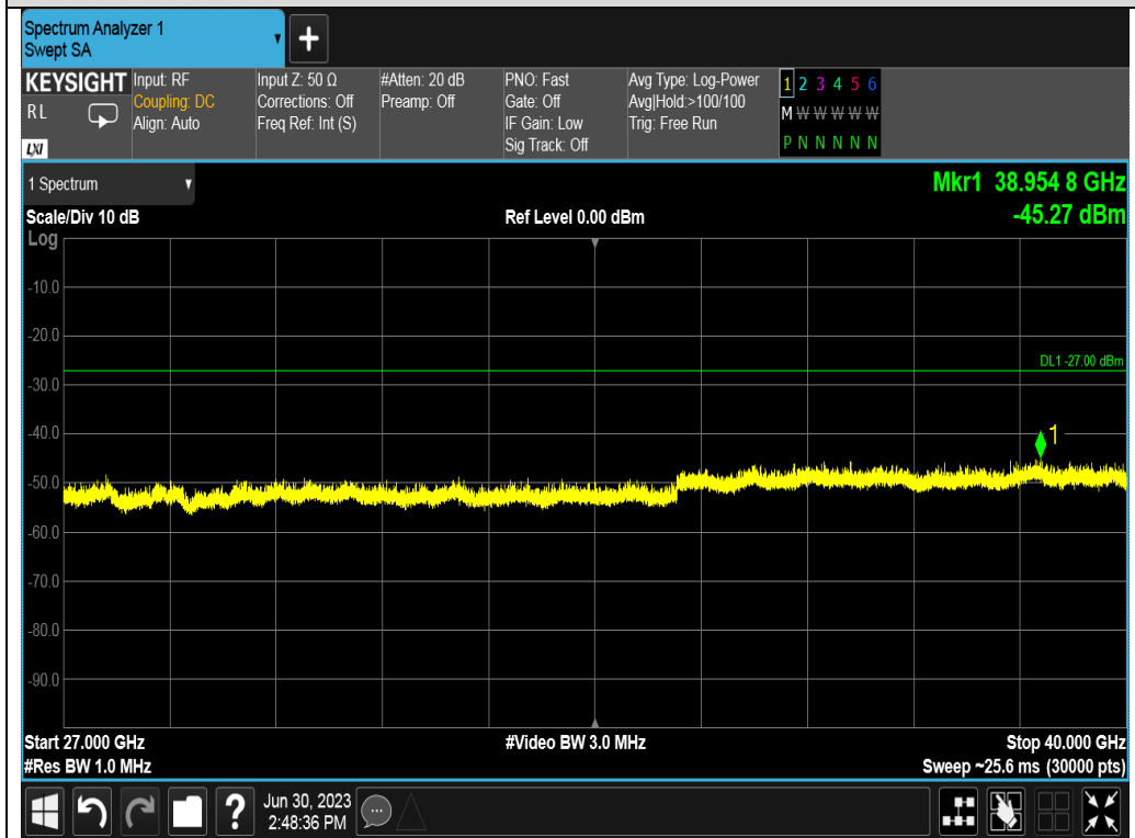
Test_Graph_802.11n40_ANT2_5230_MCS0_Frequency Band 5
