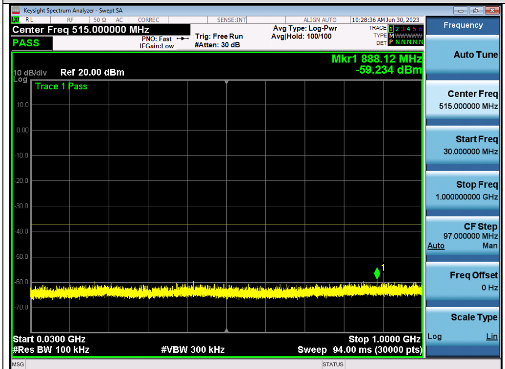
Test_Graph_802.11ax80_ANT2_5210_MCS9_Frequency Band 1
