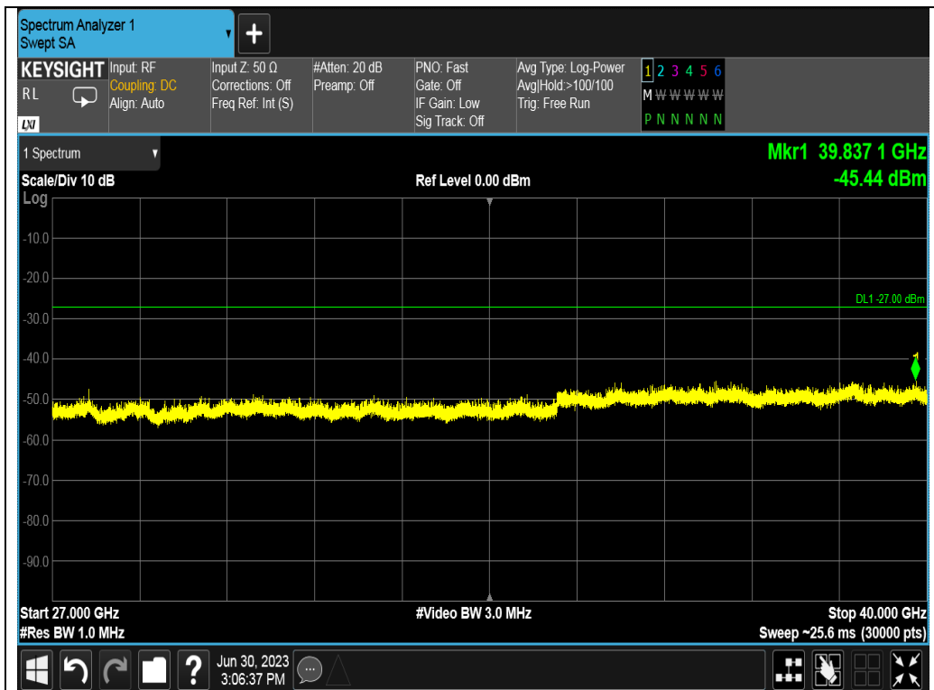
Test_Graph_802.11n40_ANT2_5270_MCS0_Frequency Band 5
