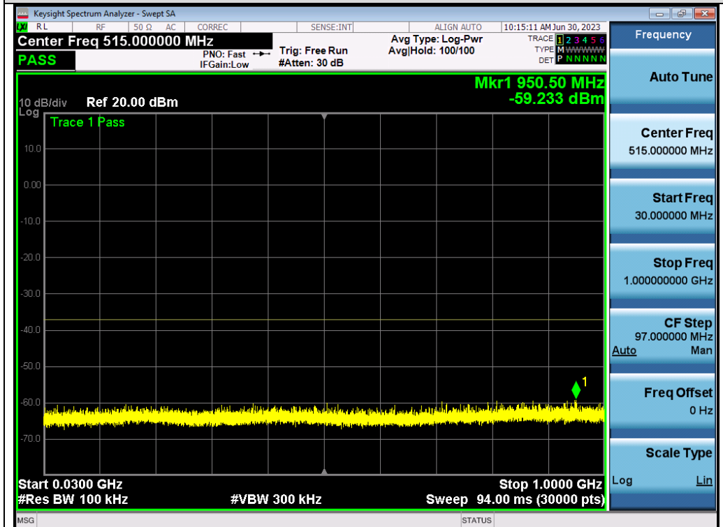
Test_Graph_802.11n40_ANT2_5230_MCS0_Frequency Band 1
