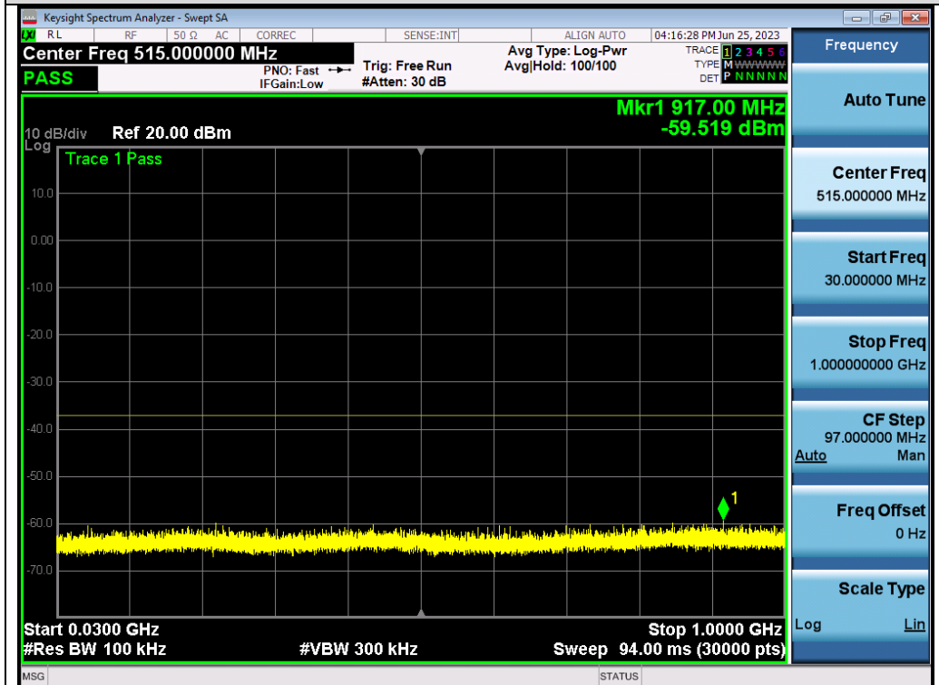
Test_Graph_802.11ax80_ANT1_5210_MCS0_Frequency Band 1
