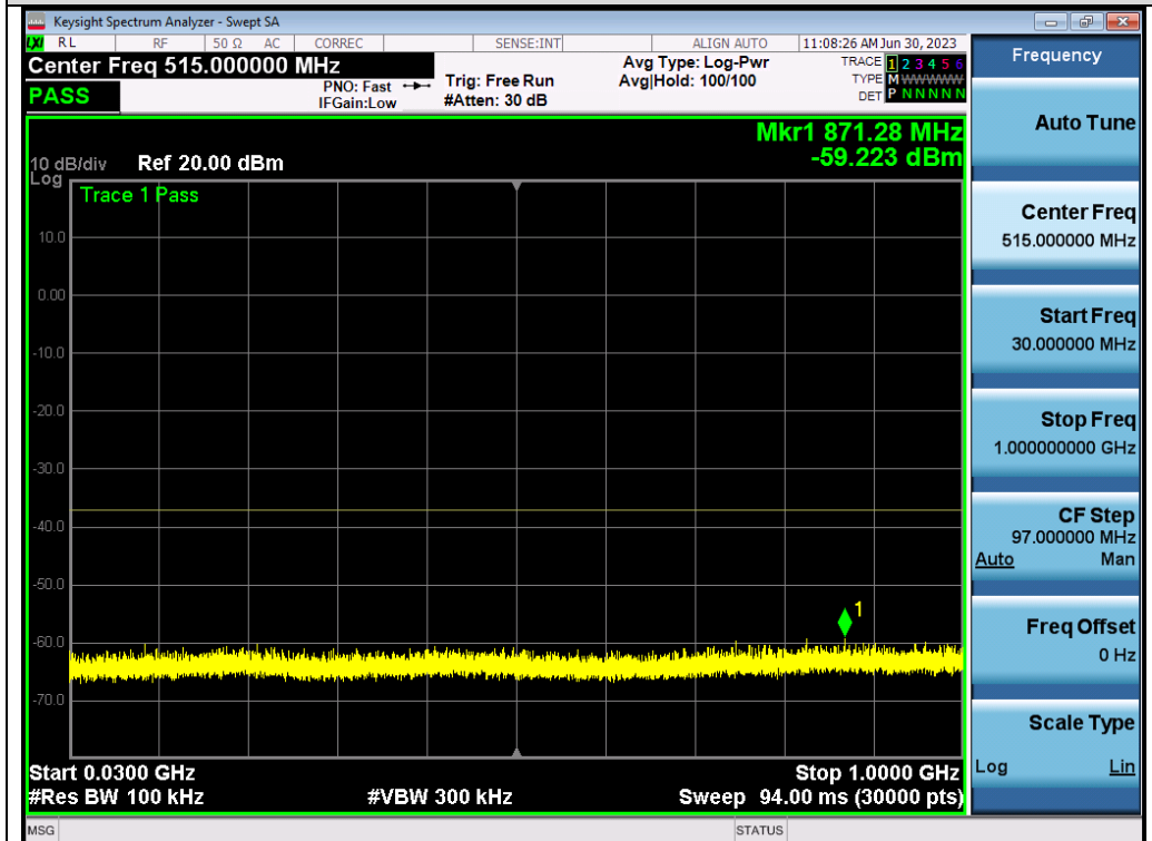
Test_Graph_802.11n40_ANT2_5310_MCS0_Frequency Band 1
