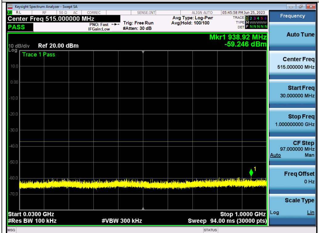
Test_Graph_802.11ax80_ANT1_5290_MCS0_Frequency Band 1
