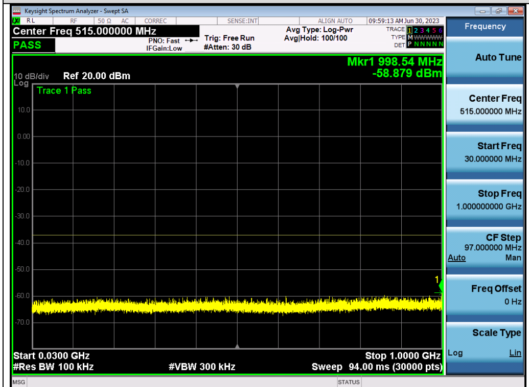
Test_Graph_802.11a_ANT2_5240_6Mbps_Frequency Band 1
