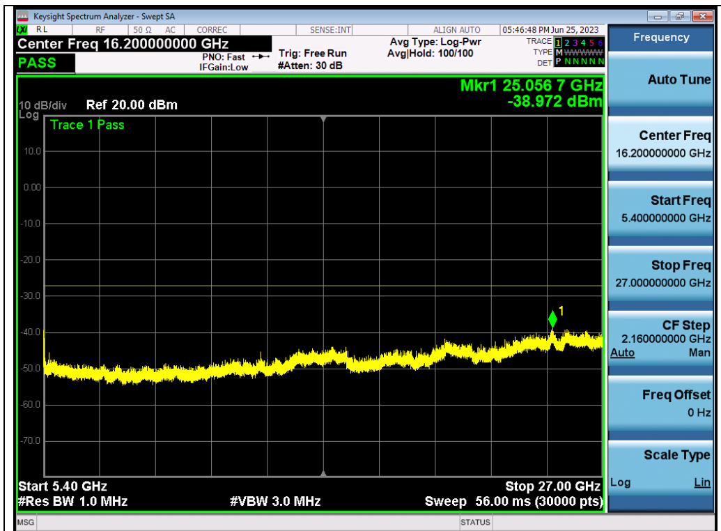
Test_Graph_802.11ax80_ANT1_5290_MCS0_Frequency Band 4
