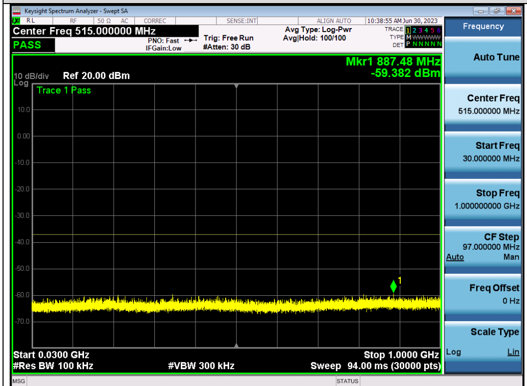
Test_Graph_802.11a_ANT2_5320_6Mbps_Frequency Band 1
