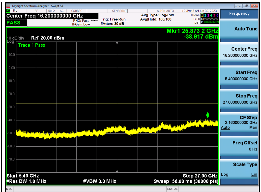
Test_Graph_802.11a_ANT2_5320_6Mbps_Frequency Band 4
