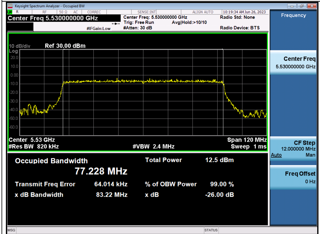
Test_Graph_802.11ax80_ANT1_5530_MCS9_OBW
