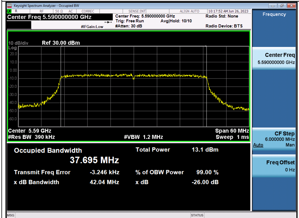
Test_Graph_802.11ax40_ANT1_5590_MCS9_OBW
