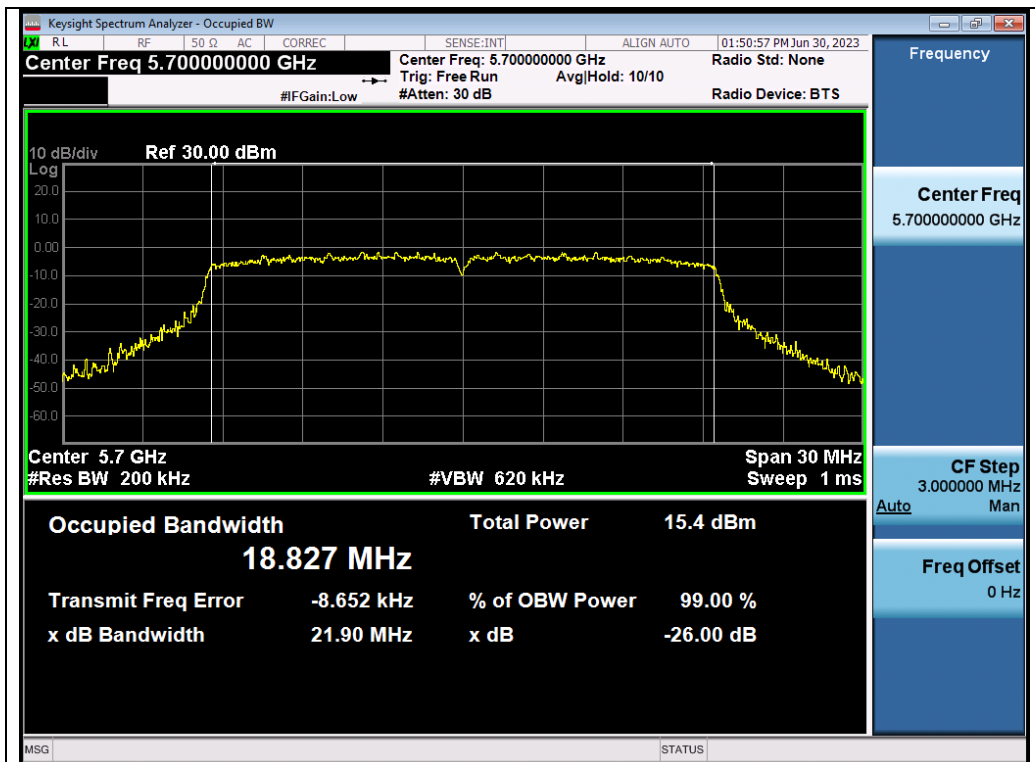
Test_Graph_802.11ax20_ANT2_5700_MCS9_OBW
