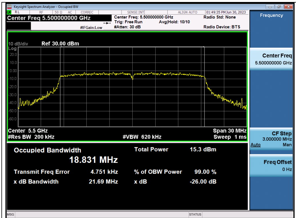
Test_Graph_802.11ax20_ANT2_5500_MCS0_OBW
