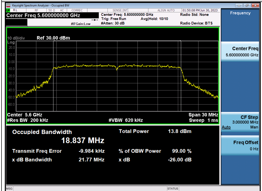
Test_Graph_802.11ax20_ANT2_5600_MCS0_OBW
