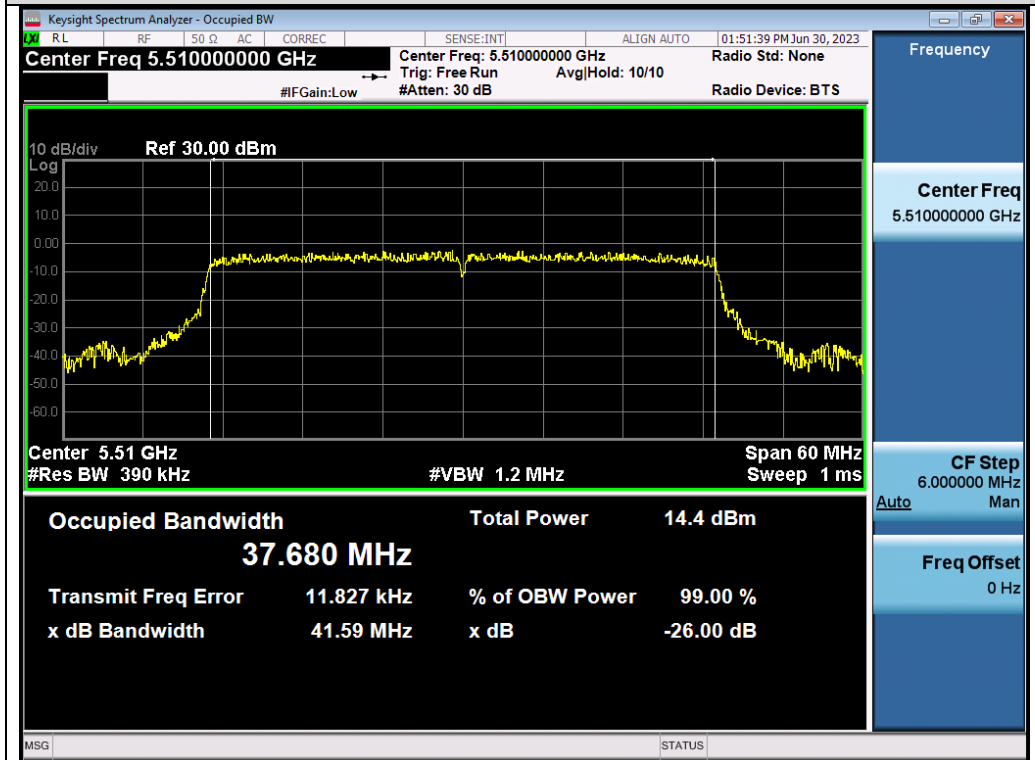
Test_Graph_802.11ax40_ANT2_5510_MCS9_OBW
