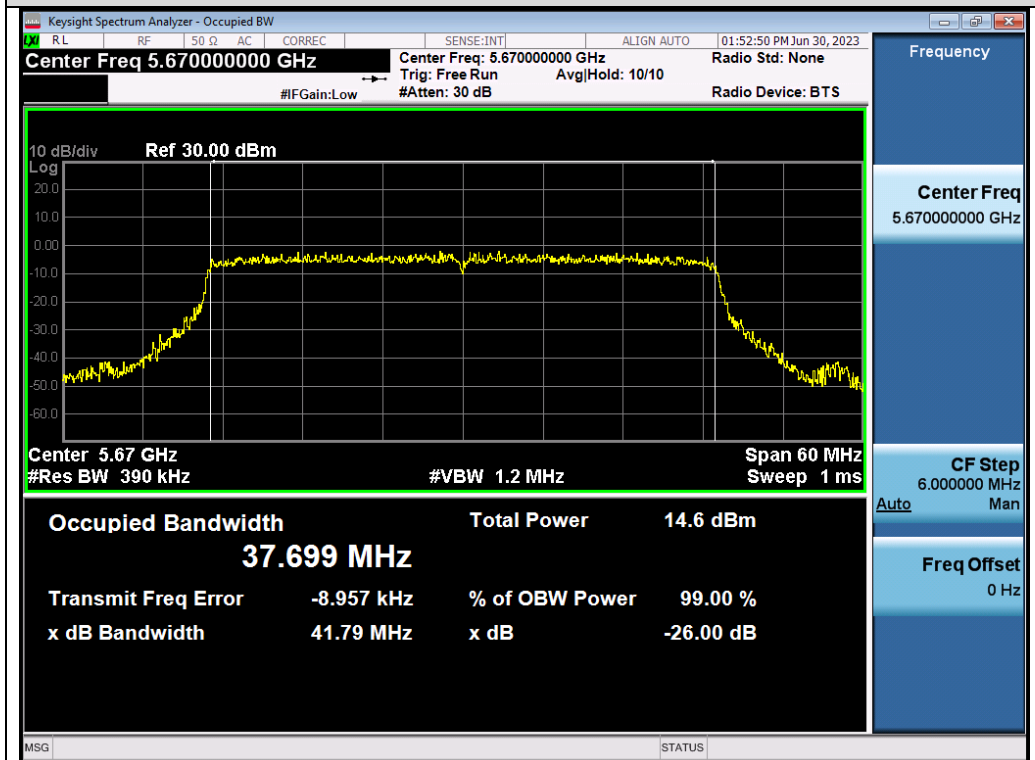
Test_Graph_802.11ax40_ANT2_5670_MCS9_OBW
