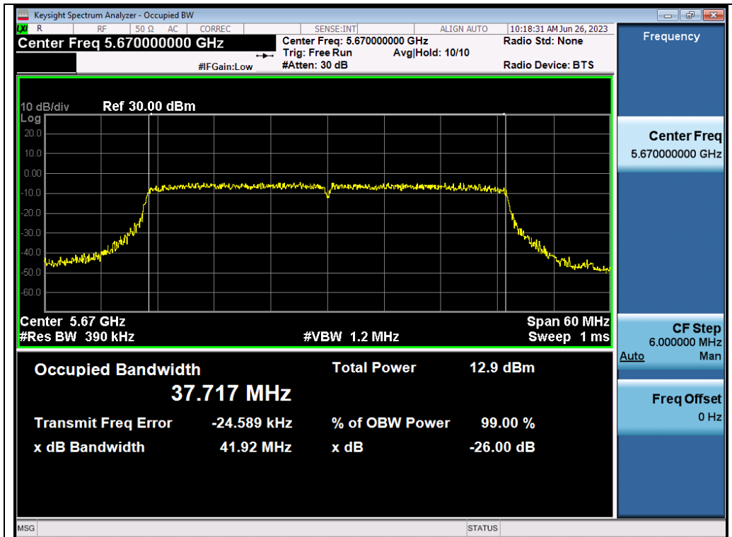
Test_Graph_802.11ax40_ANT1_5670_MCS9_OBW
