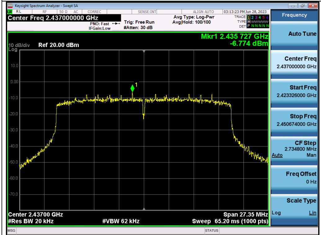
Test_Graph_802.11ax20_ANT2_2437_MCS0_PSD
