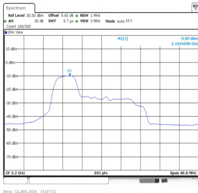
11AX20MIMO-Ant2-5200-52Tone-RU37-PASS
