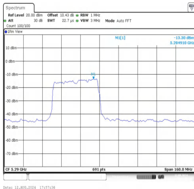
11AX80MIMO-Ant2-5290-484Tone-RU65-PASS
