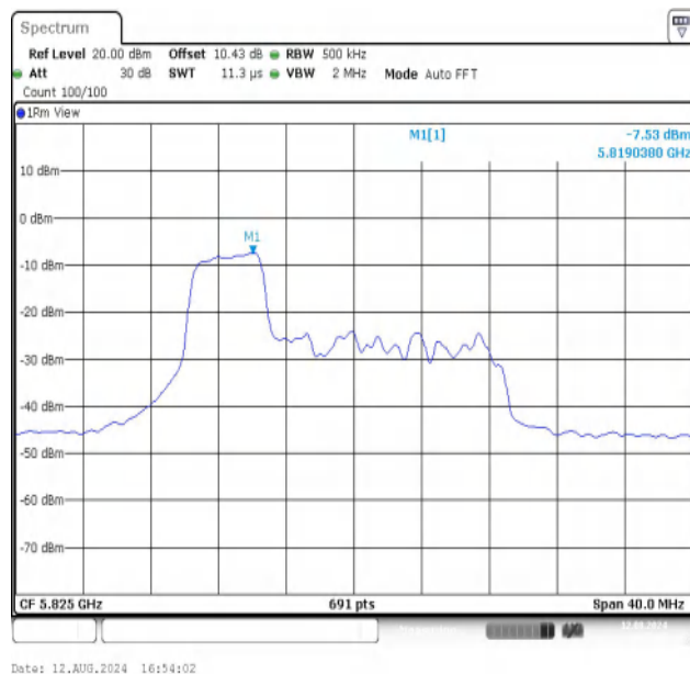
11AX20MIMO-Ant2-5825-52Tone-RU37-PASS
