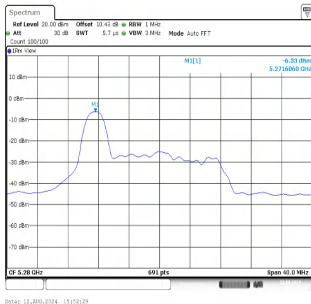
11AX20MIMO-Ant2-5280-26Tone-RU0-PASS
