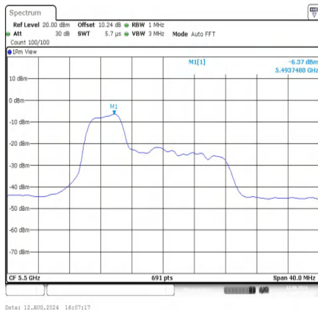
11AX20MIMO-Ant2-5500-52Tone-RU37-PASS
