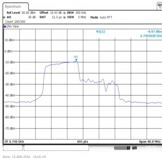
11AX20MIMO-Ant2-5745-106Tone-RU53-PASS
