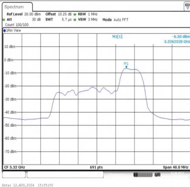
11AX20MIMO-Ant1-5320-52Tone-RU40-PASS
