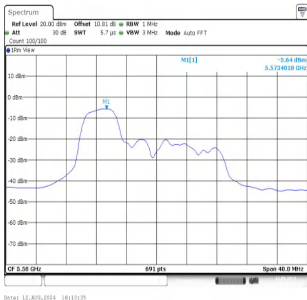
11AX20MIMO-Ant1-5580-52Tone-RU37-PASS
