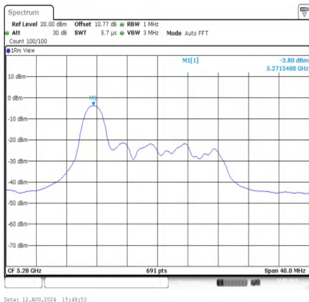
11AX20MIMO-Ant1-5280-26Tone-RU0-PASS
