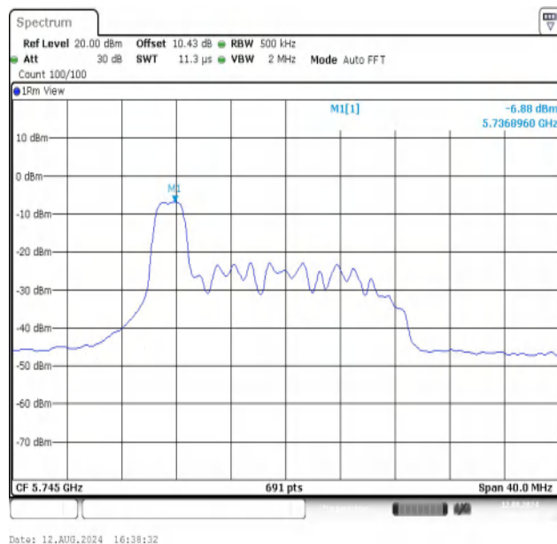
11AX20MIMO-Ant2-5745-26Tone-RU0-PASS
