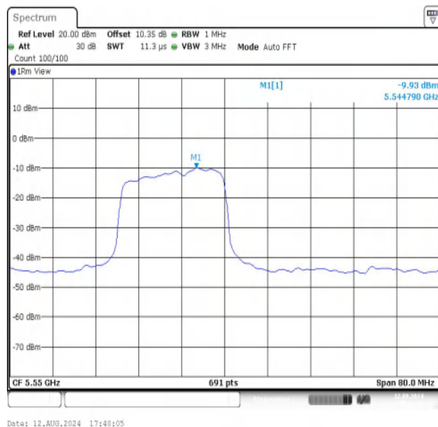
11AX40MIMO-Ant2-5550-242Tone-RU61-PASS
