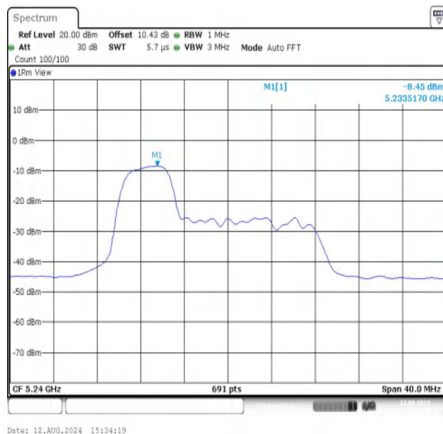
11AX20MIMO-Ant2-5240-52Tone-RU37-PASS
