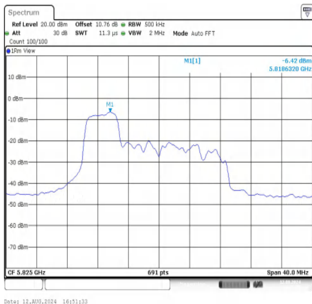
11AX20MIMO-Ant1-5825-52Tone-RU37-PASS
