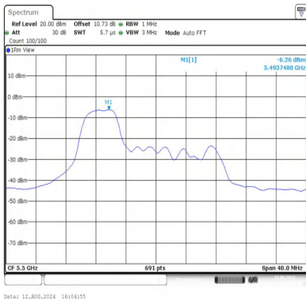
11AX20MIMO-Ant1-5500-52Tone-RU37-PASS
