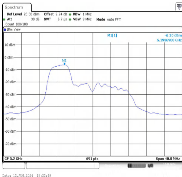
11AX20MIMO-Ant1-5200-52Tone-RU37-PASS
