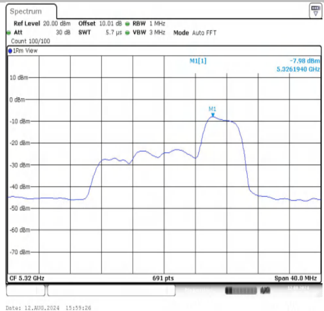
11AX20MIMO-Ant2-5320-52Tone-RU40-PASS
