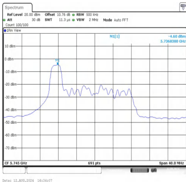
11AX20MIMO-Ant1-5745-26Tone-RU0-PASS
