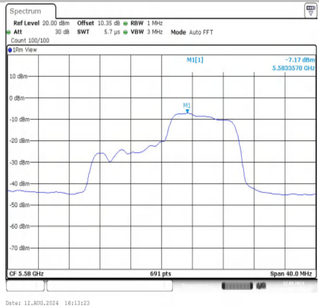
11AX20MIMO-Ant2-5580-106Tone-RU54-PASS
