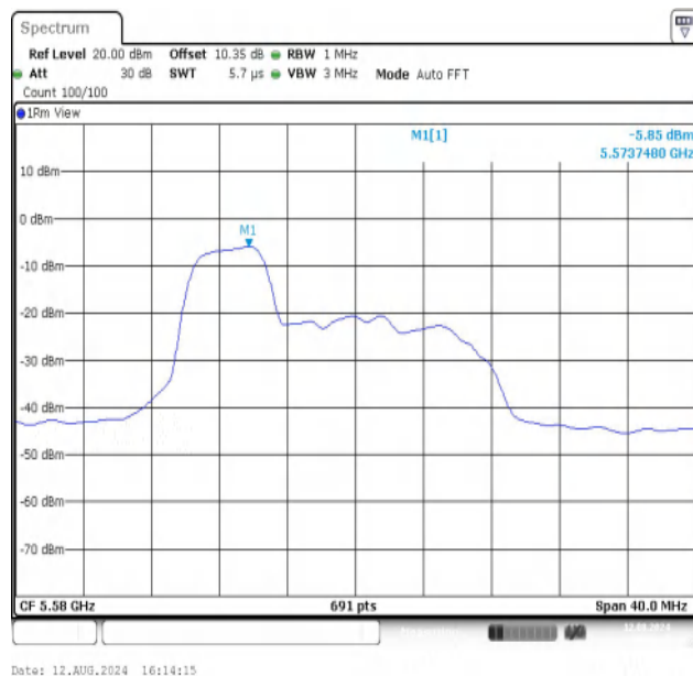
11AX20MIMO-Ant2-5580-52Tone-RU37-PASS
