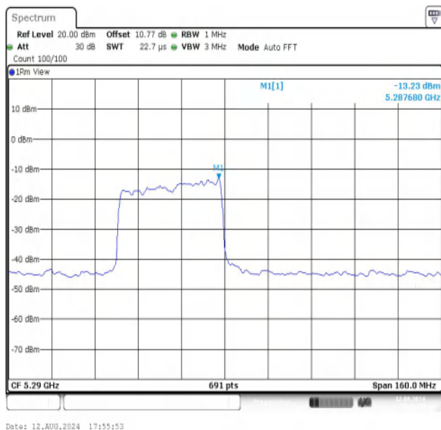
11AX80MIMO-Ant1-5290-484Tone-RU65-PASS
