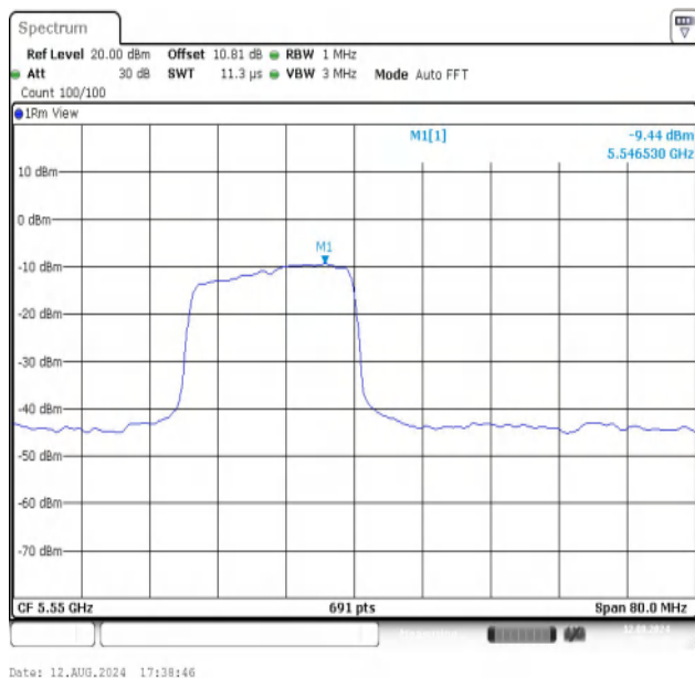
11AX40MIMO-Ant1-5550-242Tone-RU61-PASS
