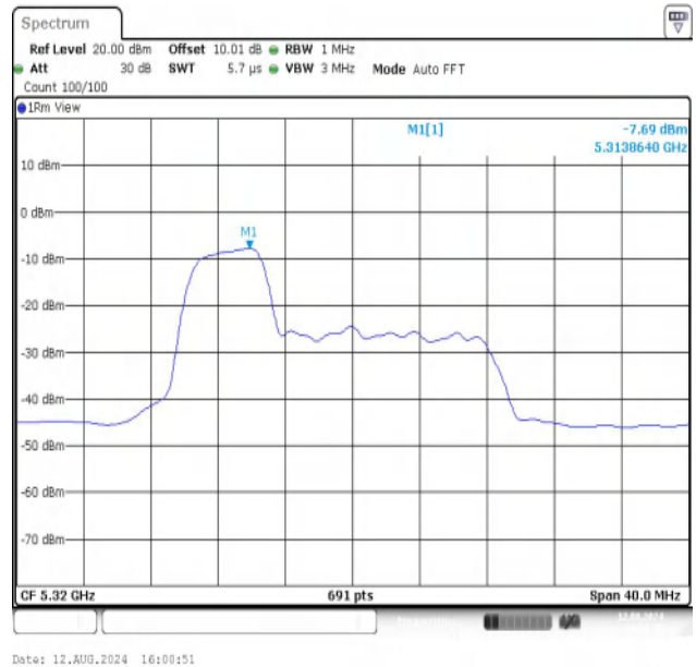
11AX20MIMO-Ant2-5320-52Tone-RU37-PASS
