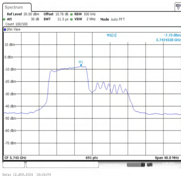
11AX20MIMO-Ant1-5745-106Tone-RU53-PASS
