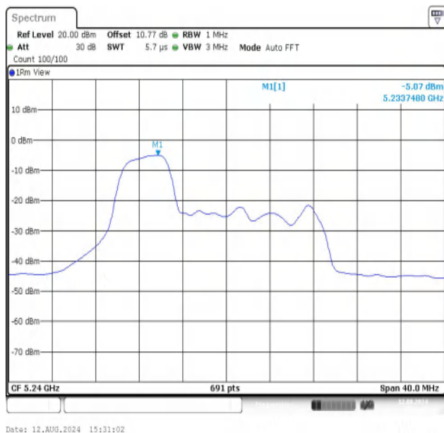
11AX20MIMO-Ant1-5240-52Tone-RU37-PASS
