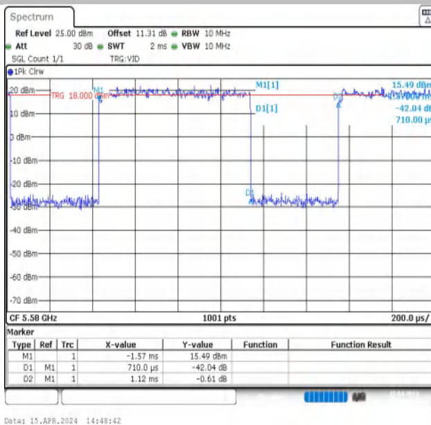
NTNV-11A-Ant1-5580
