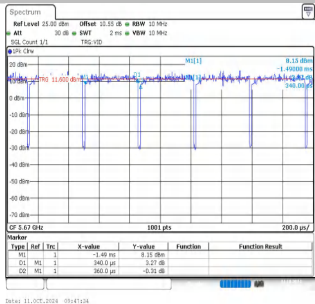
NTNV-11AC40MIMO-Ant2-5670
