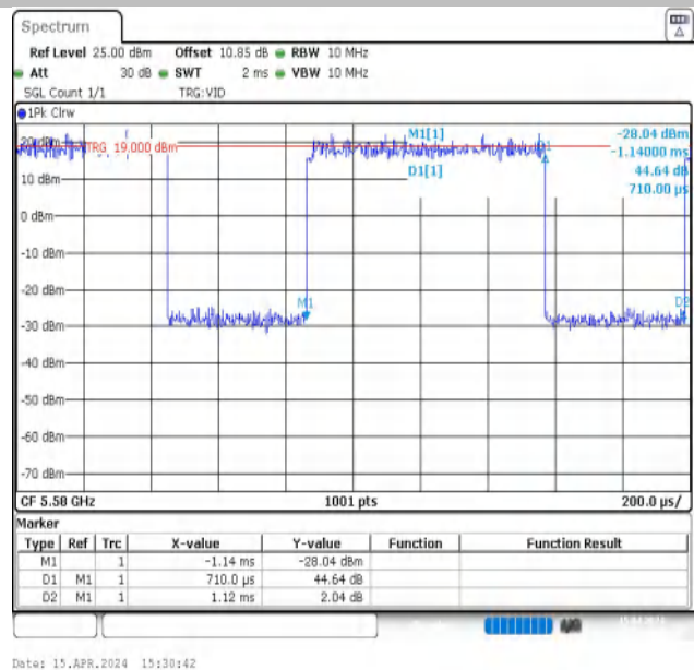
NTNV-11A-Ant2-5580
