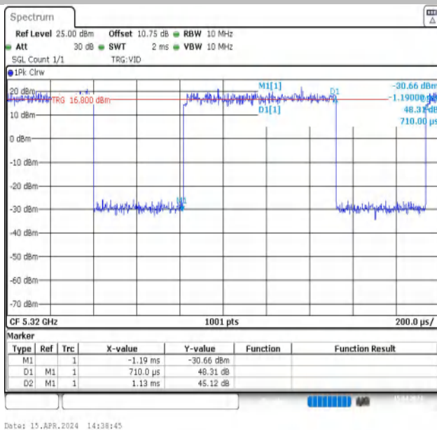
NTNV-11A-Ant1-5320
