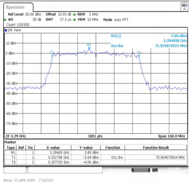
11AC80MIMO-Ant2-5290
