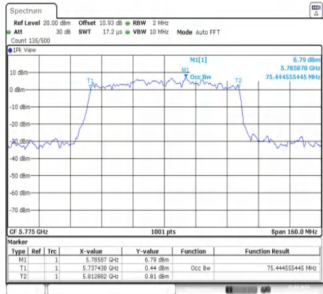
11AC80MIMO-Ant2-5775
