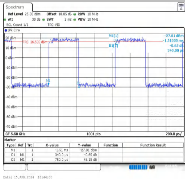
NTNV-11N20MIMO-Ant2-5580
