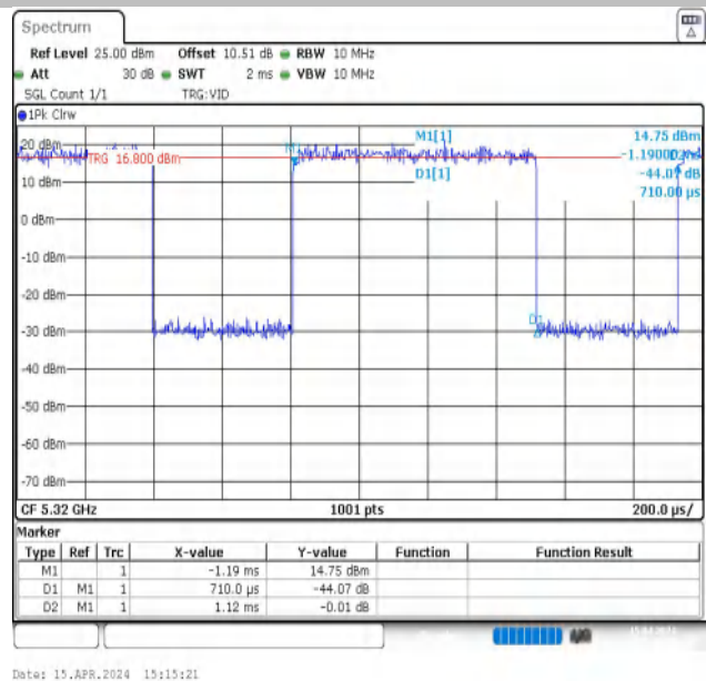
NTNV-11A-Ant2-5320
