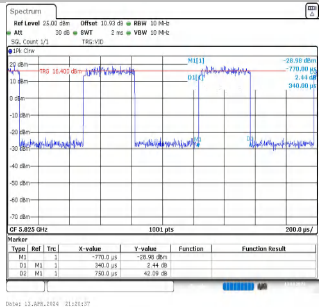
NTNV-11N20MIMO-Ant2-5825
