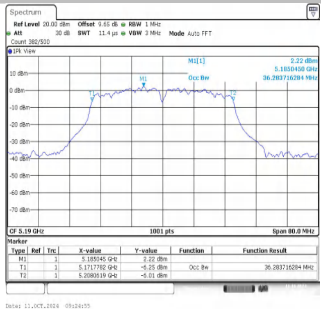
11AC40MIMO-Ant2-5190
