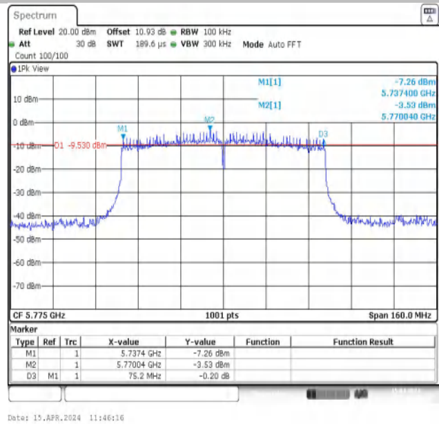
11AC80MIMO-Ant2-5775-PASS
