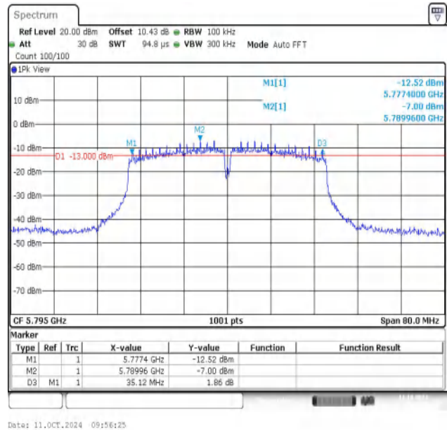
11AC40MIMO-Ant2-5795-PASS
