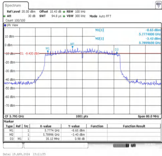
11AX40MIMO-Ant2-5795-PASS
