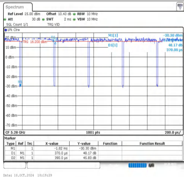
NTVN-11AC20MIMO-Ant2-5280
