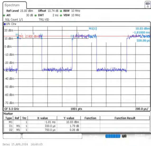
NTNV-11N20MIMO-Ant2-5500
