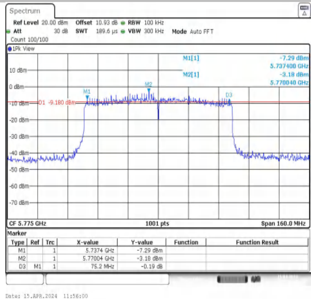
11AX80MIMO-Ant2-5775-PASS
