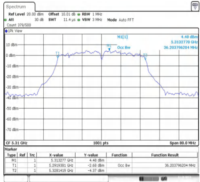
11AC40MIMO-Ant2-5310
