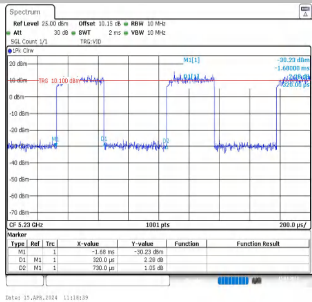
NTNV-11N40MIMO-Ant2-5230
