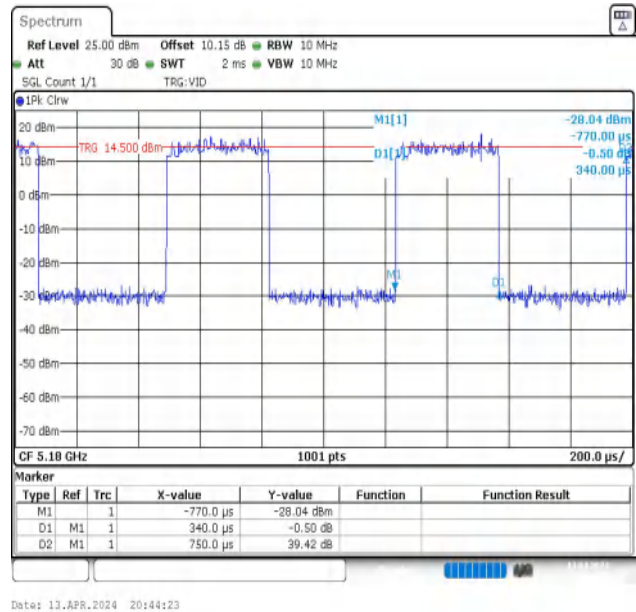
NTNV-11N20MIMO-Ant2-5180
