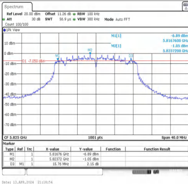
11N20MIMO-Ant1-5825-PASS
