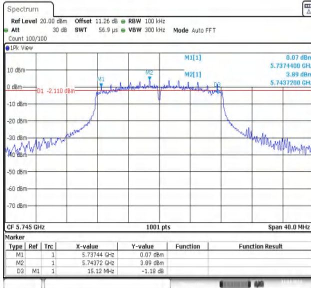
11A-Ant1-5745-PASS
