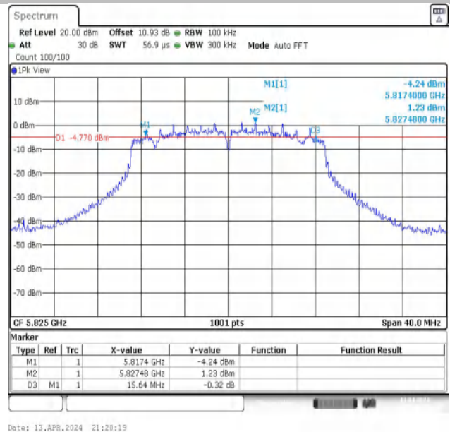
11N20MIMO-Ant2-5825-PASS
