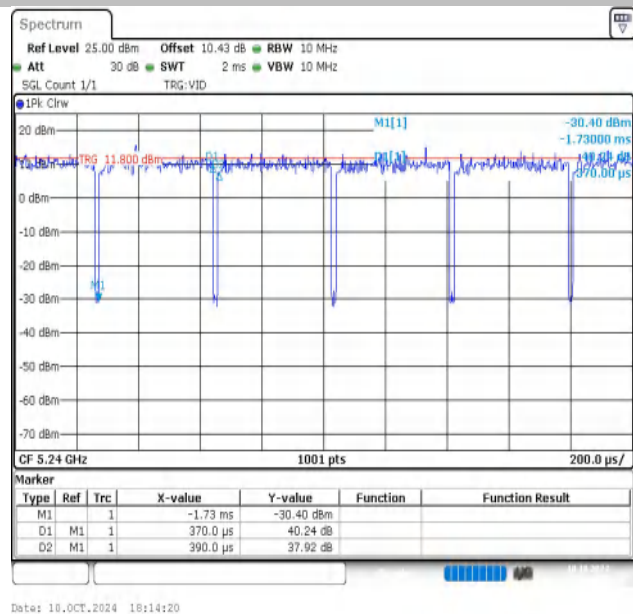
NTNV-11AC20MIMO-Ant2-5240
