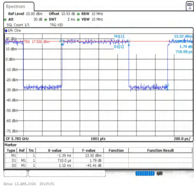
NTNV-11A-Ant2-5785
