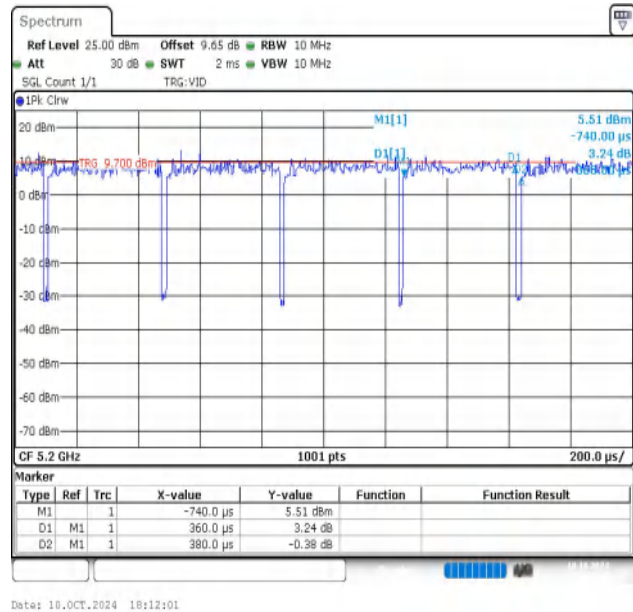
NTNV-11AC20MIMO-Ant2-5200
