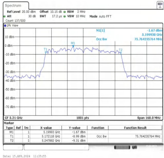
11AC80MIMO-Ant2-5210
