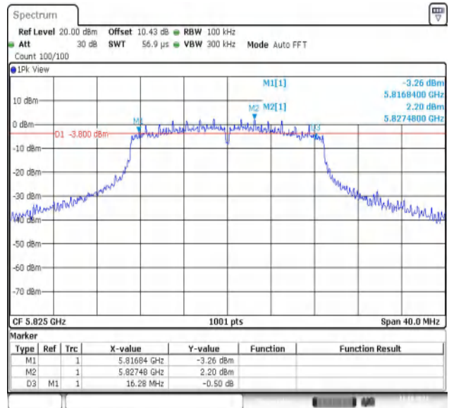
11AC20MIMO-Ant2-5825-PASS
