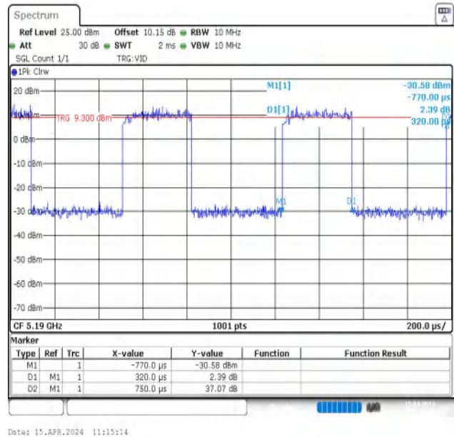
NTNV-11N40MIMO-Ant2-5190
