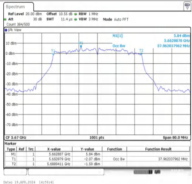
11AX40MIMO-Ant2-5670
