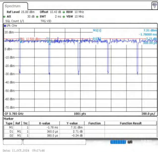
NTNV-11AC20MIMO-Ant2-5785
