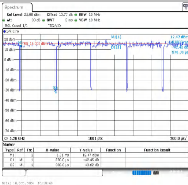
NTVN-11AC20MIMO-Ant1-5280
