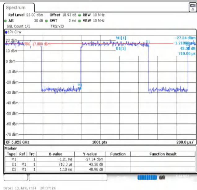
NTNV-11A-Ant2-5825
