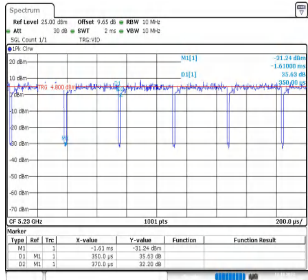
NTNV-11AC40MIMO-Ant2-5230
