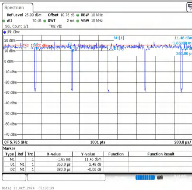
NTNV-11AC20MIMO-Ant1-5785
