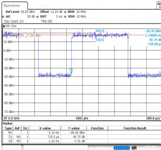
NTNV-11A-Ant1-5500
