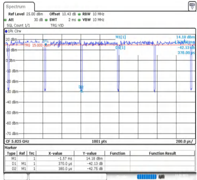
NTVN-11AC20MIMO-Ant2-5825
