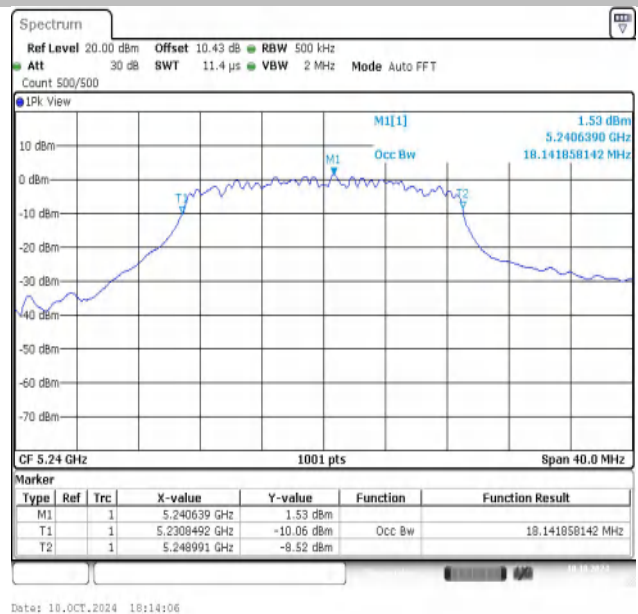
11AC20MIMO-Ant2-5240
