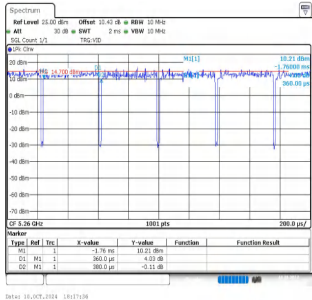
NTVN-11AC20MIMO-Ant2-5260
