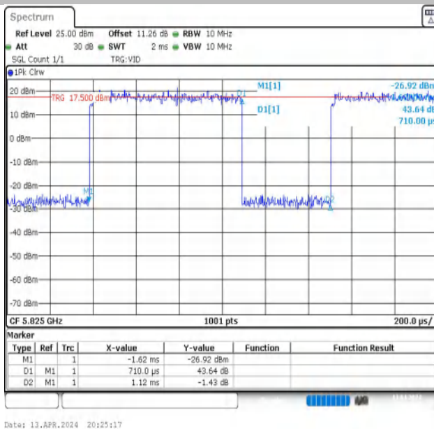
NTNV-11A-Ant1-5825
