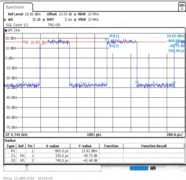
NTNV-11N20MIMO-Ant2-5745
