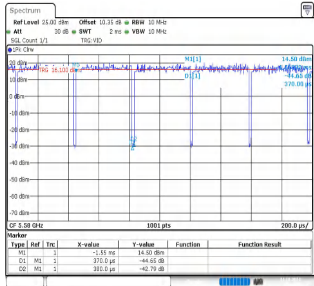
NTVN-11AC20MIMO-Ant2-5580
