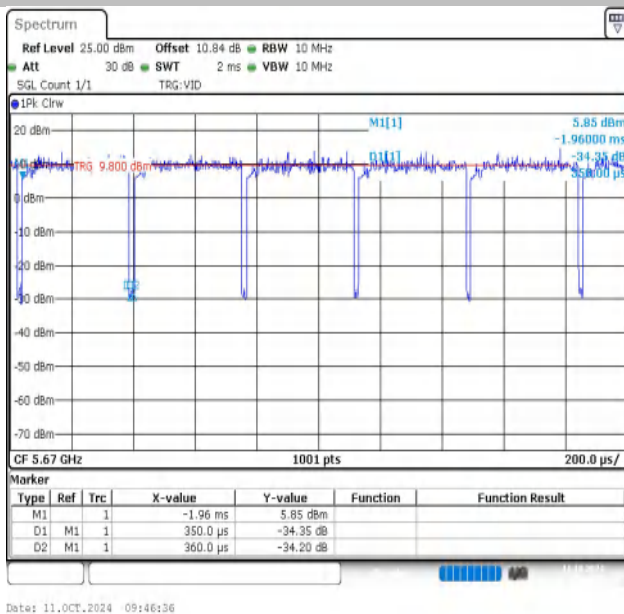
NTNV-11AC40MIMO-Ant1-5670
