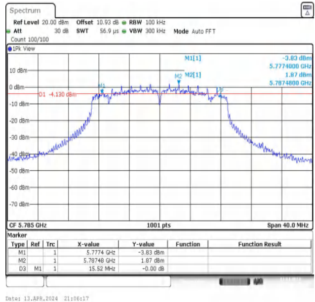
11N20MIMO-Ant2-5785-PASS
