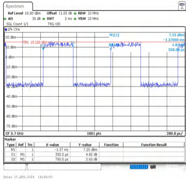
NTNV-11N20MIMO-Ant2-5700
