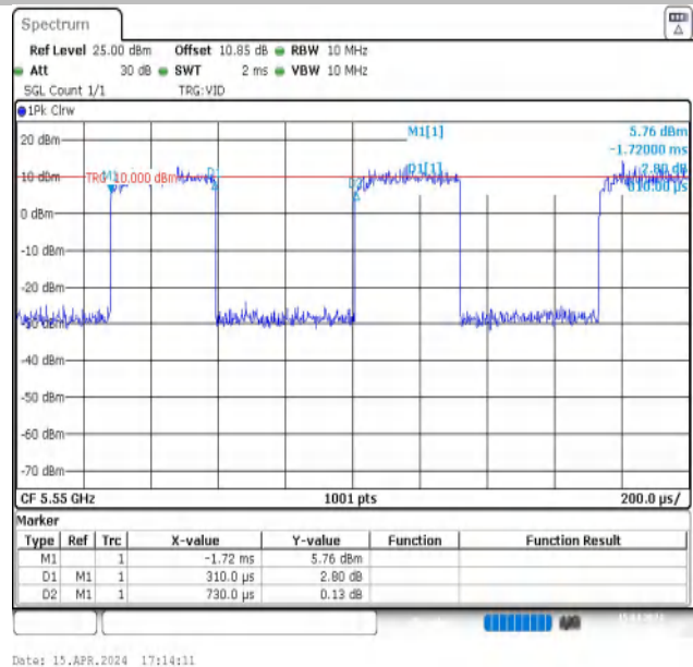
NTNV-11N40MIMO-Ant2-5550
