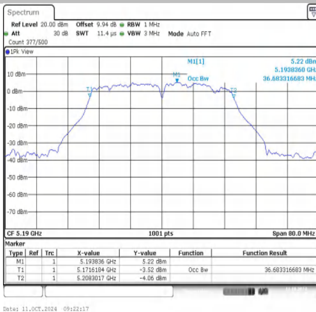
11AC40MIMO-Ant1-5190
