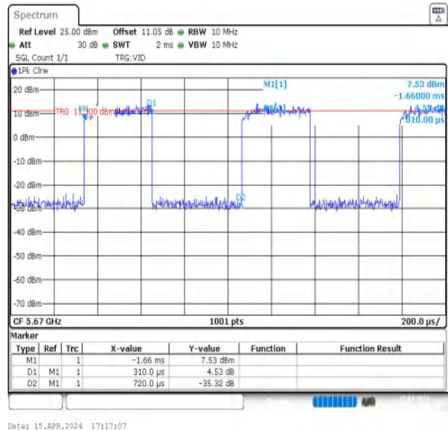
NTNV-11N40MIMO-Ant2-5670
