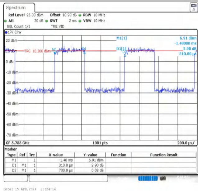
NTNV-11N40MIMO-Ant2-5755
