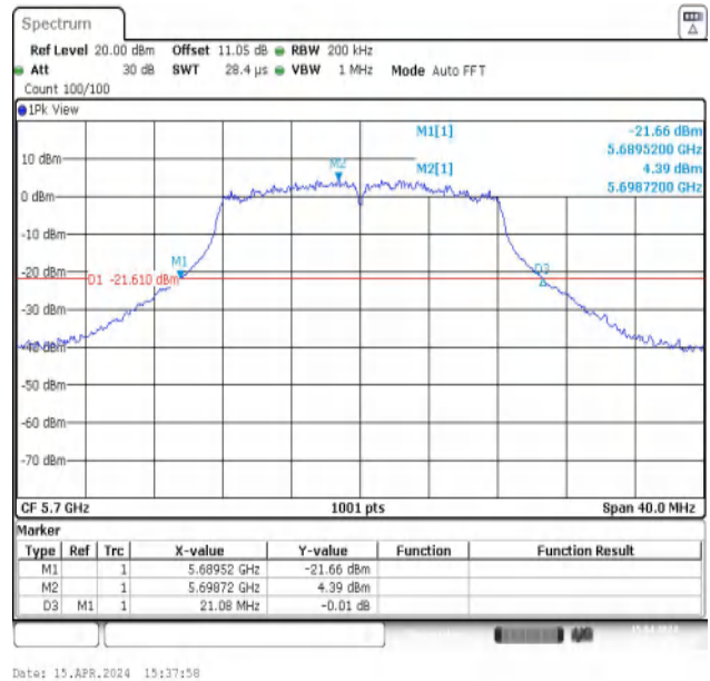
11A-Ant2-5700
