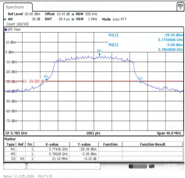
11AC20MIMO-Ant2-5785
