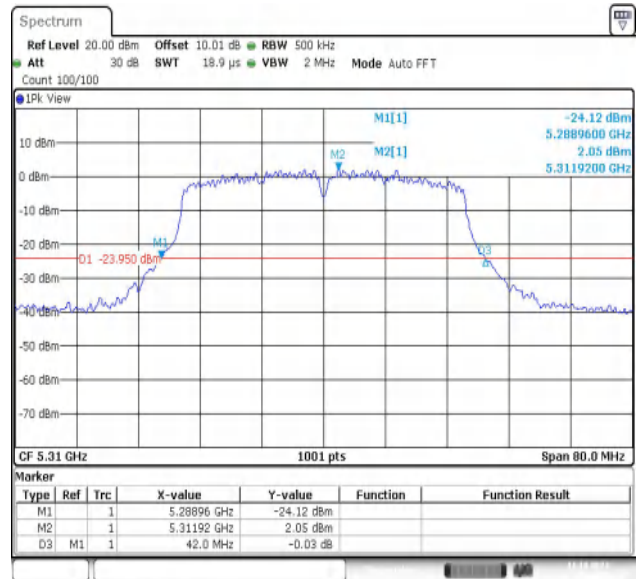
11AC40MIMO-Ant2-5310
