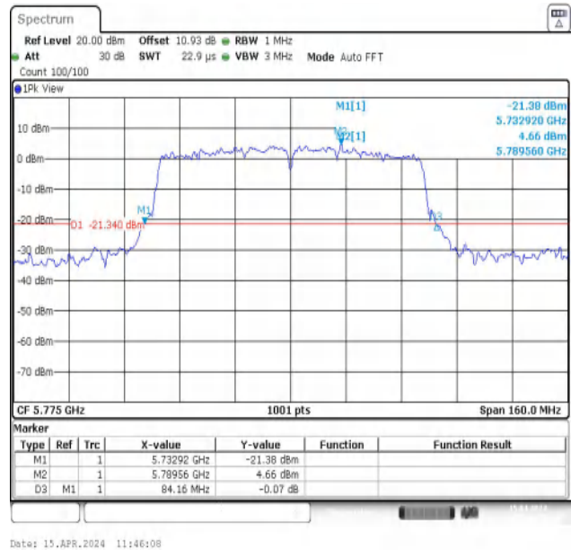
11AC80MIMO-Ant2-5775
