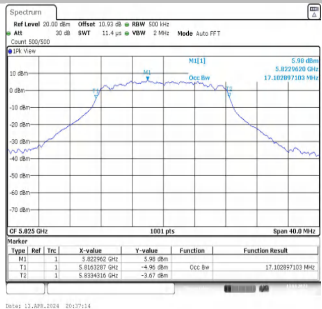
11A-Ant2-5825
