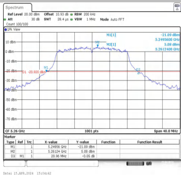
11A-Ant2-5260
