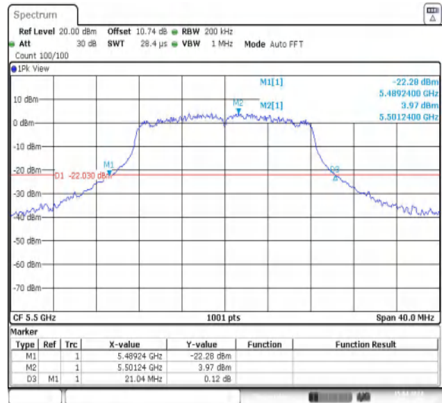
11A-Ant2-5500
