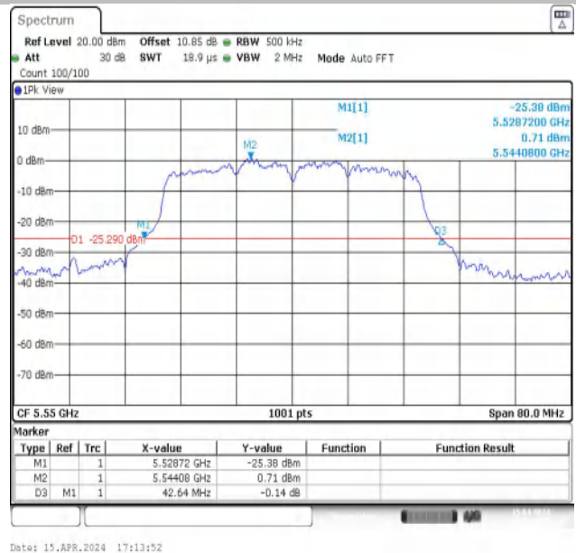
11N40MIMO-Ant2-5550
