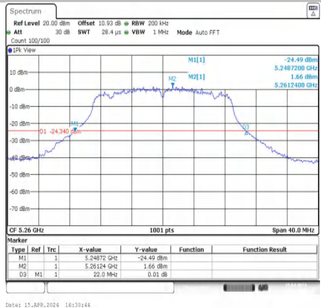
11N20MIMO-Ant2-5260
