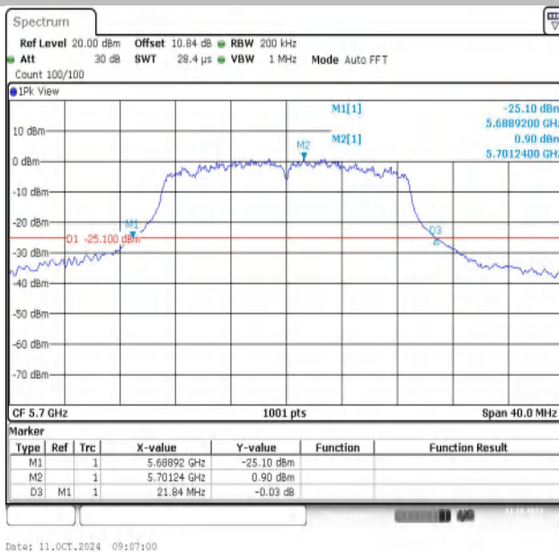
11AC20MIMO-Ant1-5700
