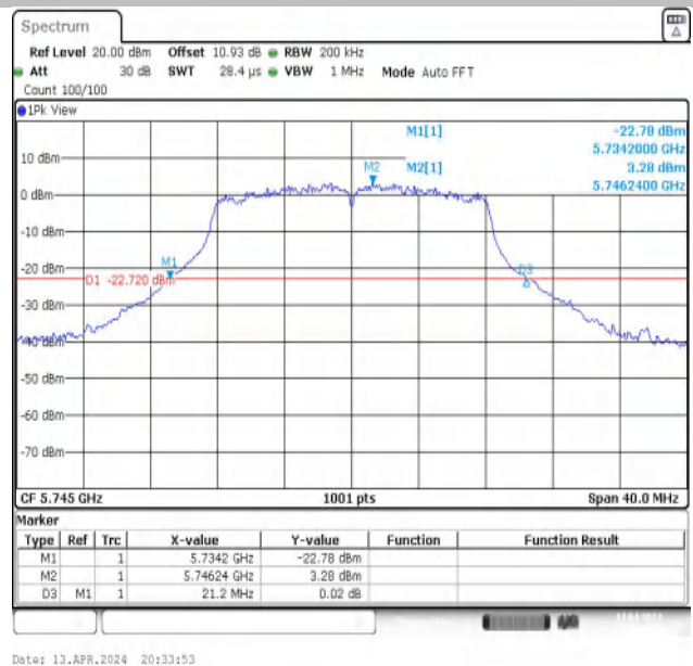
11A-Ant2-5745
