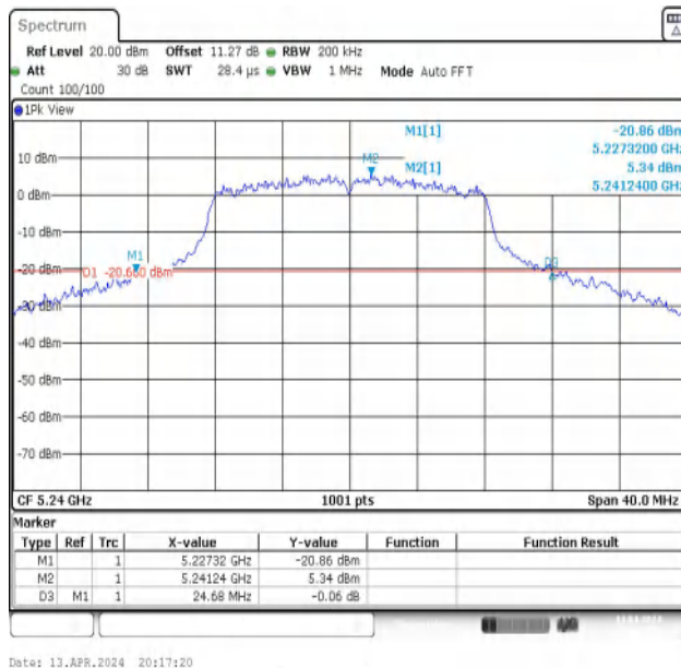
11A-Ant1-5240
