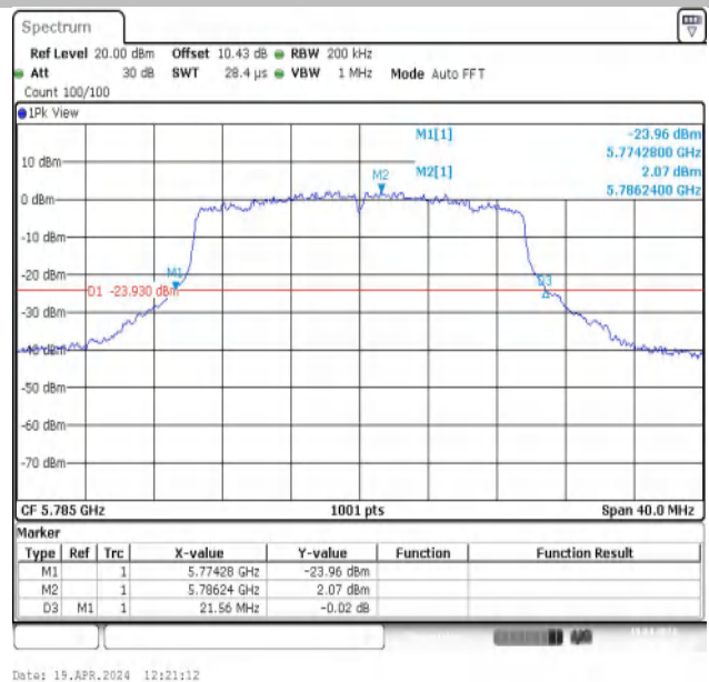
11AX20MIMO-Ant2-5785
