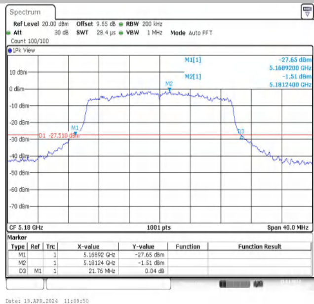
11AX20MIMO-Ant2-5180
