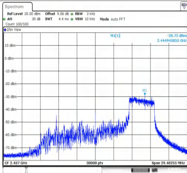
11AX20MIMO-Ant1-2437-52Tone-RU37-PASS
