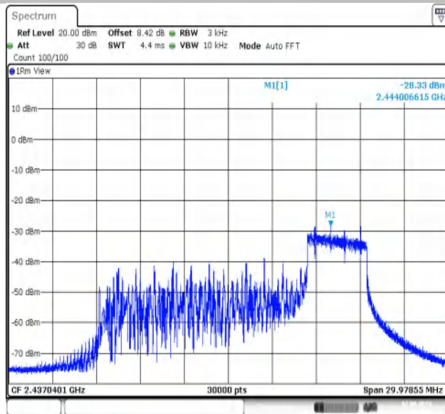
11AX20MIMO-Ant2-2437-52Tone-RU37-PASS
