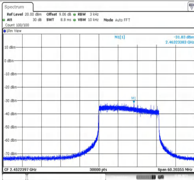
11AX40MIMO-Ant1-2452-242Tone-RU61-PASS
