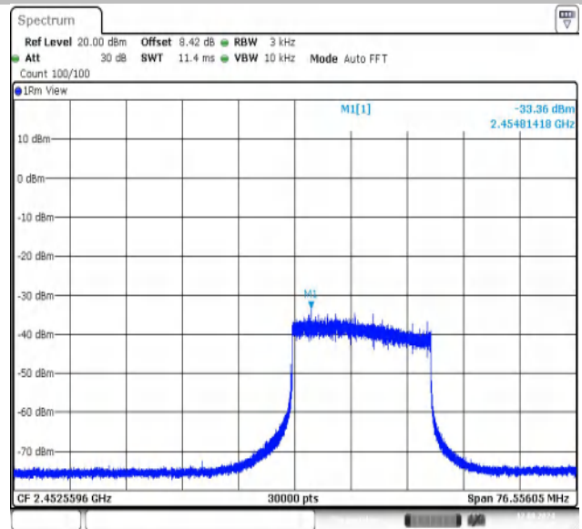
11AX40MIMO-Ant2-2452-242Tone-RU61-PASS
