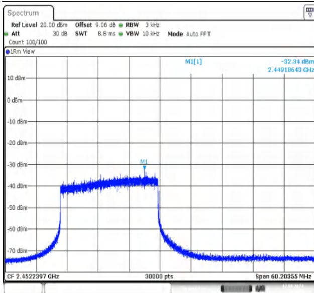
11AX40MIMO-Ant1-2452-242Tone-RU61-PASS
