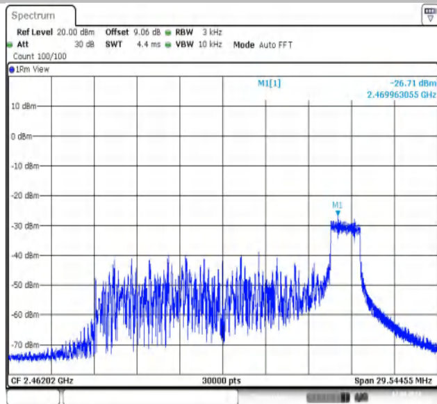
11AX20MIMO-Ant1-2462-26Tone-RU0-PASS
