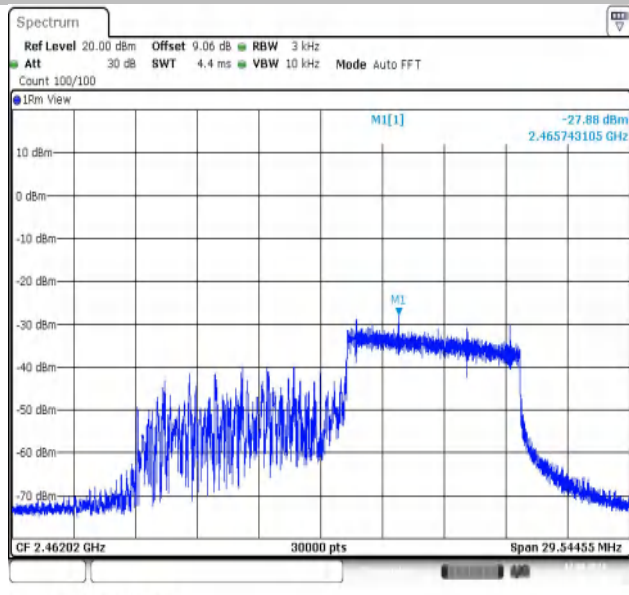
11AX20MIMO-Ant1-2462-106Tone-RU53-PASS
