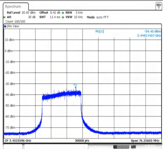
11AX40MIMO-Ant2-2452-242Tone-RU61-PASS
