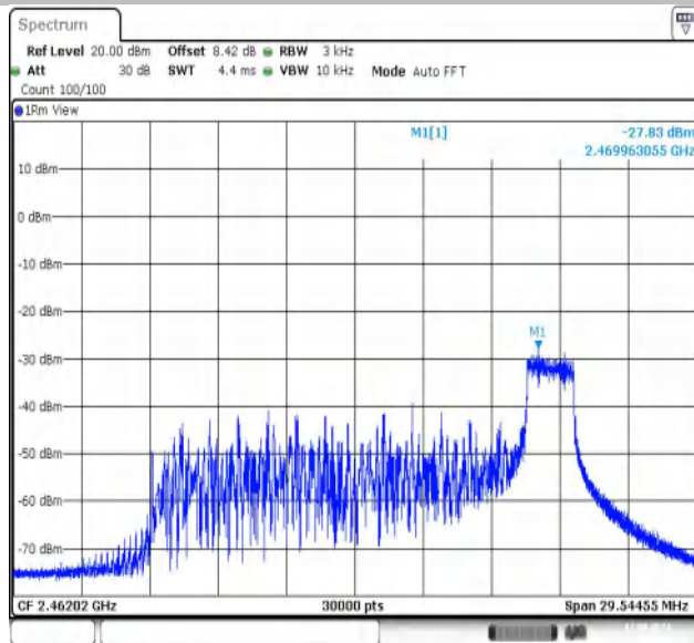
11AX20MIMO-Ant2-2462-26Tone-RU0-PASS
