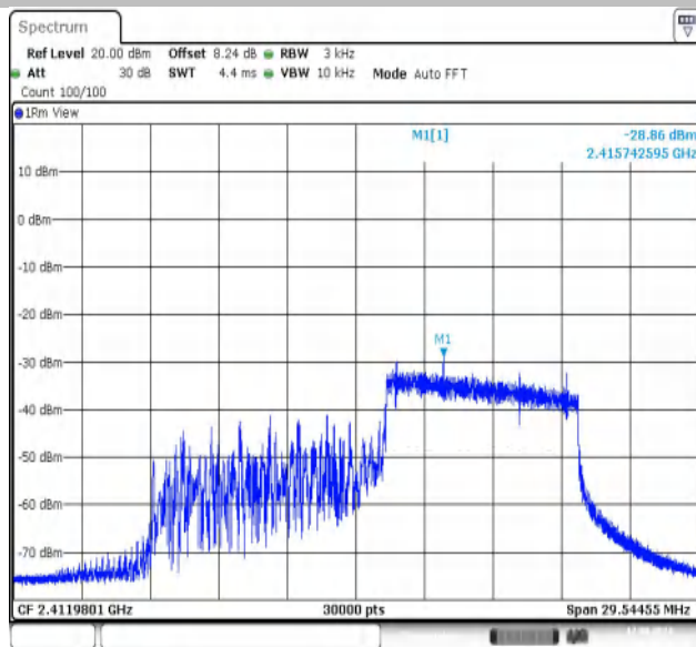
11AX20MIMO-Ant2-2412-106Tone-RU53-PASS
