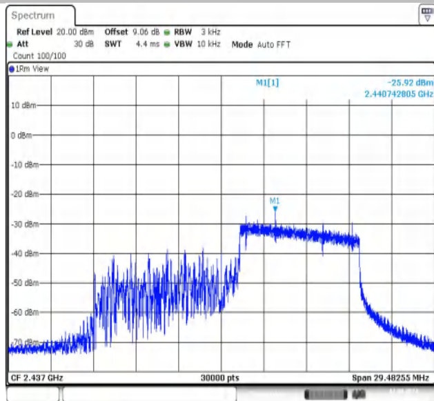
11AX20MIMO-Ant1-2437-106Tone-RU53-PASS
