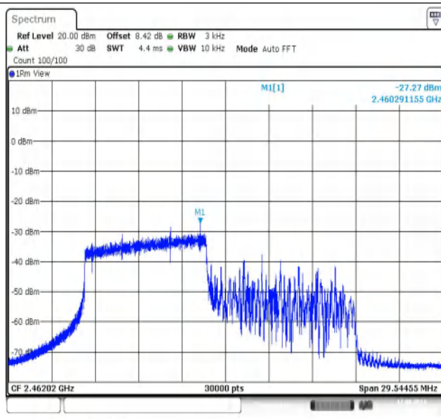
11AX20MIMO-Ant2-2462-106Tone-RU53-PASS
