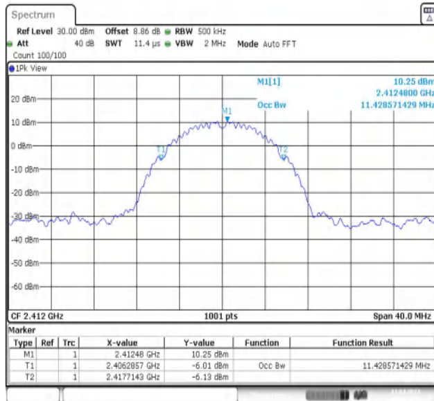
11B-Ant1-2412
