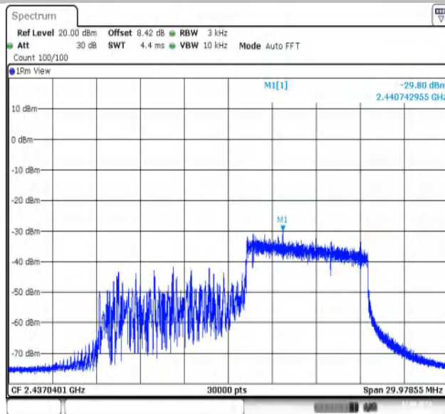
11AX20MIMO-Ant2-2437-106Tone-RU53-PASS
