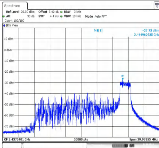
11AX20MIMO-Ant2-2437-26Tone-RU0-PASS
