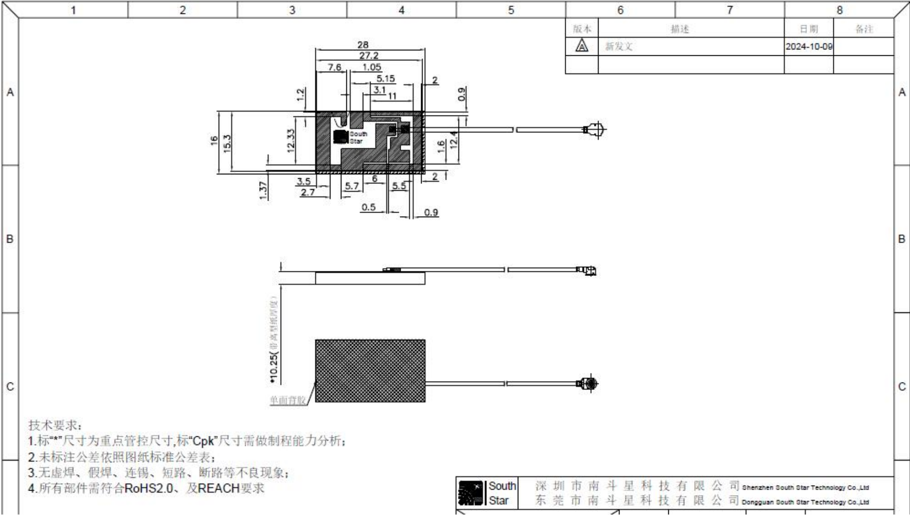
Antenna Drawing
