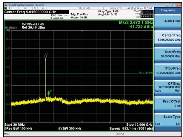
30 MHz – 10 GHz
