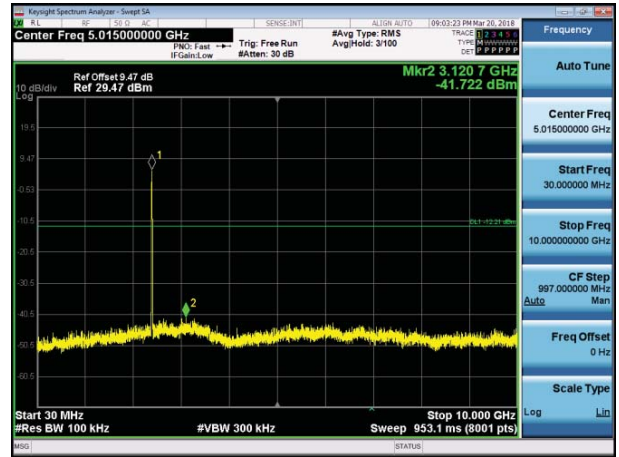
30 MHz – 10 GHz
