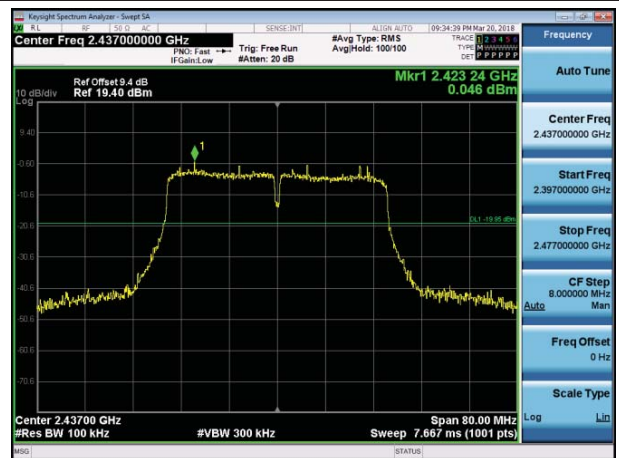
2397 MHz – 2477 MHz
