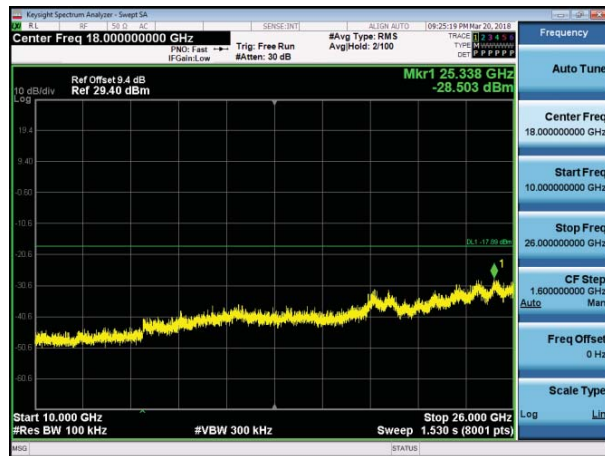
10 GHz – 26 GHz
