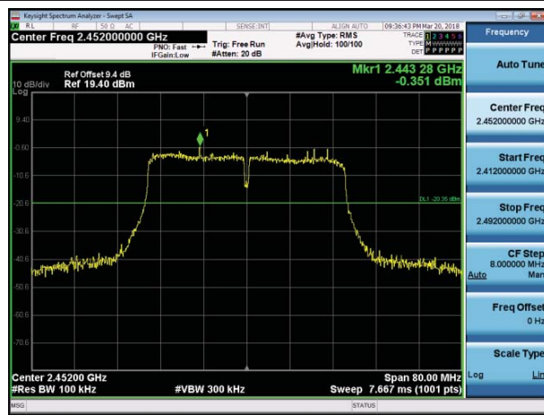
2412 MHz – 2492 MHz
