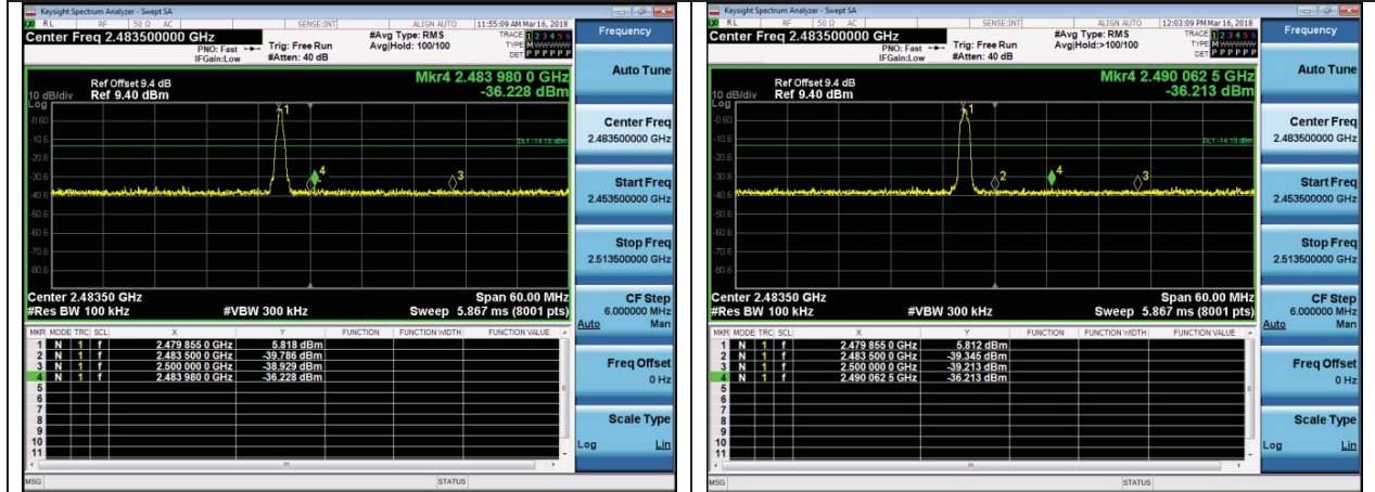
Channel 78 / 2480 MHz – Non-Hopping
