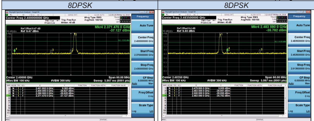
Channel 0 / 2402 MHz – Non-Hopping
