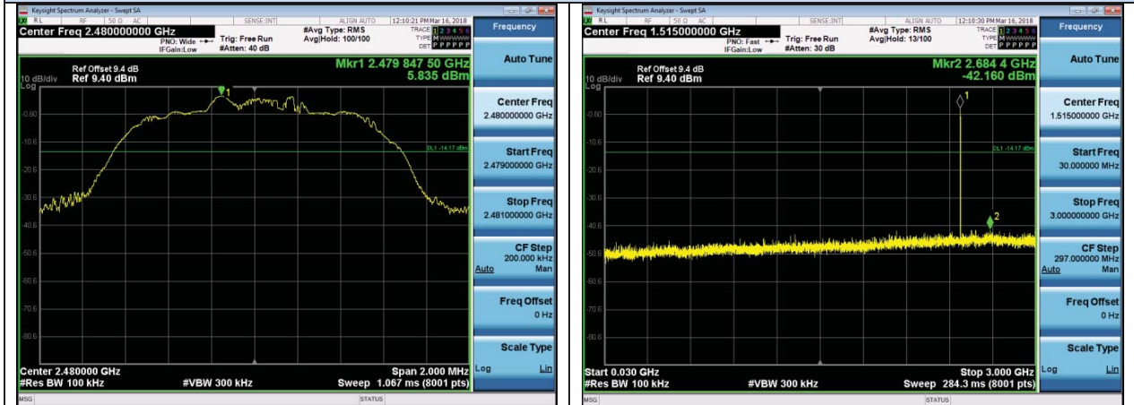
2479 MHz – 2481 MHz
