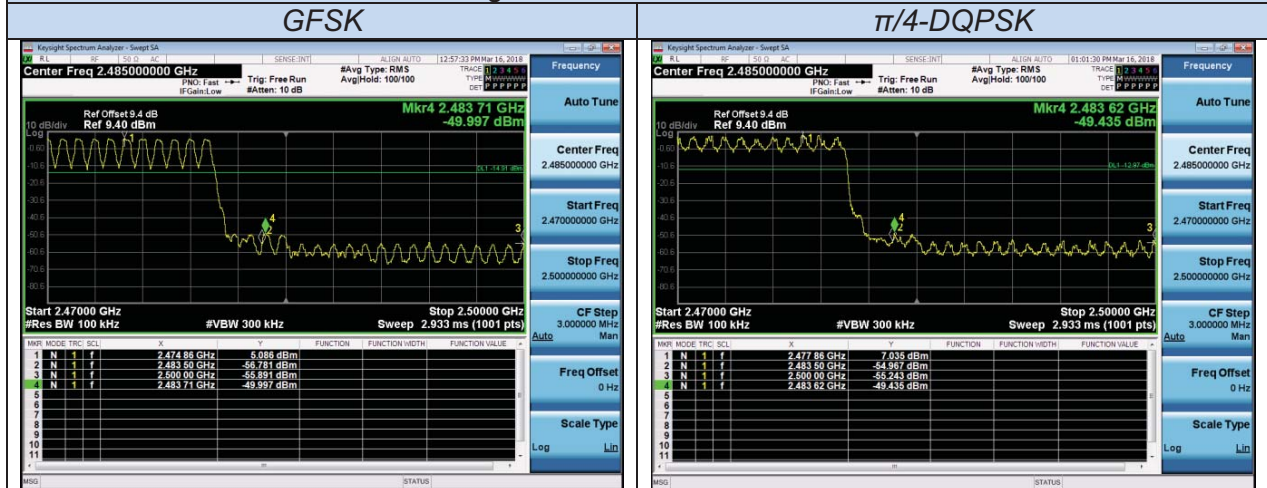
Channel 78 / 2480 MHz – Hopping
