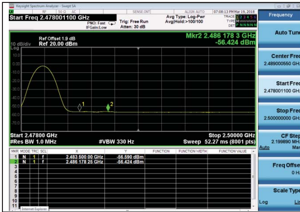
Channel 78 / 2480 MHz – Non-Hopping–Average 8DPSK
