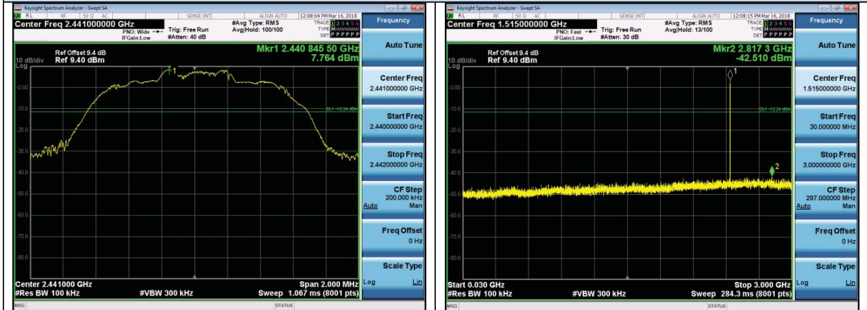
2440 MHz – 2442 MHz
