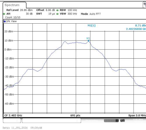
BLE_1M-Ant1-2402-0~Reference-PASS
