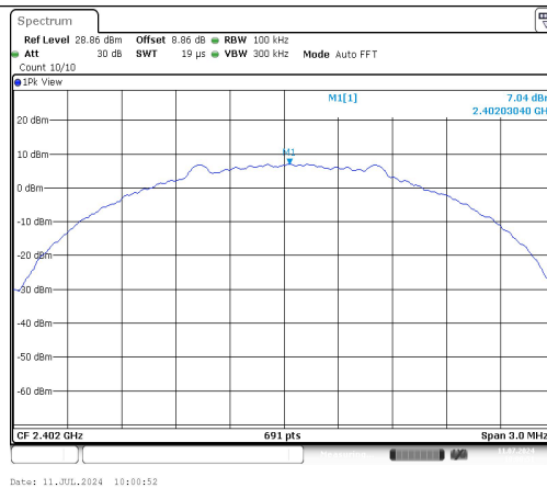
BLE_2M-Ant1-2402-0~Reference-PASS
