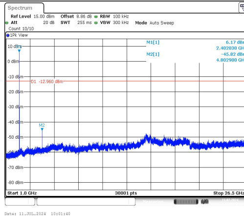
BLE_2M-Ant1-2402-1000~26500-PASS
