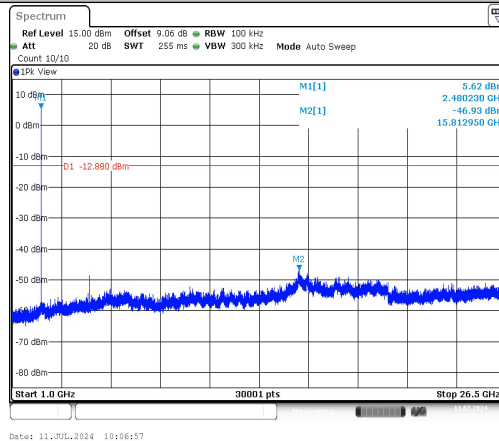
BLE_2M-Ant1-2480-1000~26500-PASS
