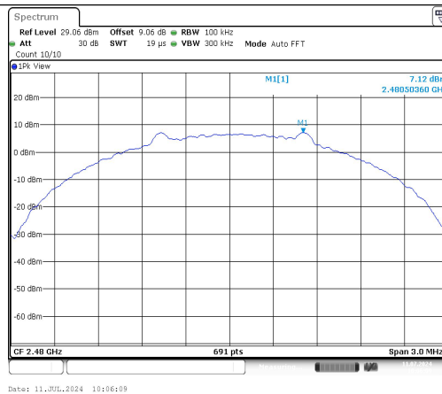
BLE_2M-Ant1-2480-0~Reference-PASS
