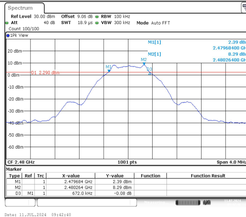
BLE_1M-Ant1-2480-PASS
