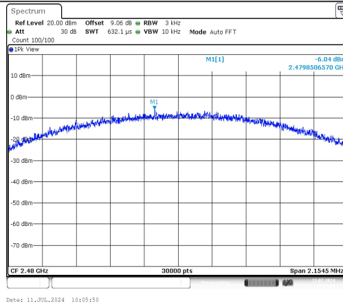
BLE_2M-Ant1-2480-PASS
