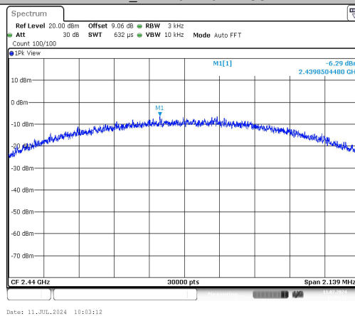
BLE_2M-Ant1-2440-PASS
