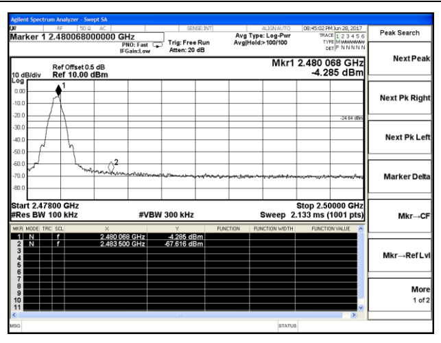
Channel 39 / 2480 MHz
