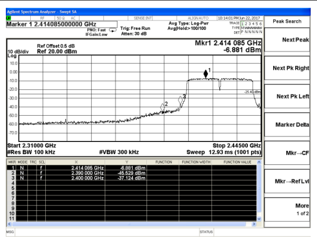
Channel 3 / 2422 MHz
