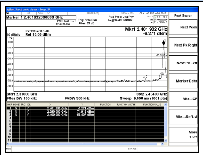
Channel 0 / 2402 MHz
