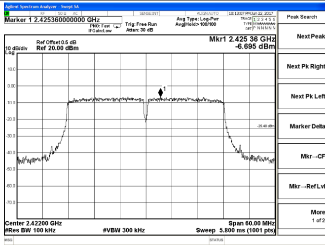
2392 MHz – 2452 MHz
