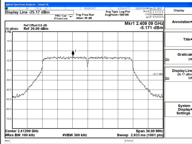
2397 MHz – 2427 MHz
