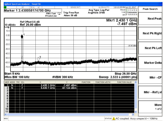
9 KHz – 26.5 GHz
