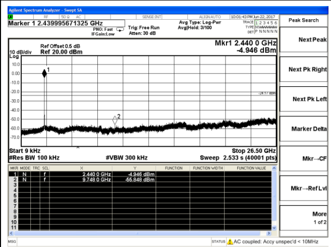
9 KHz – 26.5 GHz
