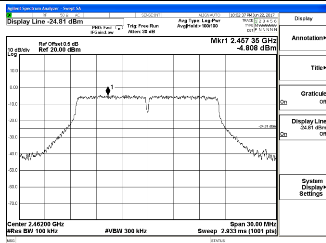
2447 MHz – 2477 MHz
