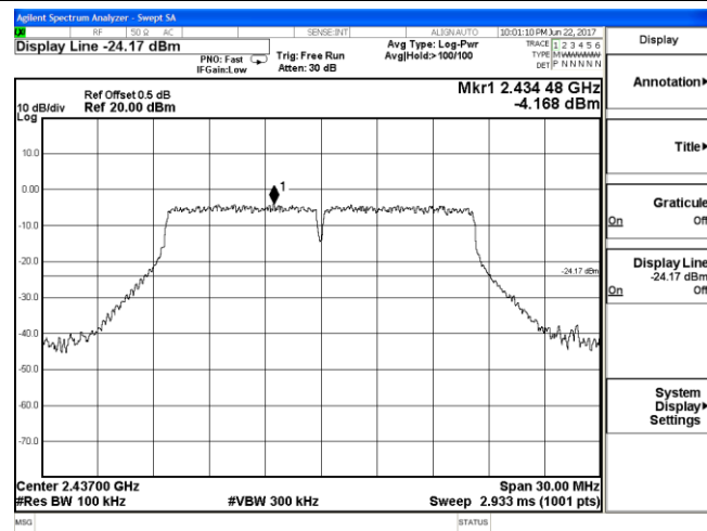
2422 MHz – 2452 MHz
