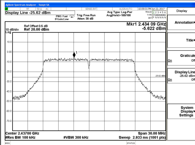
2422 MHz – 2452 MHz
