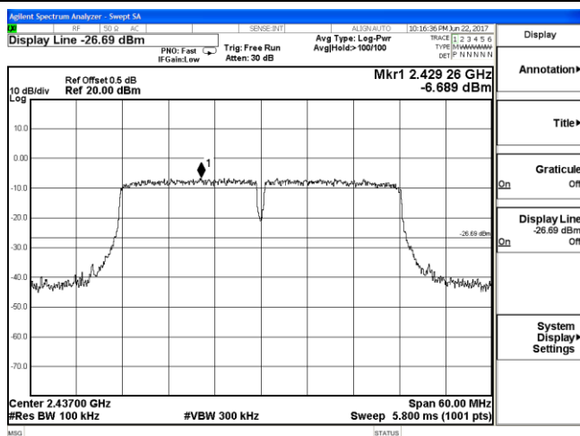
2407 MHz – 2467 MHz
