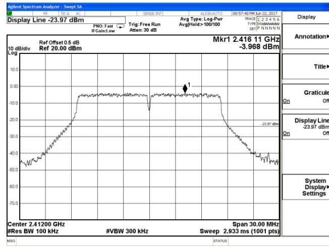
2397 MHz – 2427 MHz
