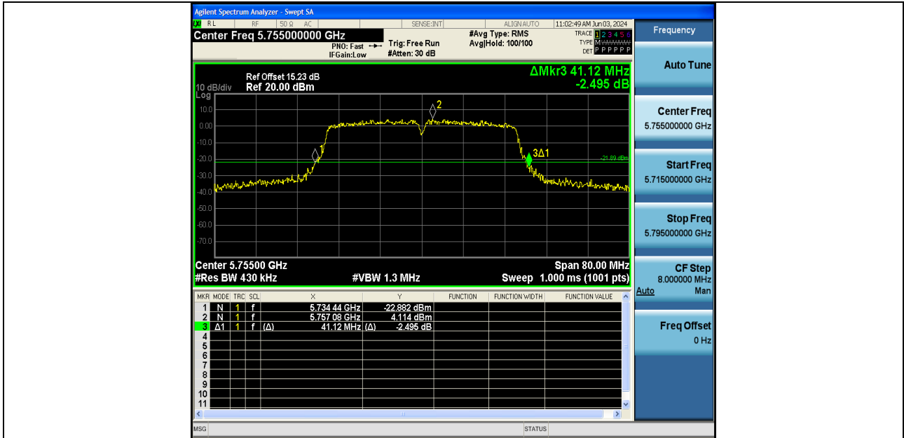
11AX40SISO-Ant2-5755
