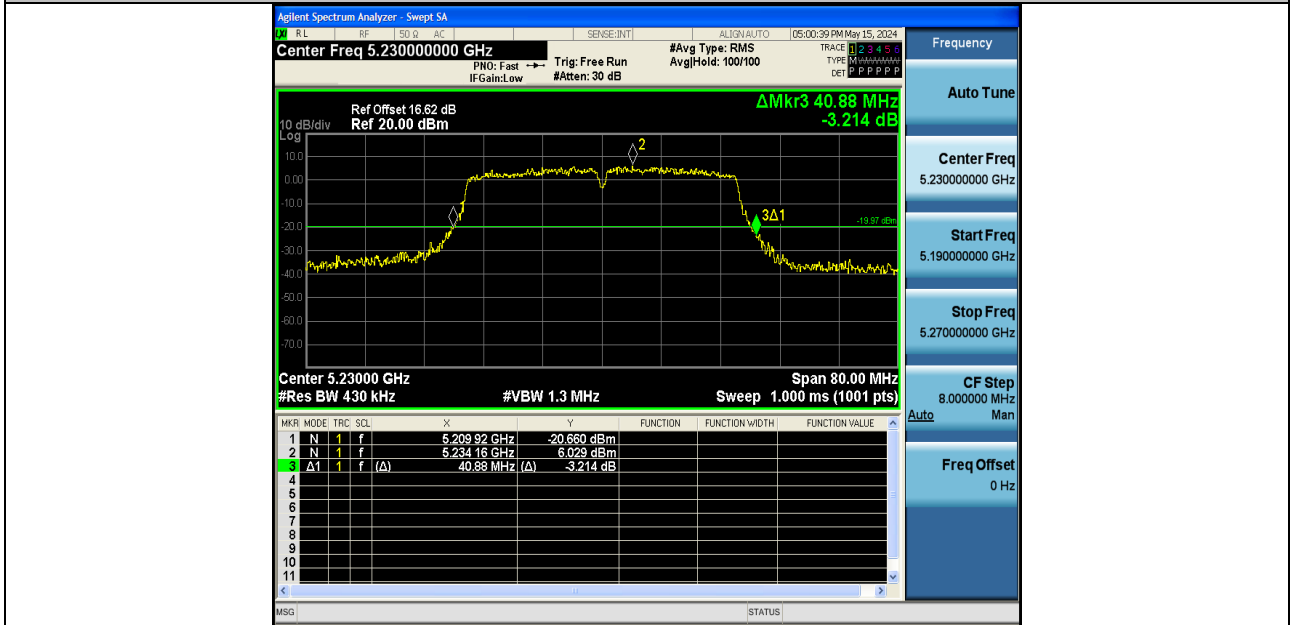
11AX40SISO-Ant1-5230
