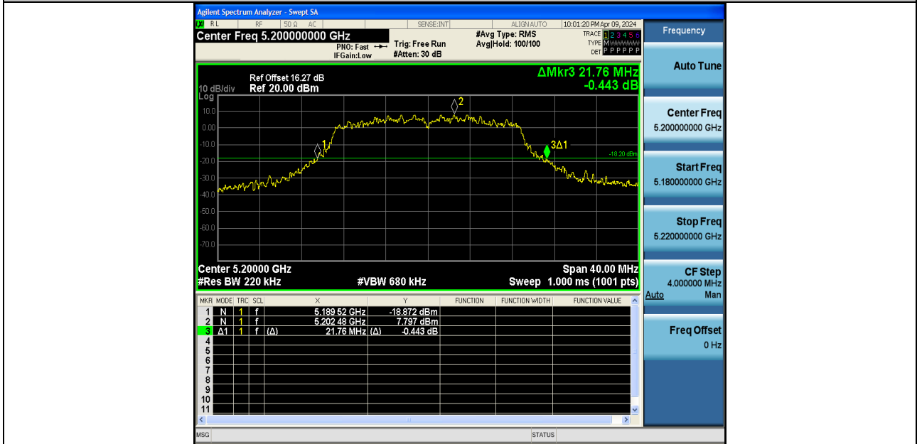
11AC20SISO-Ant2-5200
