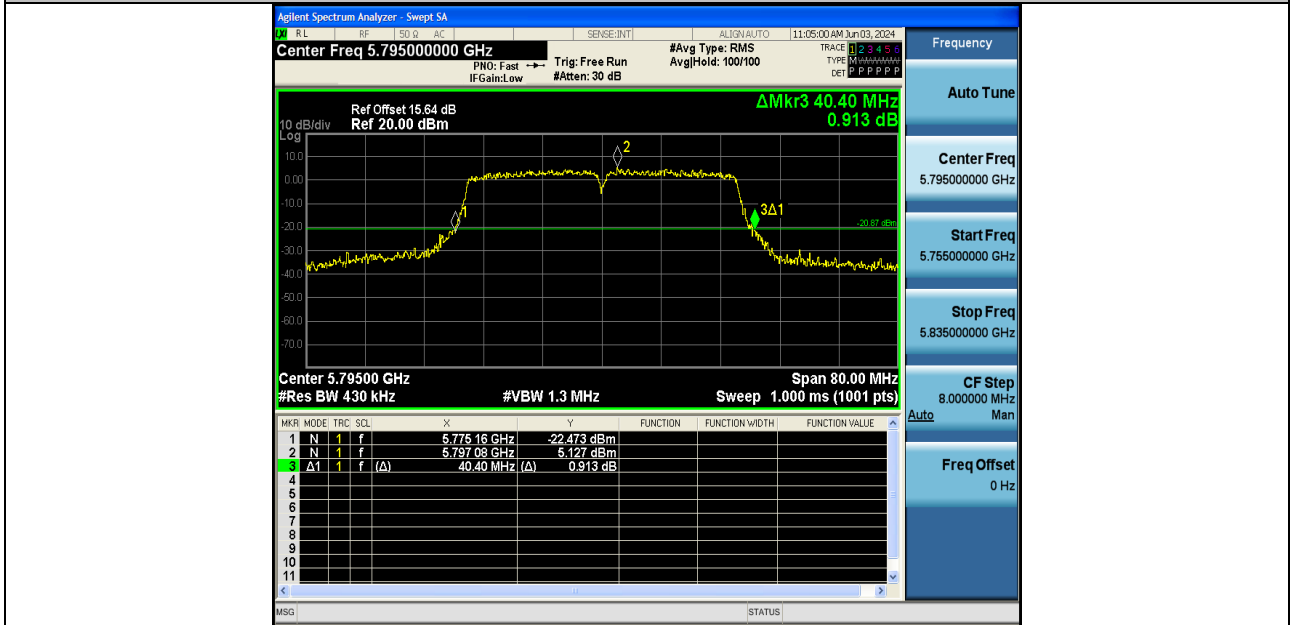
11AX40SISO-Ant2-5795
