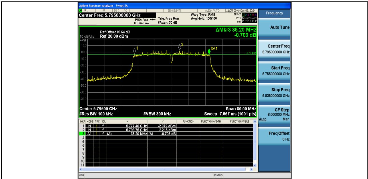
11AX40SISO-Ant2-5795-PASS
