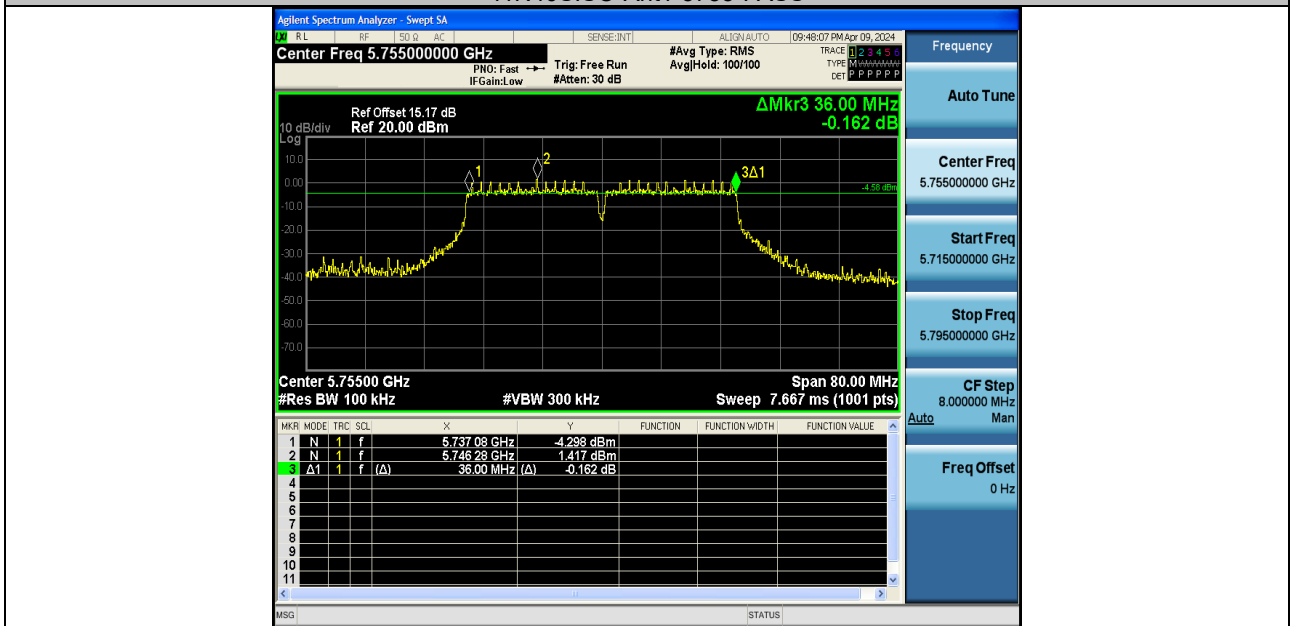
11N40SISO-Ant2-5755-PASS
