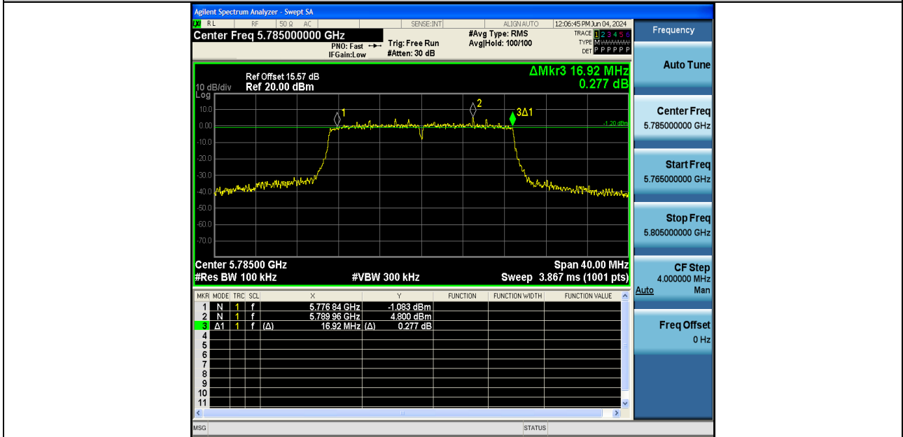
11AX20SISO-Ant1-5785-PASS
