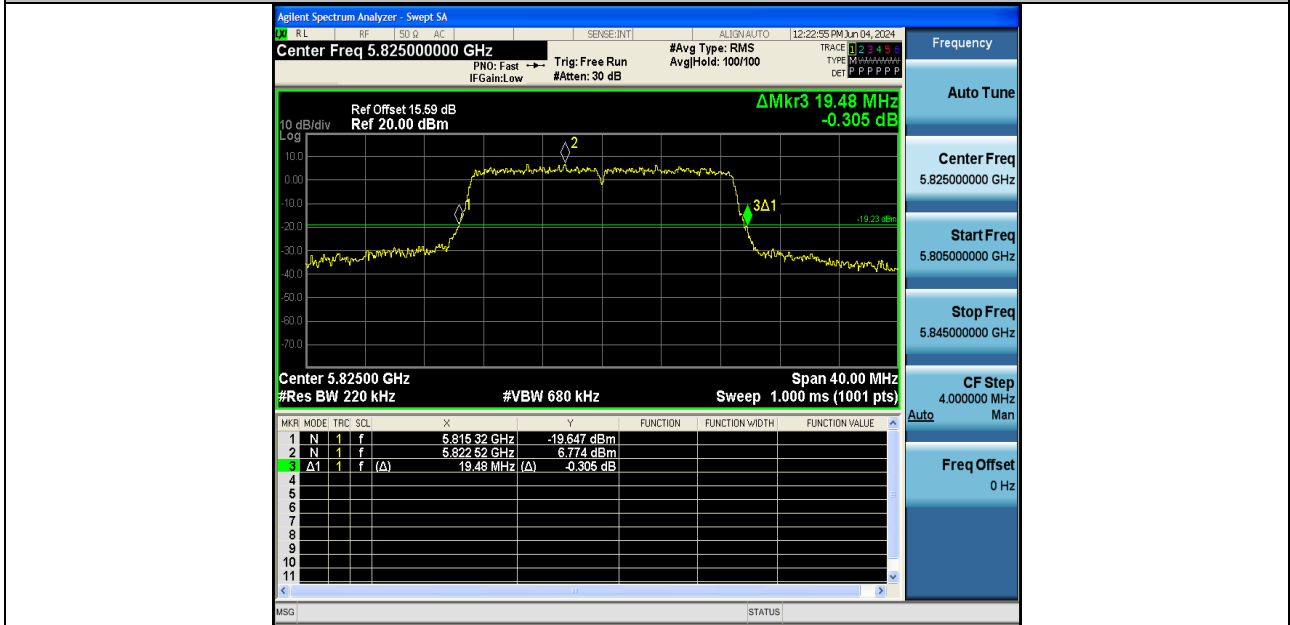
11AX20SISO-Ant2-5825
