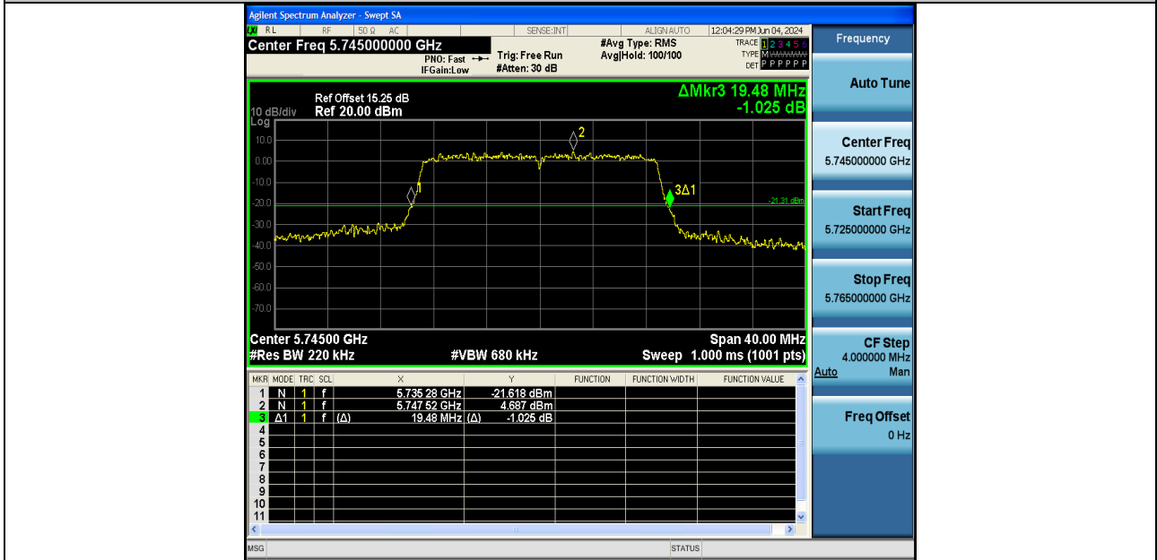
11AX20SISO-Ant1-5745
