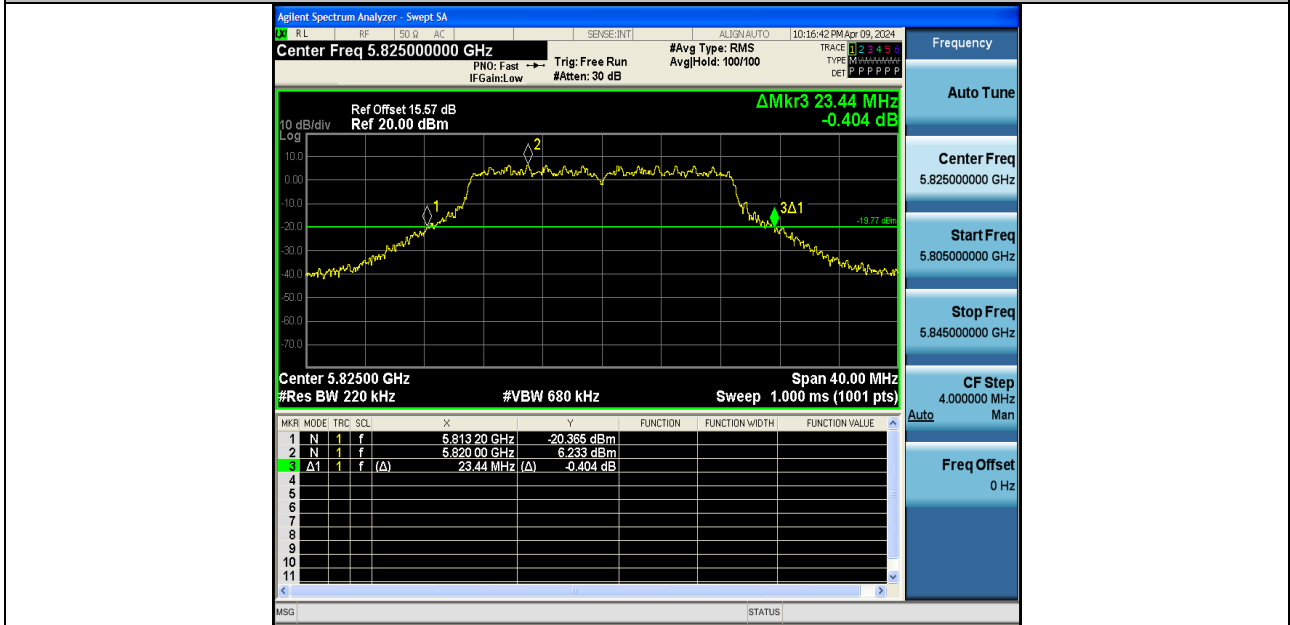
11AC20SISO-Ant2-5825
