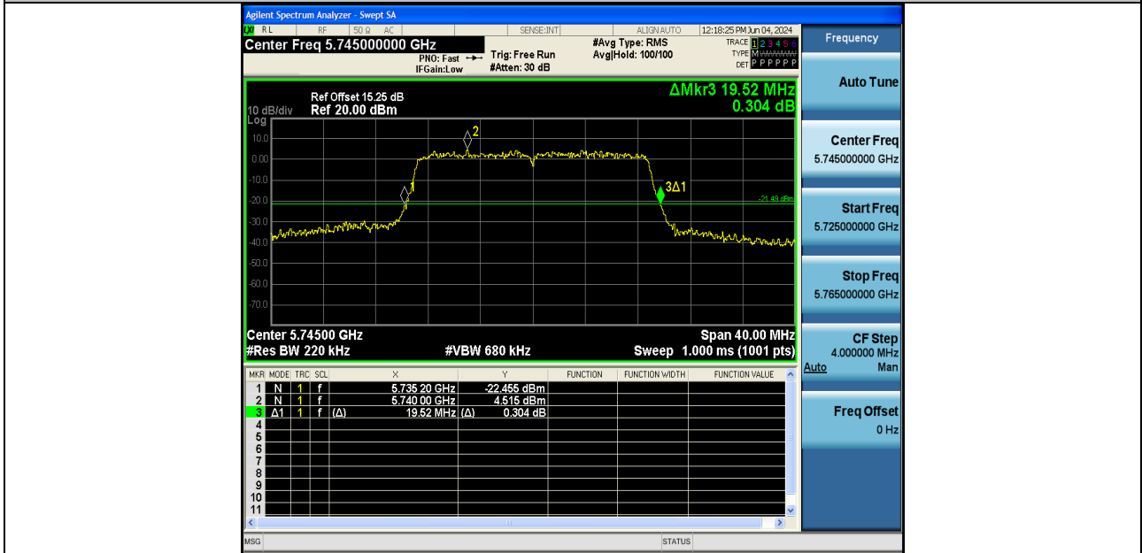
11AX20SISO-Ant2-5745
