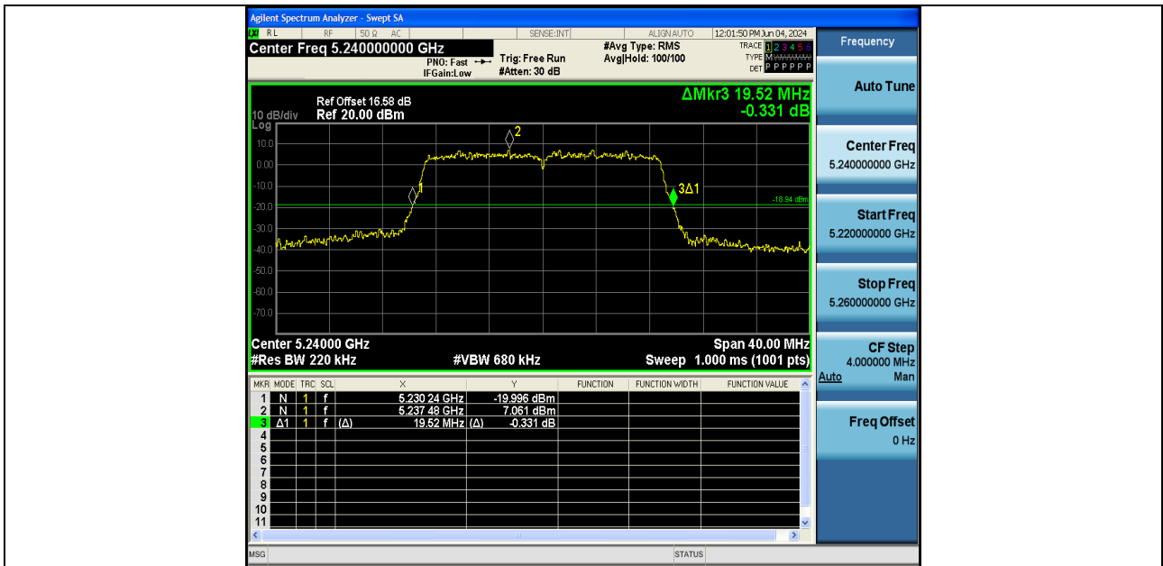
11AX20SISO-Ant1-5240
