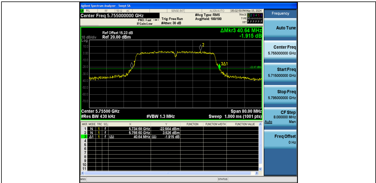
11AX40SISO-Ant1-5755
