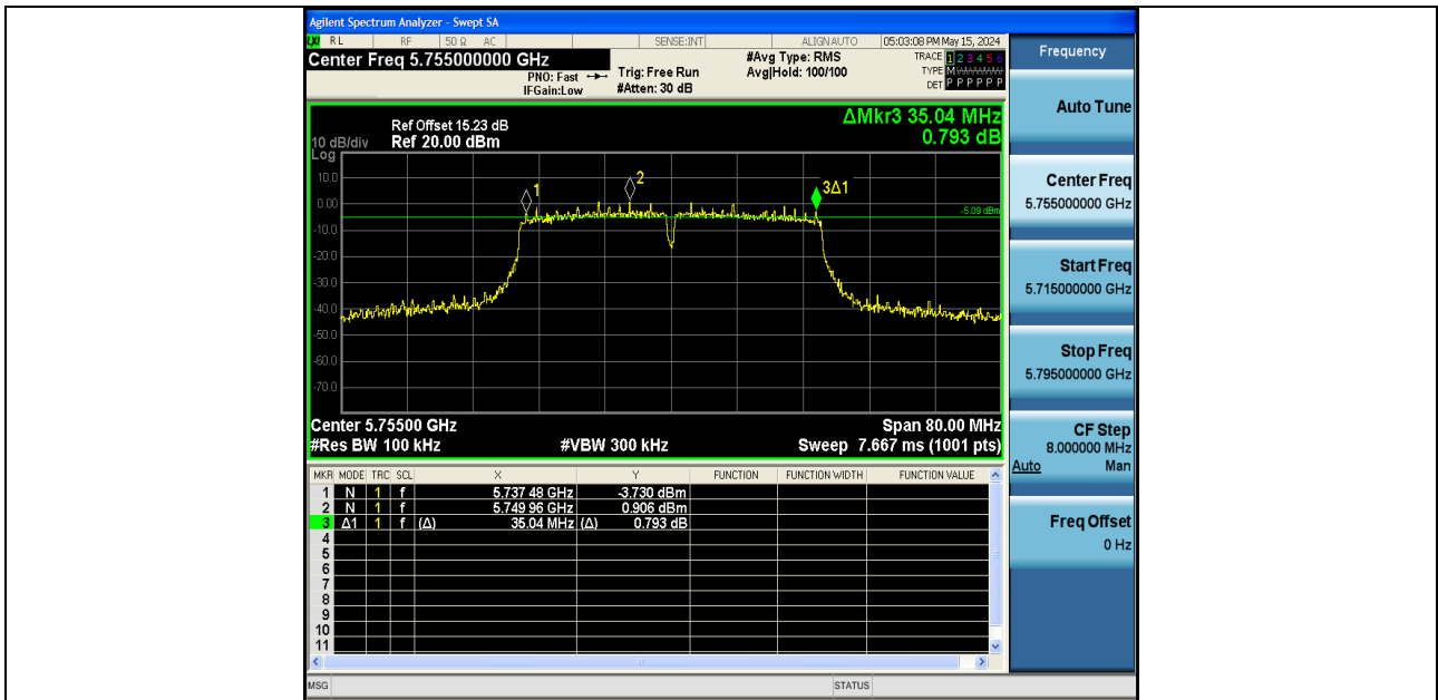
11AX40SISO-Ant1-5755-PASS
