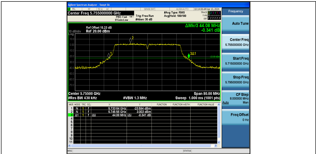
11AC40SISO-Ant1-5755
