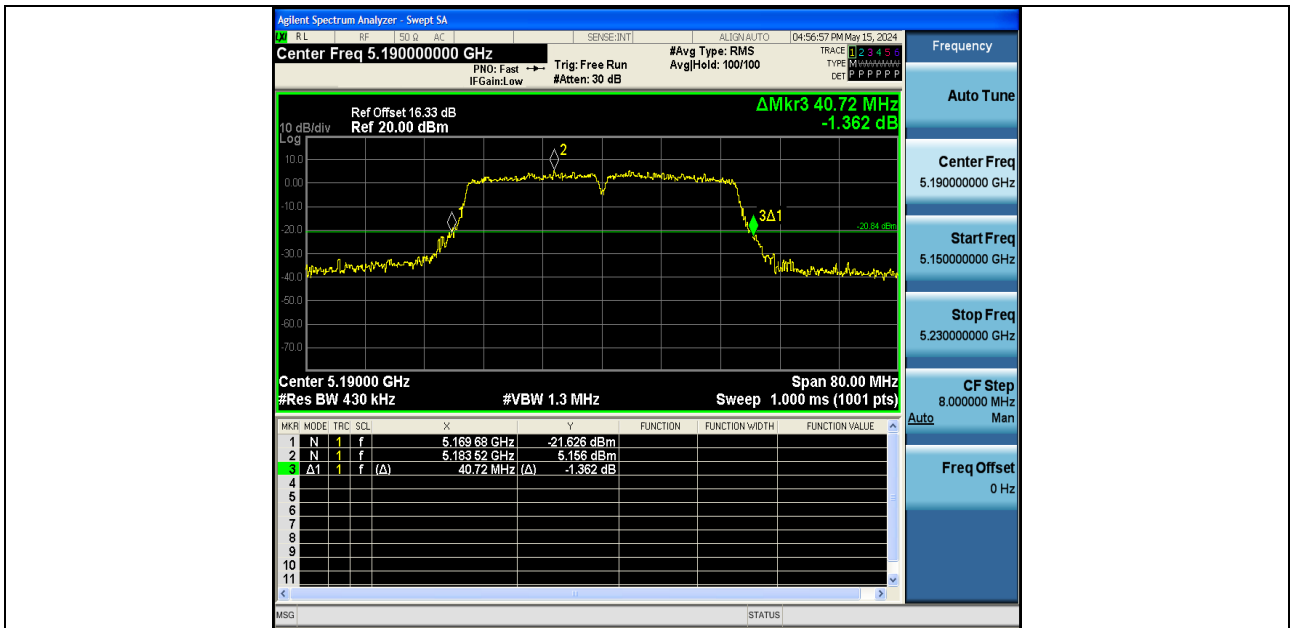
11AX40SISO-Ant1-5190
