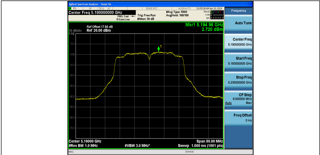
11AC40SISO-Ant1-5190-PASS
