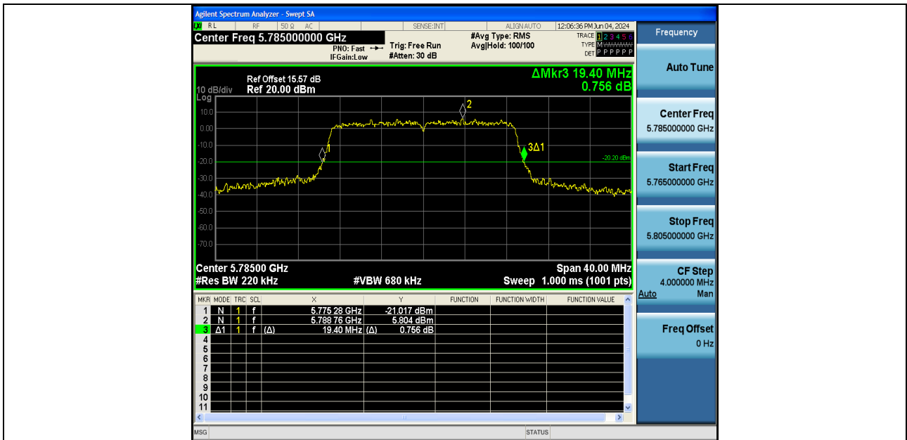
11AX20SISO-Ant1-5785
