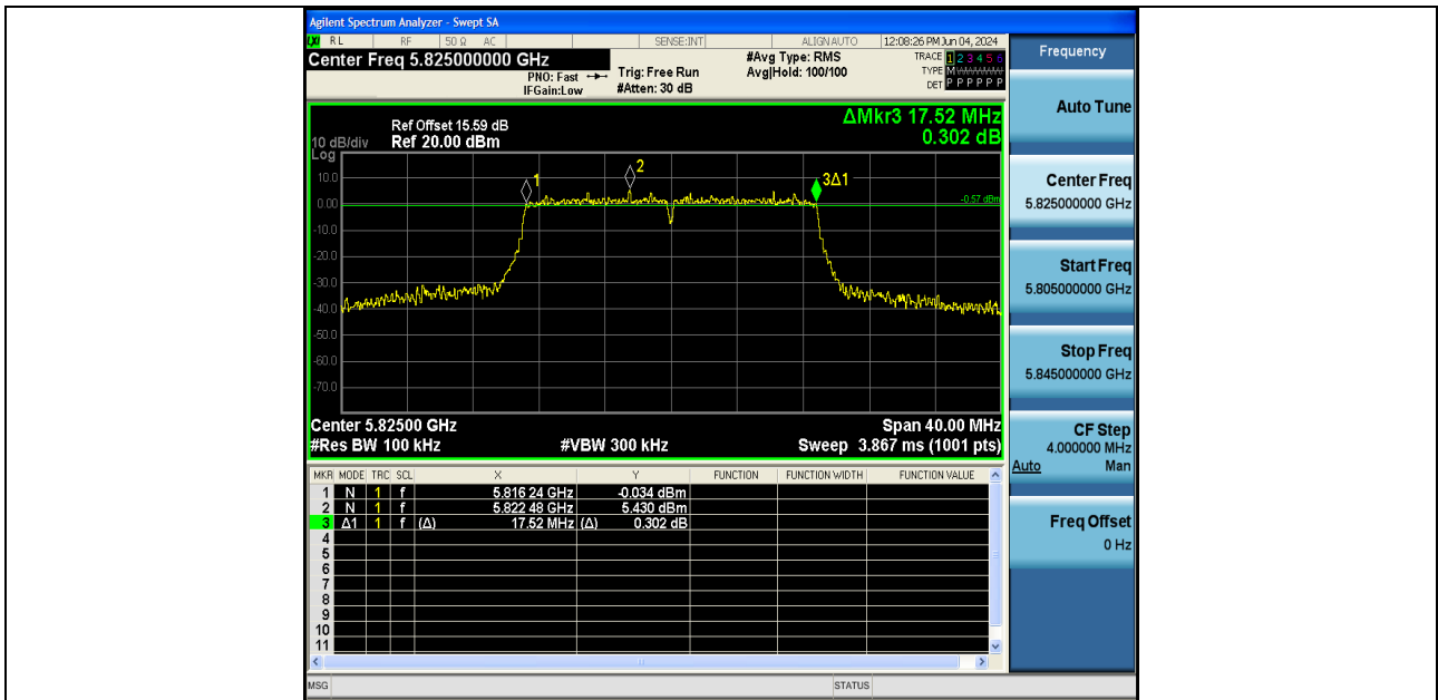
11AX20SISO-Ant1-5825-PASS
