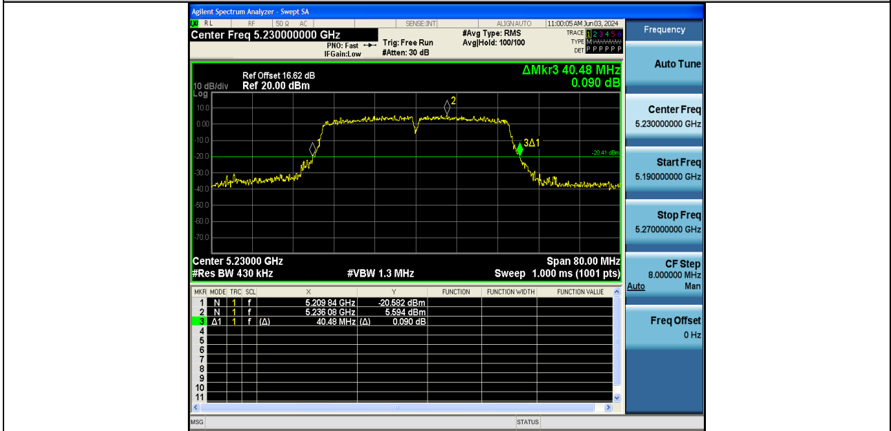
11AX40SISO-Ant2-5230
