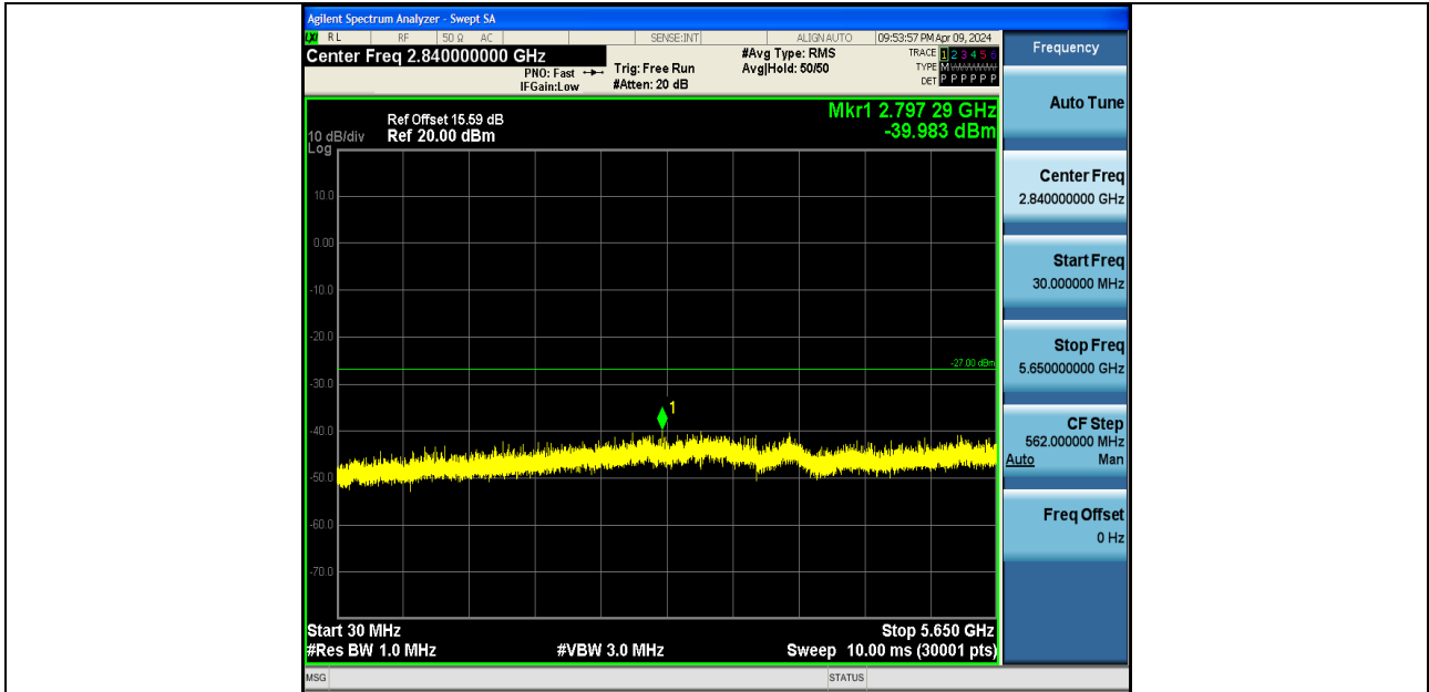
11N40SISO-Ant2-5795-30~5650-PASS
