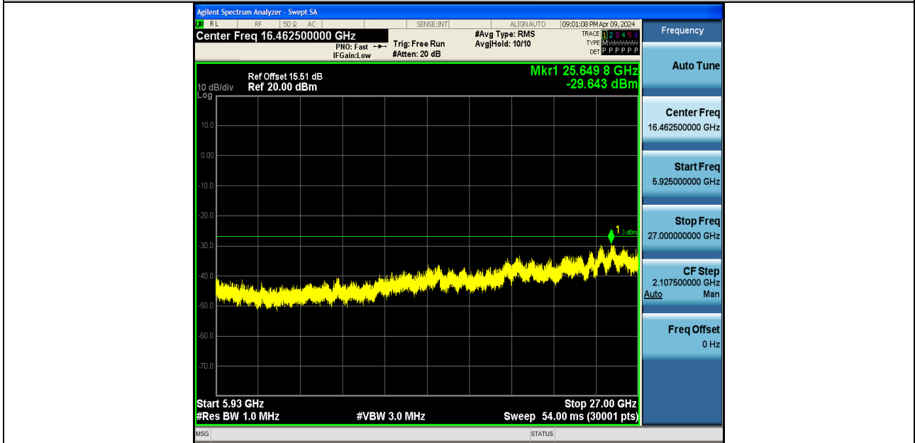
11A-Ant2-5785-5925~27000-PASS
