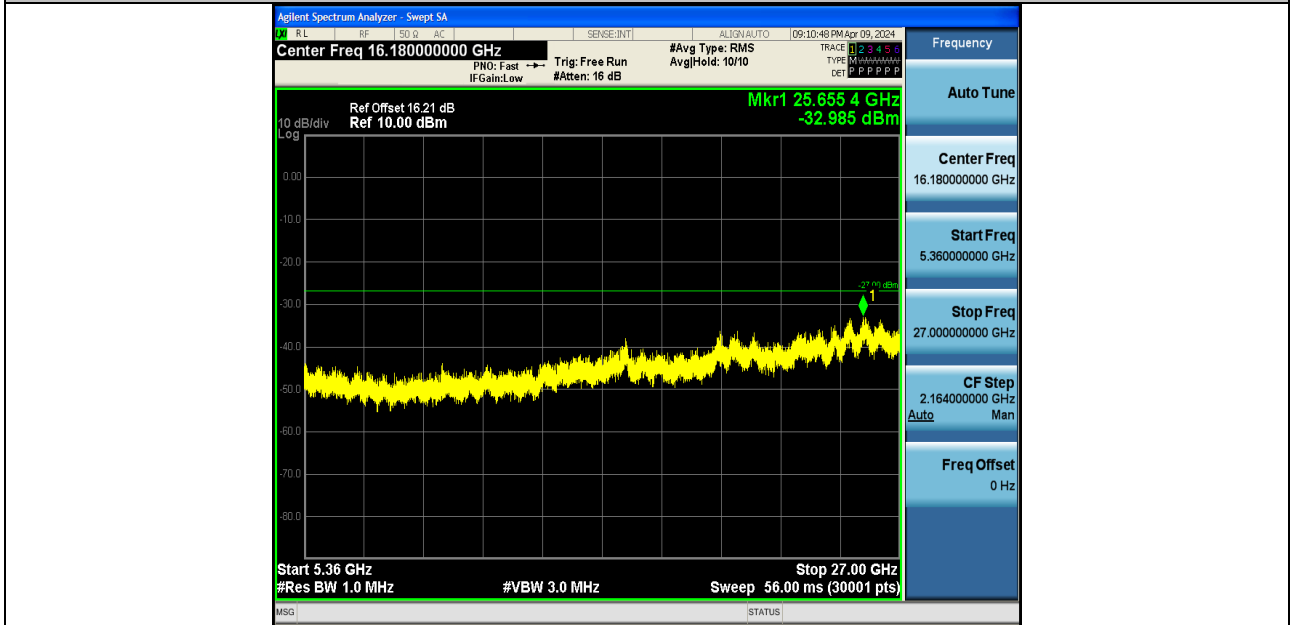
11N20SISO-Ant2-5180-5360~27000-PASS
