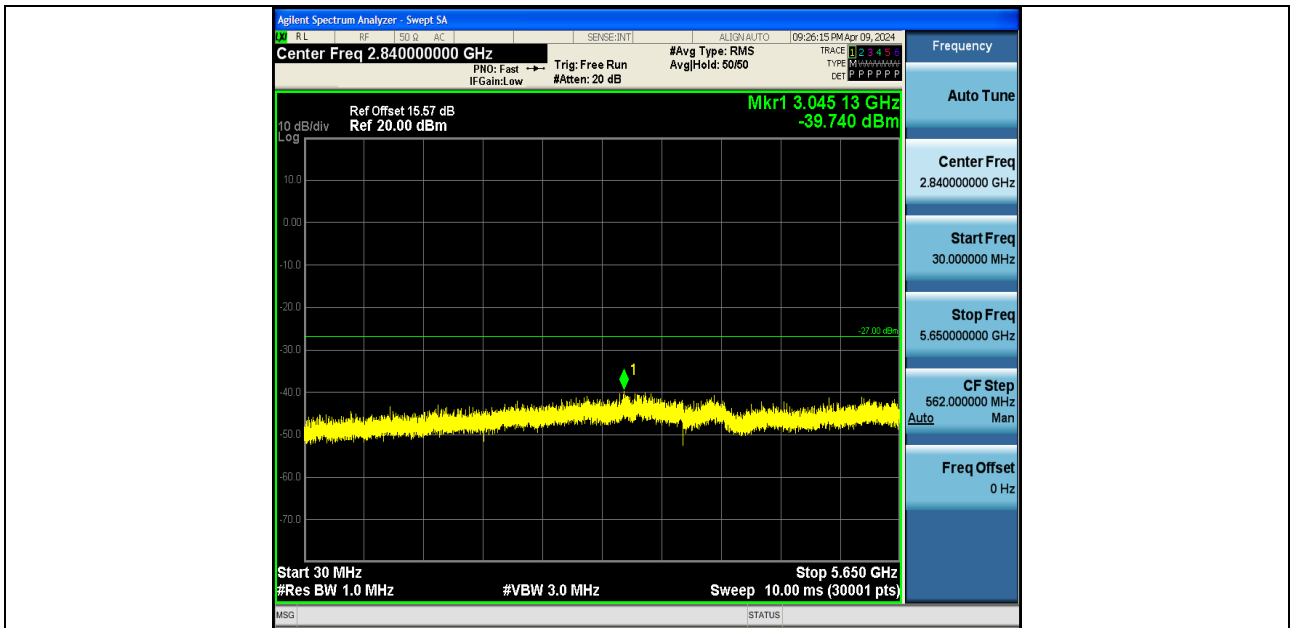
11N20SISO-Ant1-5785-30~5650-PASS
