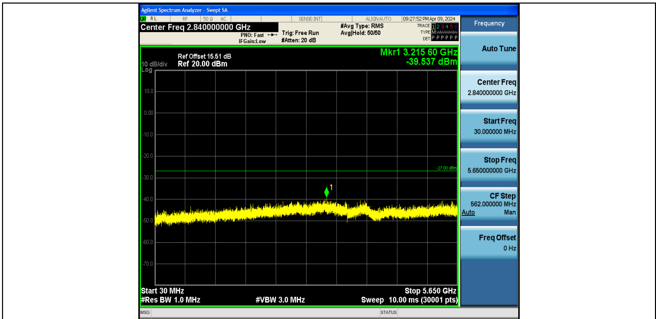
11N20SISO-Ant2-5785-30~5650-PASS
