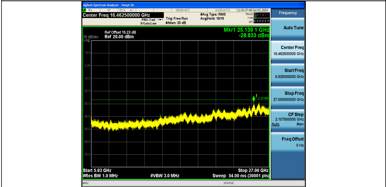
11AX40SISO-Ant2-5755-5925~27000-PASS
