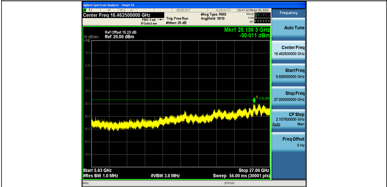
11N40SISO-Ant1-5755-5925~27000-PASS
