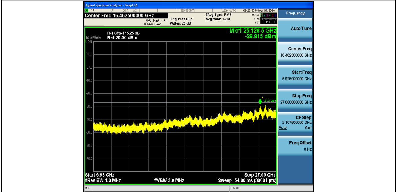
11N20SISO-Ant1-5745-5925~27000-PASS
