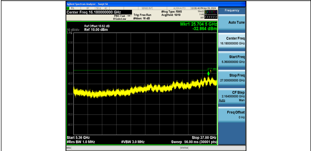
11AC20SISO-Ant2-5240-5360~27000-PASS
