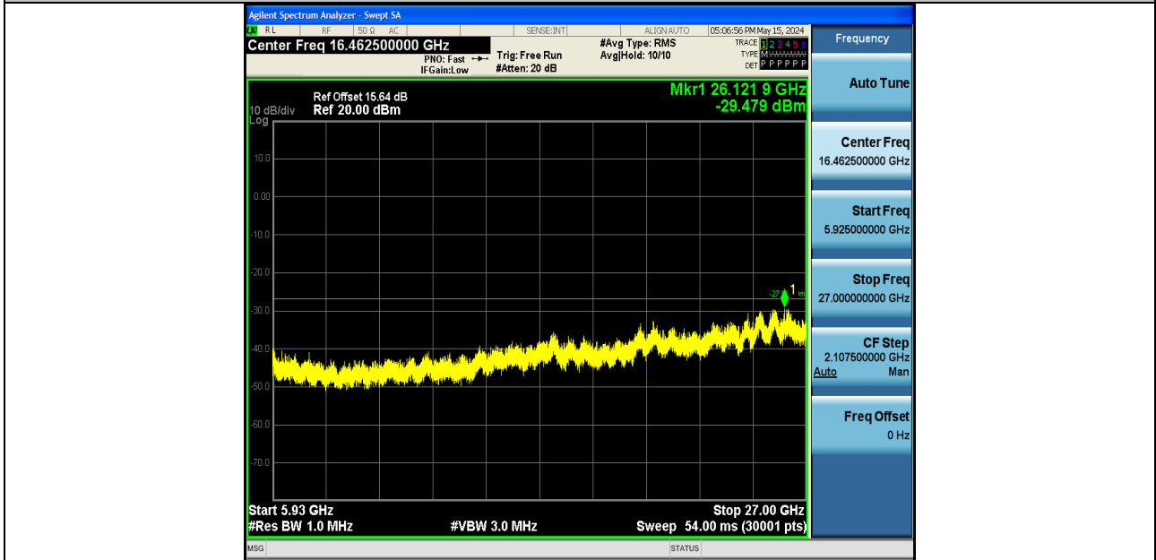
11AX40SISO-Ant1-5795-5925~27000-PASS
