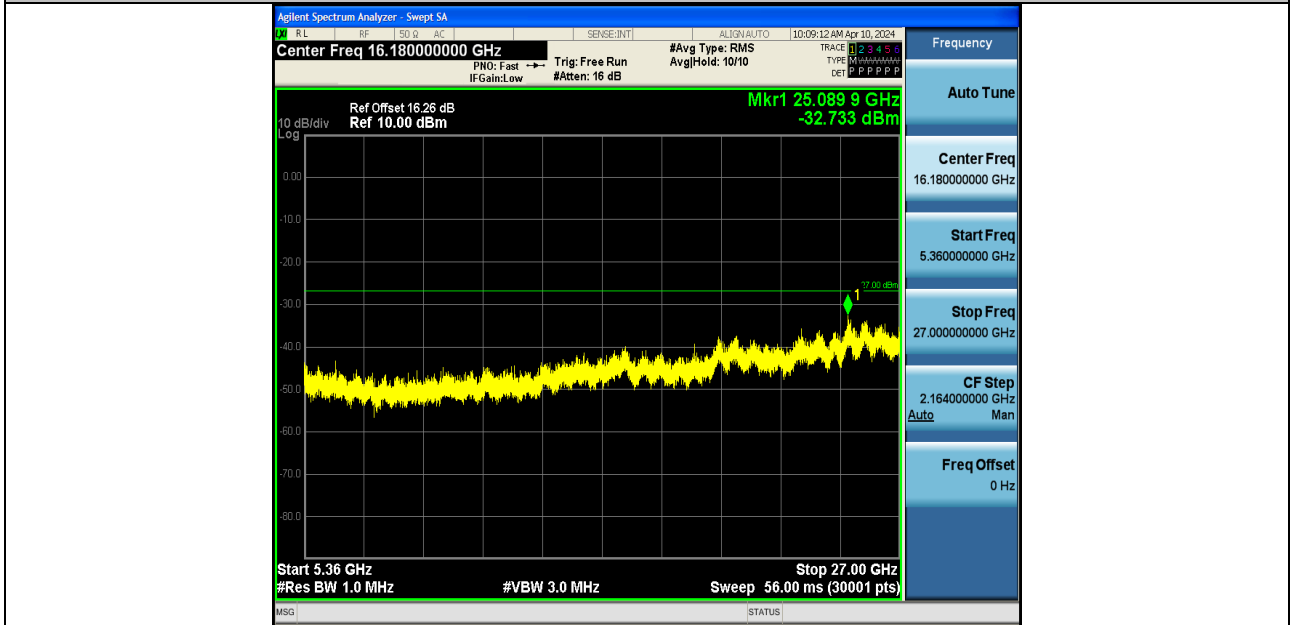
11AC40SISO-Ant2-5190-5360~27000-PASS
