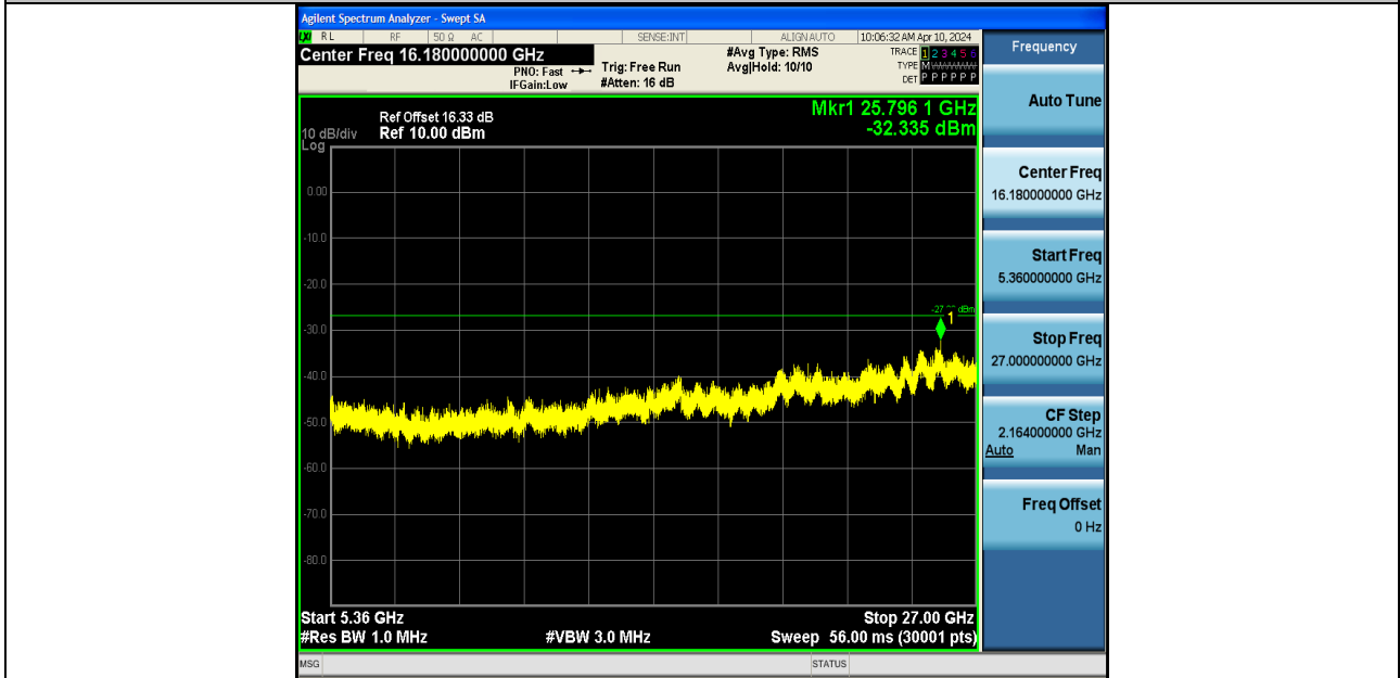
11AC40SISO-Ant1-5190-5360~27000-PASS
