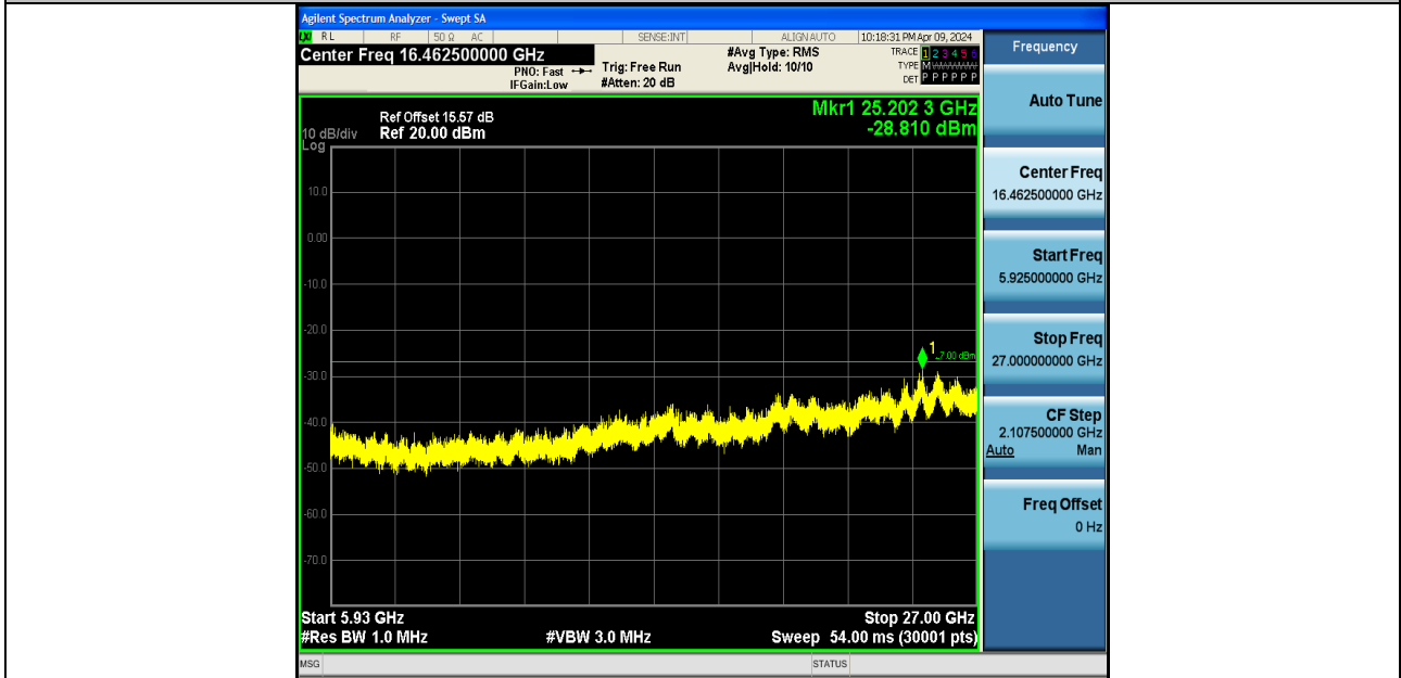
11AC20SISO-Ant2-5825-5925~27000-PASS
