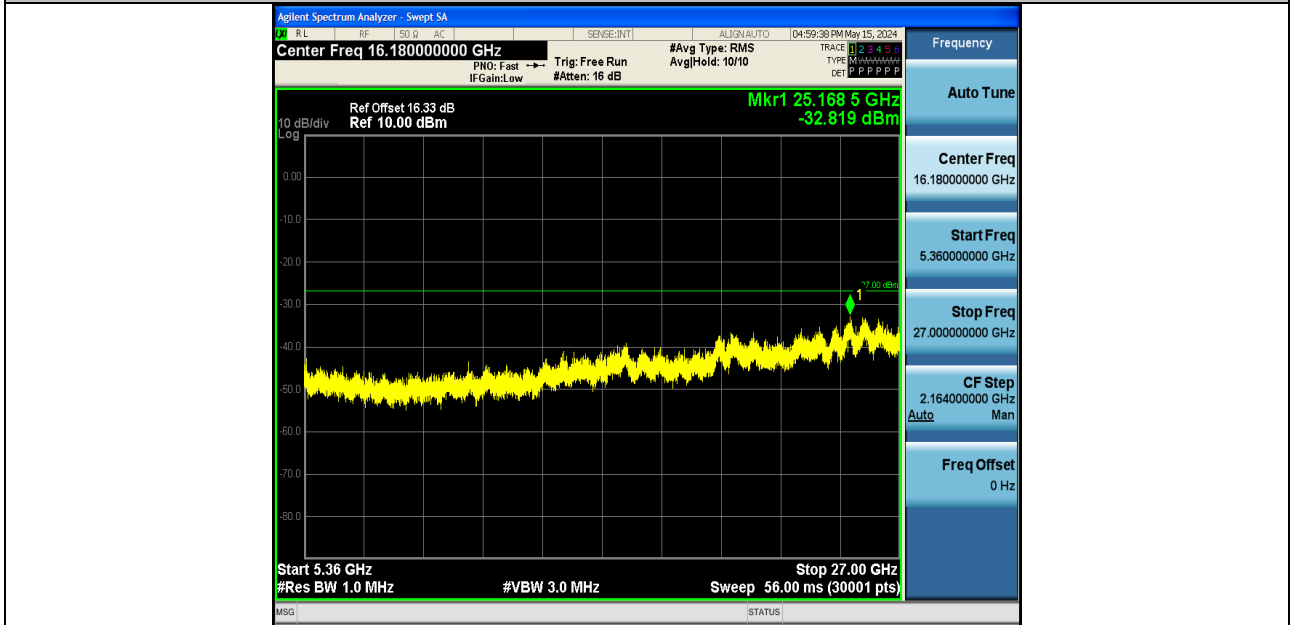
11AX40SISO-Ant1-5190-5360~27000-PASS
