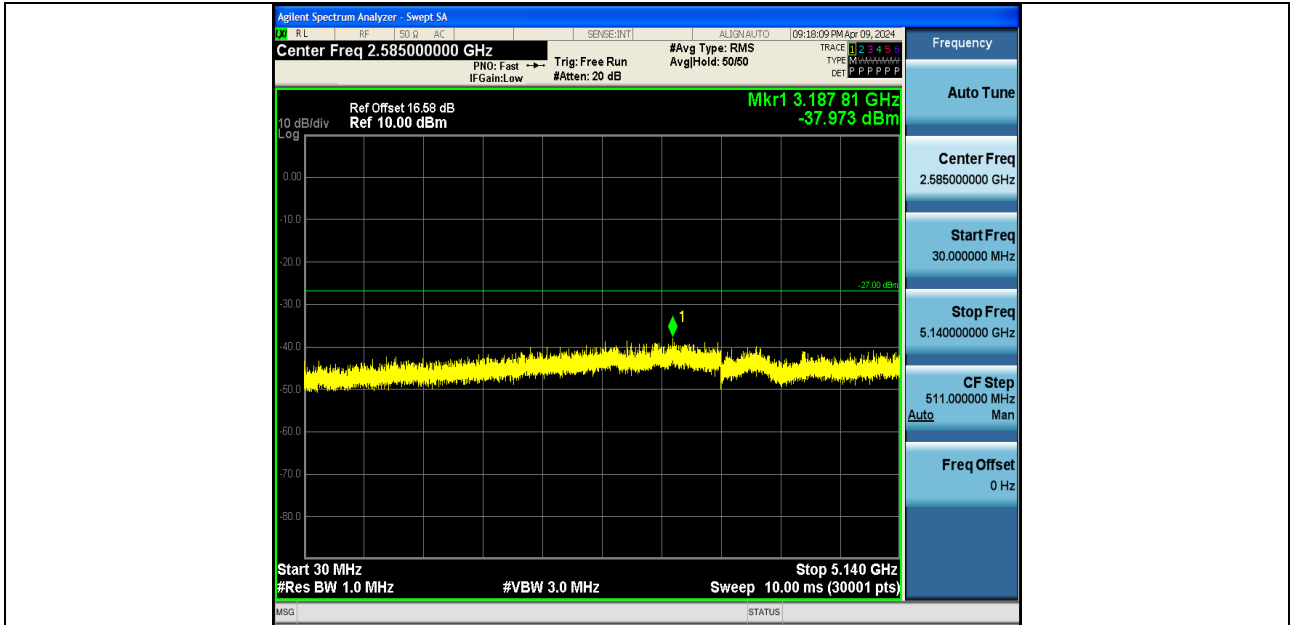
11N20SISO-Ant1-5240-30~5140-PASS
