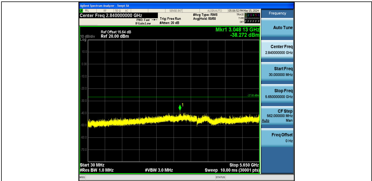
11AX40SISO-Ant1-5795-30~5650-PASS
