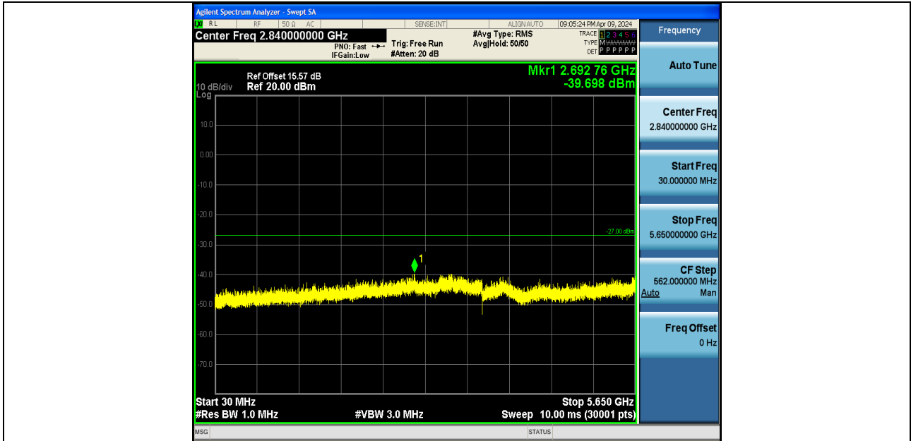
11A-Ant2-5825-30~5650-PASS
