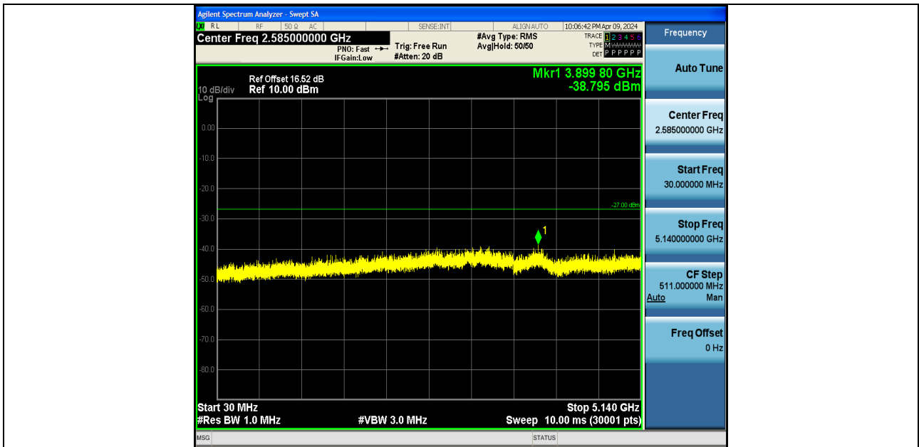
11AC20SISO-Ant2-5240-30~5140-PASS
