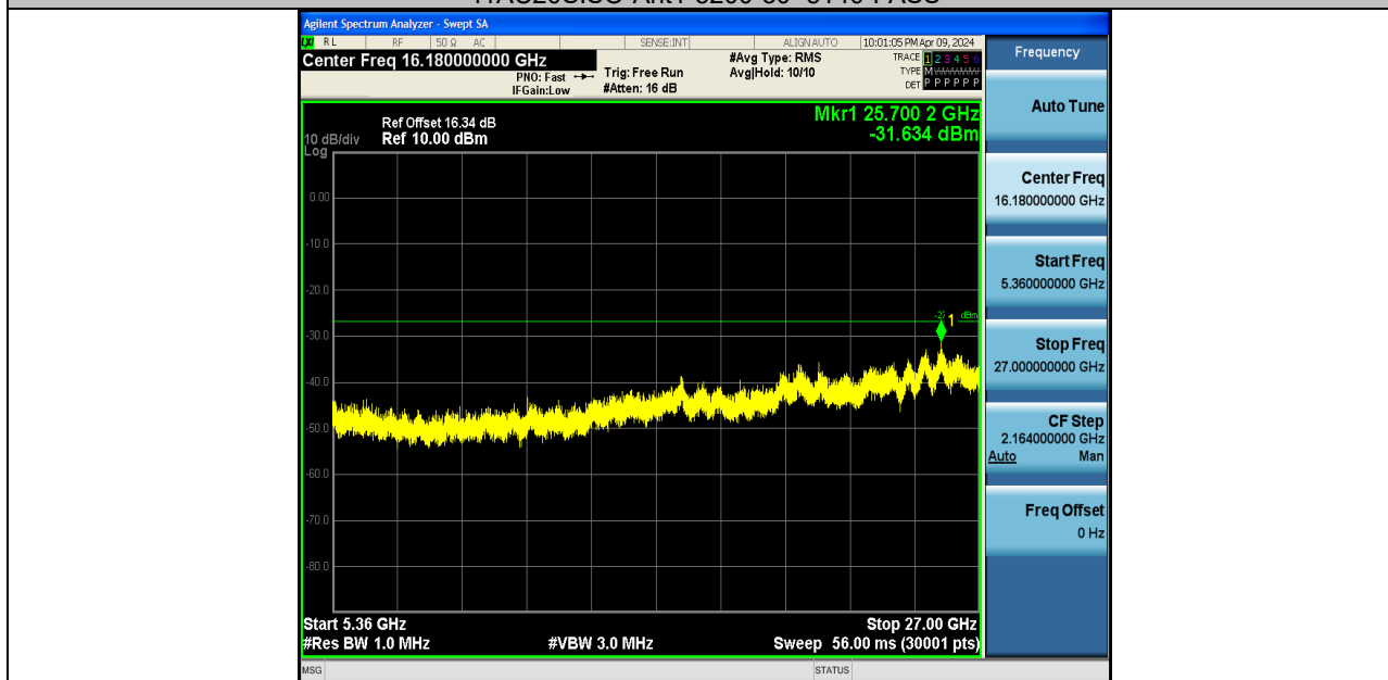
11AC20SISO-Ant1-5200-5360~27000-PASS
