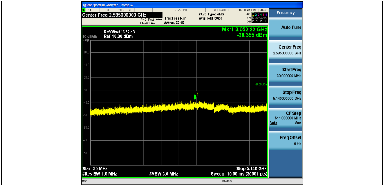
11AX40SISO-Ant2-5230-30~5140-PASS
