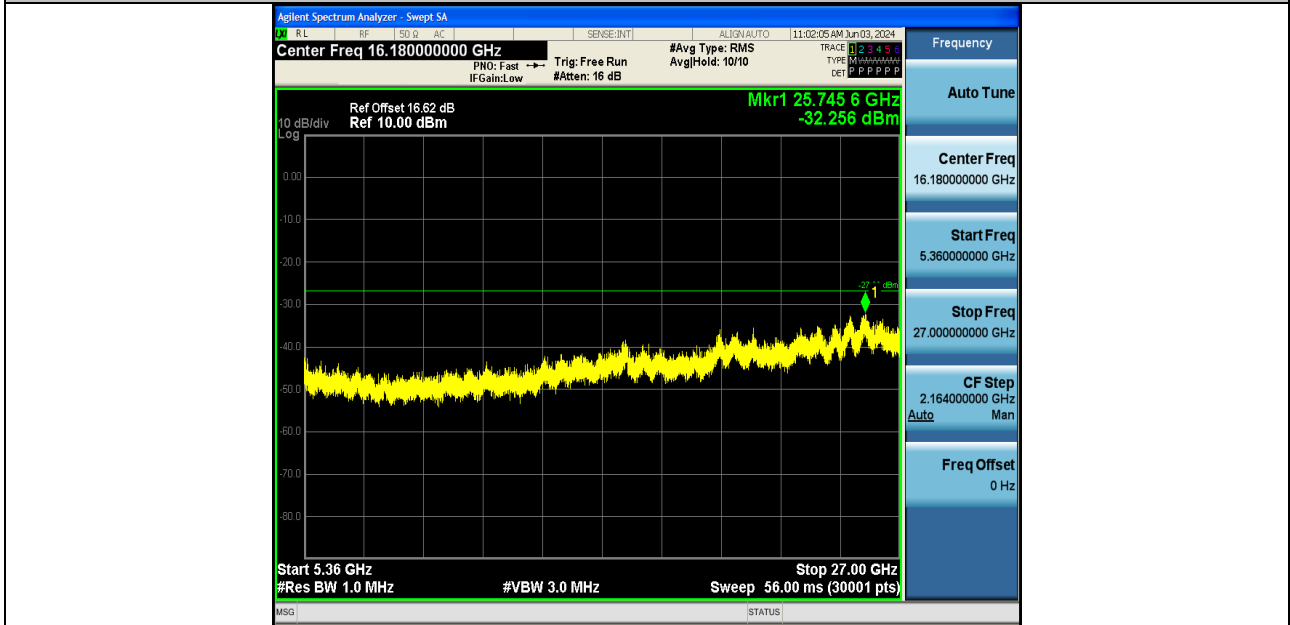
11AX40SISO-Ant2-5230-5360~27000-PASS
