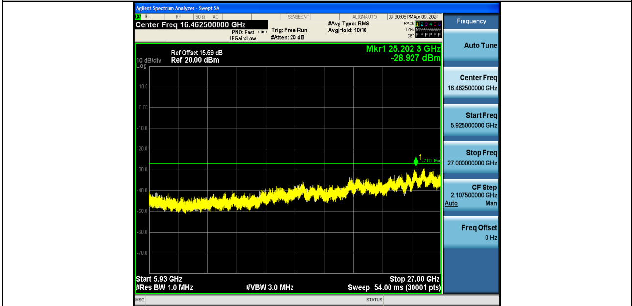
11N20SISO-Ant1-5825-5925~27000-PASS
