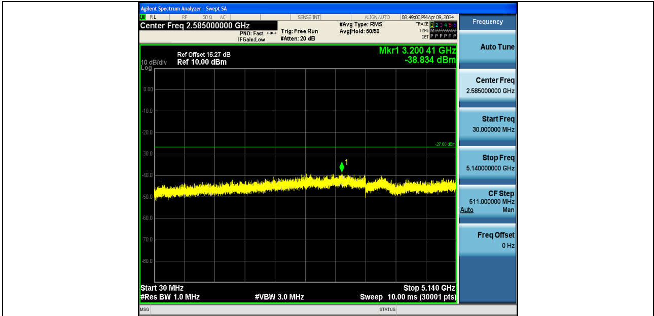
11A-Ant2-5200-30~5140-PASS
