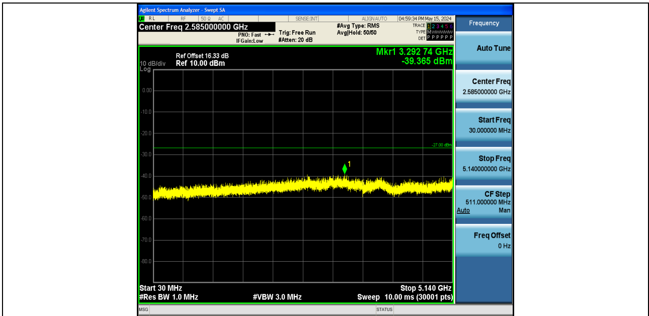
11AX40SISO-Ant1-5190-30~5140-PASS
