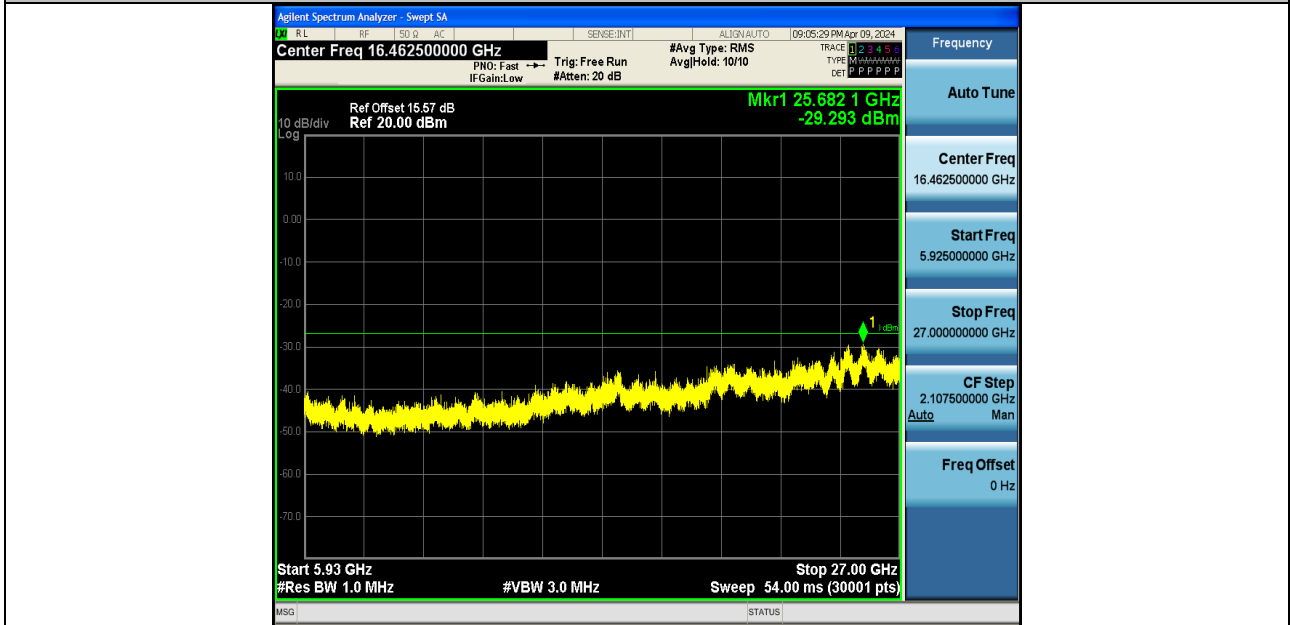
11A-Ant2-5825-5925~27000-PASS
