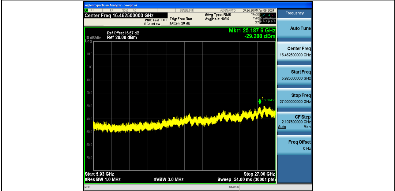
11N20SISO-Ant1-5785-5925~27000-PASS
