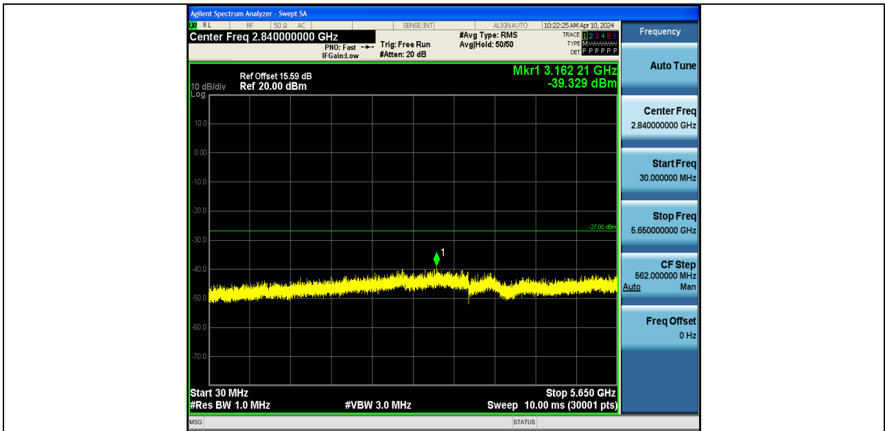
11AC40SISO-Ant2-5795-30~5650-PASS
