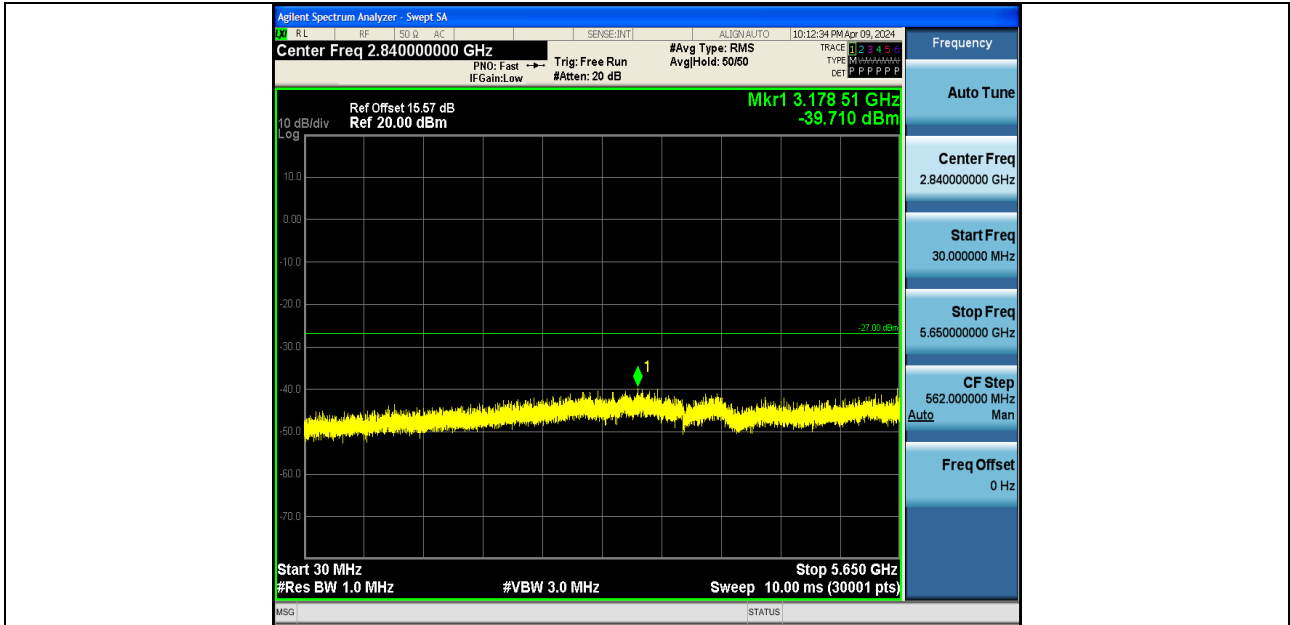
11AC20SISO-Ant1-5785-30~5650-PASS
