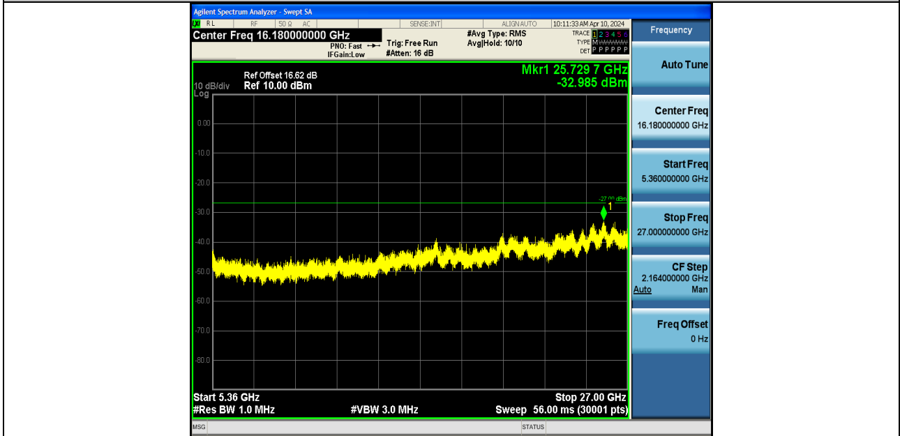
11AC40SISO-Ant1-5230-5360~27000-PASS
