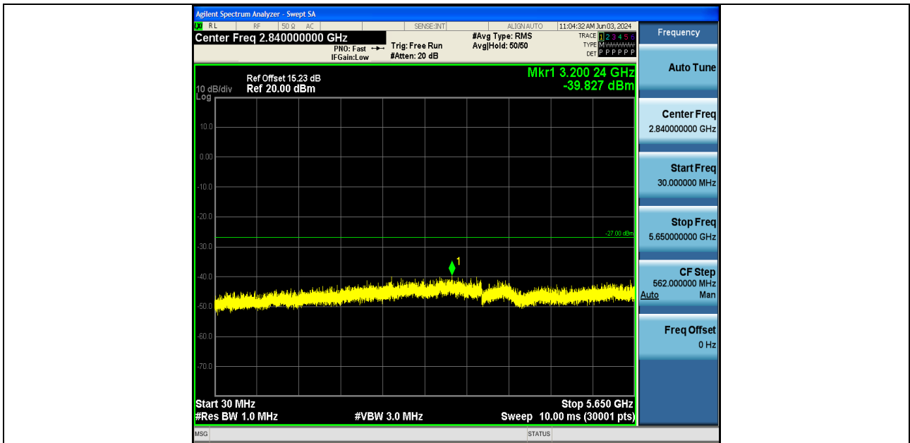
11AX40SISO-Ant2-5755-30~5650-PASS
