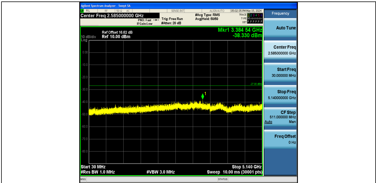
11AX40SISO-Ant1-5230-30~5140-PASS
