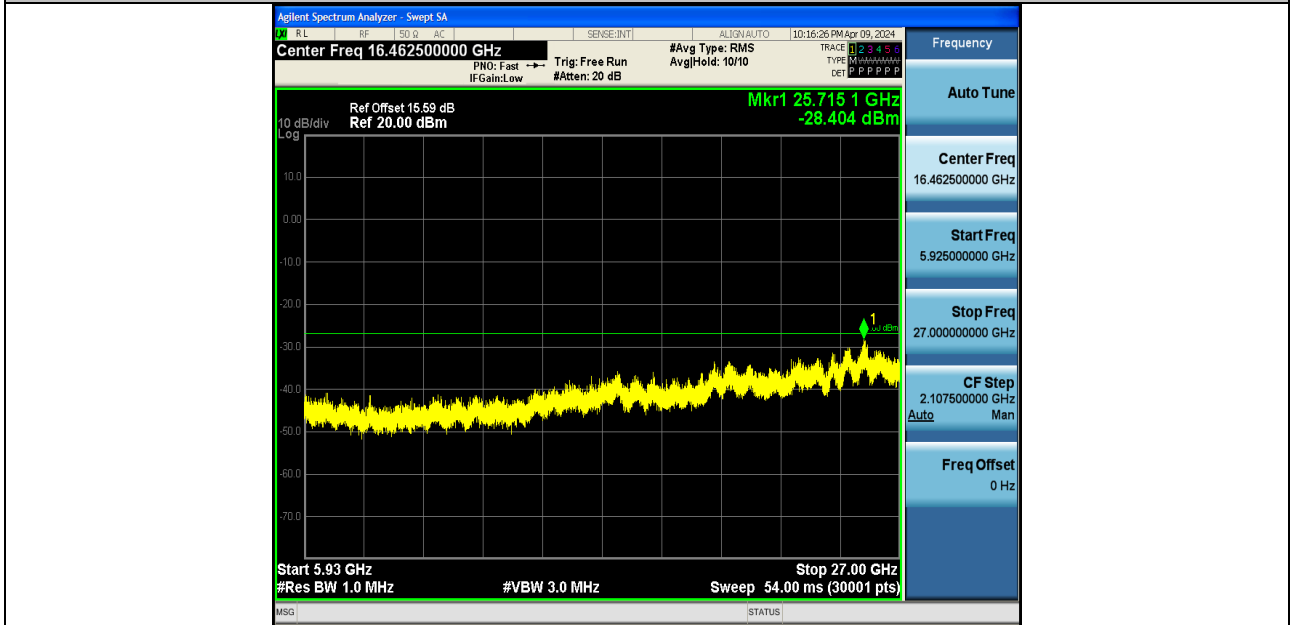
11AC20SISO-Ant1-5825-5925~27000-PASS
