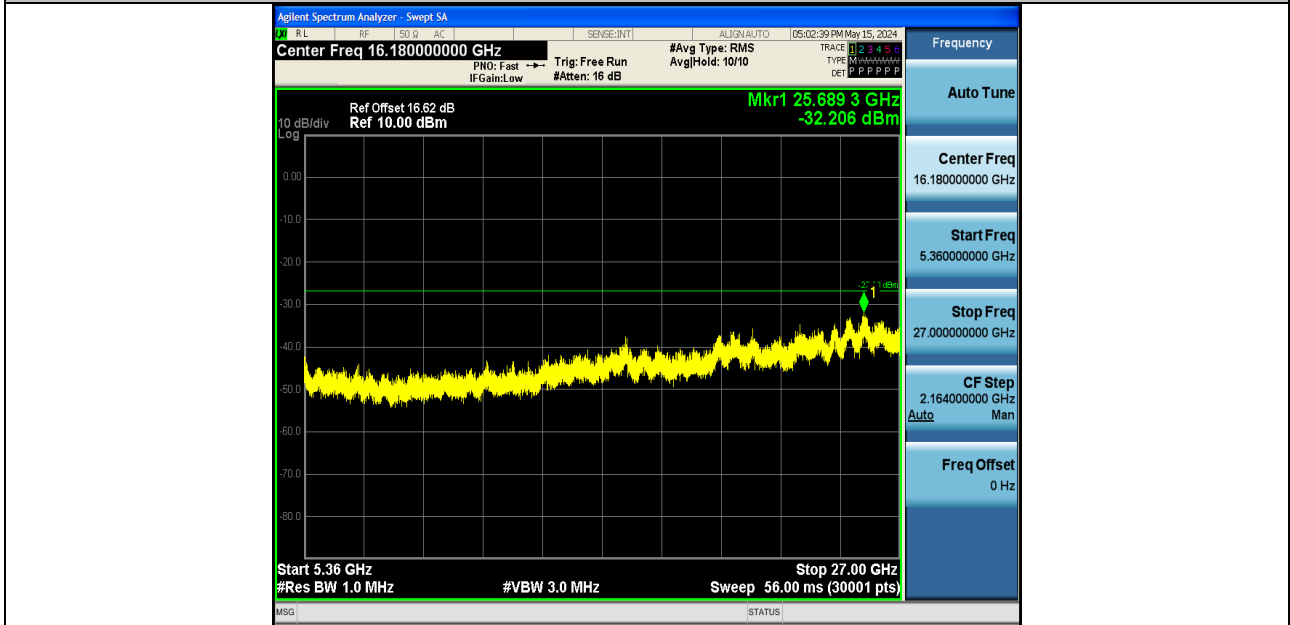
11AX40SISO-Ant1-5230-5360~27000-PASS
