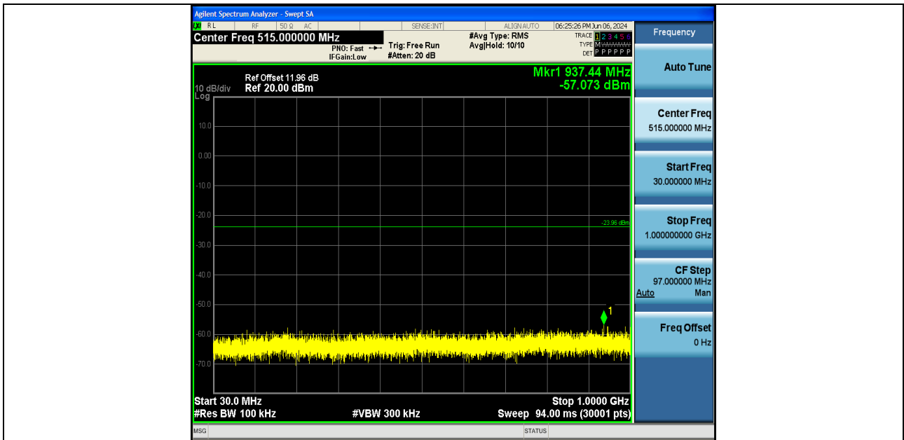
11AX40SISO-Ant2-2452-30~1000-PASS
