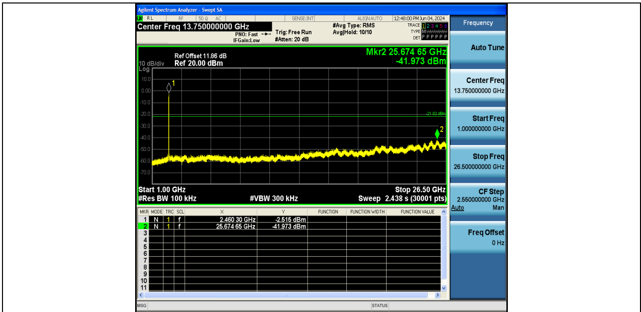
11AX20SISO-Ant1-2462-1000~26500-PASS
