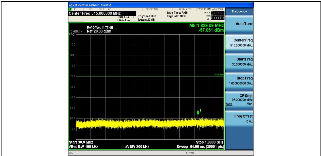
11AX20SISO-Ant2-2437-30~1000-PASS
