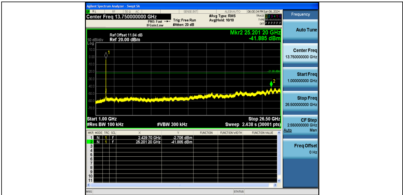
11AX40SISO-Ant1-2422-1000~26500-PASS
