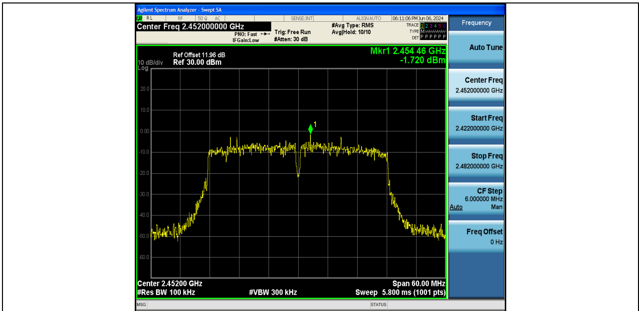
11AX40SISO-Ant1-2452-0~Reference-PASS
