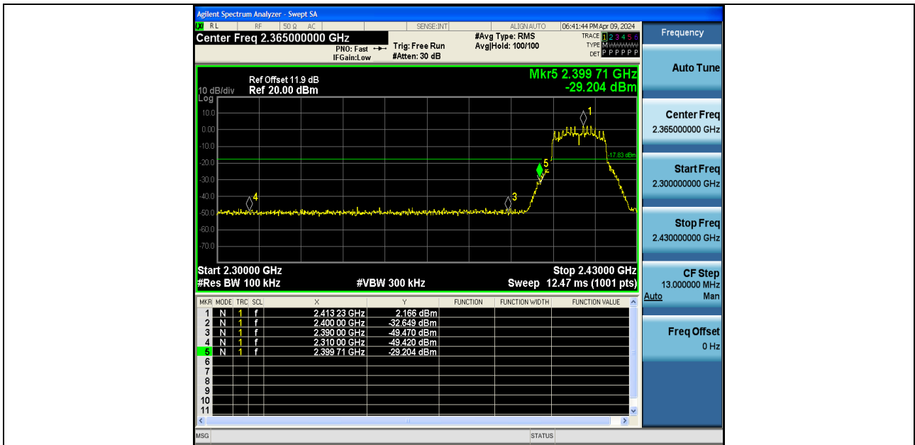
11G-Ant2-2412-PASS
