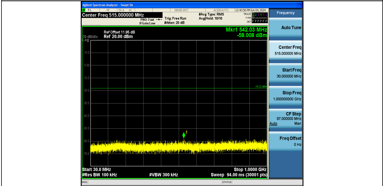
11AX20SISO-Ant1-2412-30~1000-PASS
