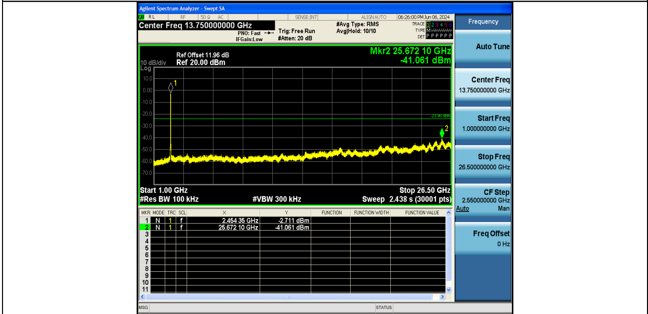
11AX40SISO-Ant2-2452-1000~26500-PASS
