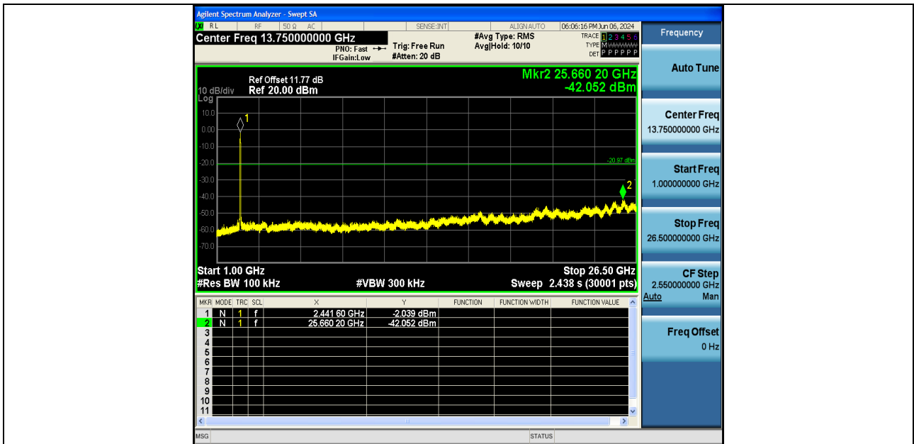
11AX40SISO-Ant1-2437-1000~26500-PASS
