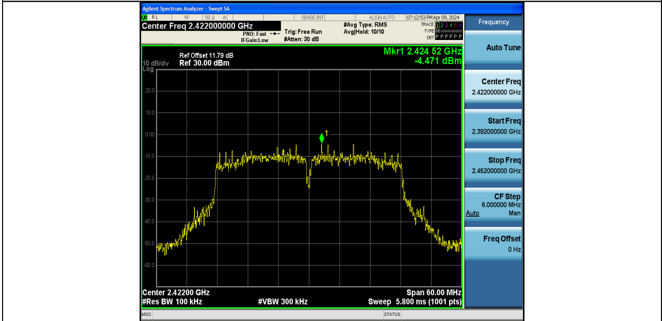
11N40SISO-Ant2-2422-0~Reference-PASS
