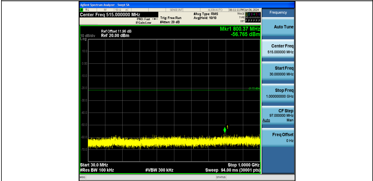
11AX40SISO-Ant1-2452-30~1000-PASS
