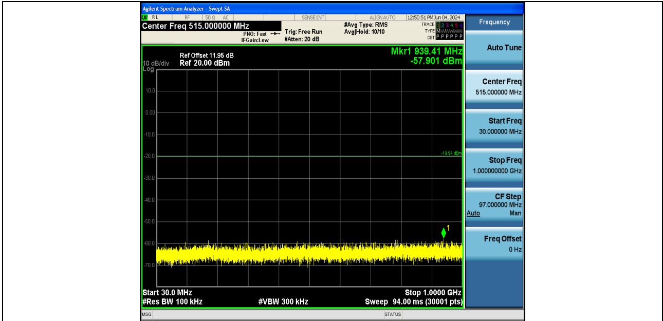
11AX20SISO-Ant2-2412-30~1000-PASS
