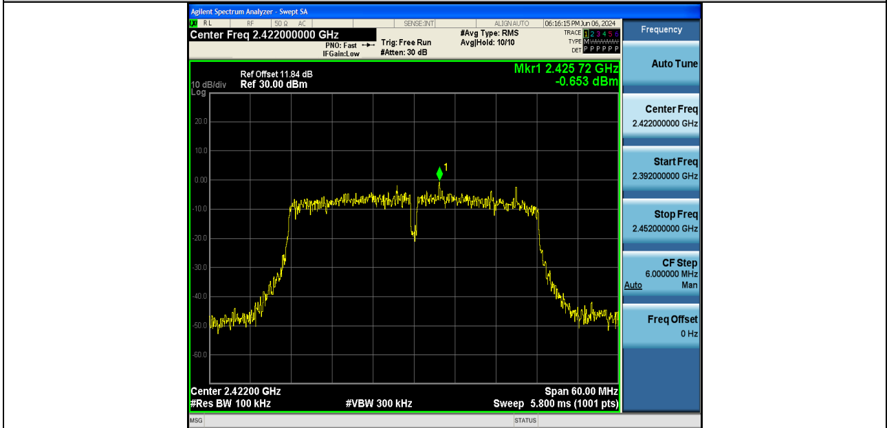
11AX40SISO-Ant2-2422-0~Reference-PASS
