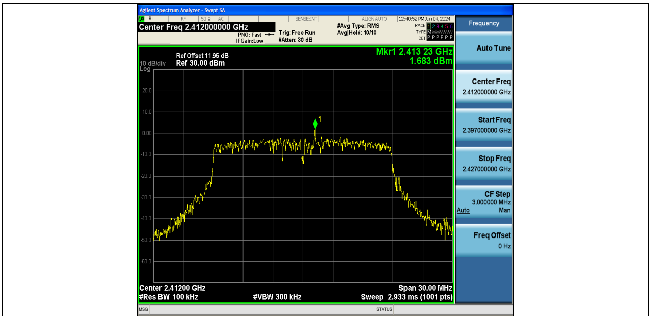
11AX20SISO-Ant1-2412-0~Reference-PASS
