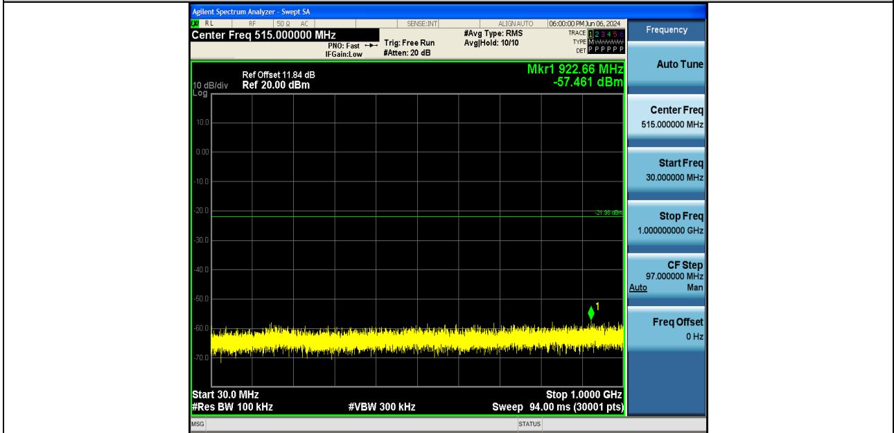
11AX40SISO-Ant1-2422-30~1000-PASS
