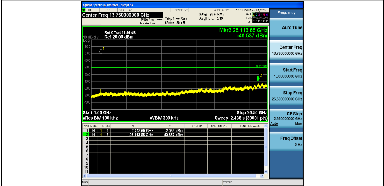
11AX20SISO-Ant2-2412-1000~26500-PASS
