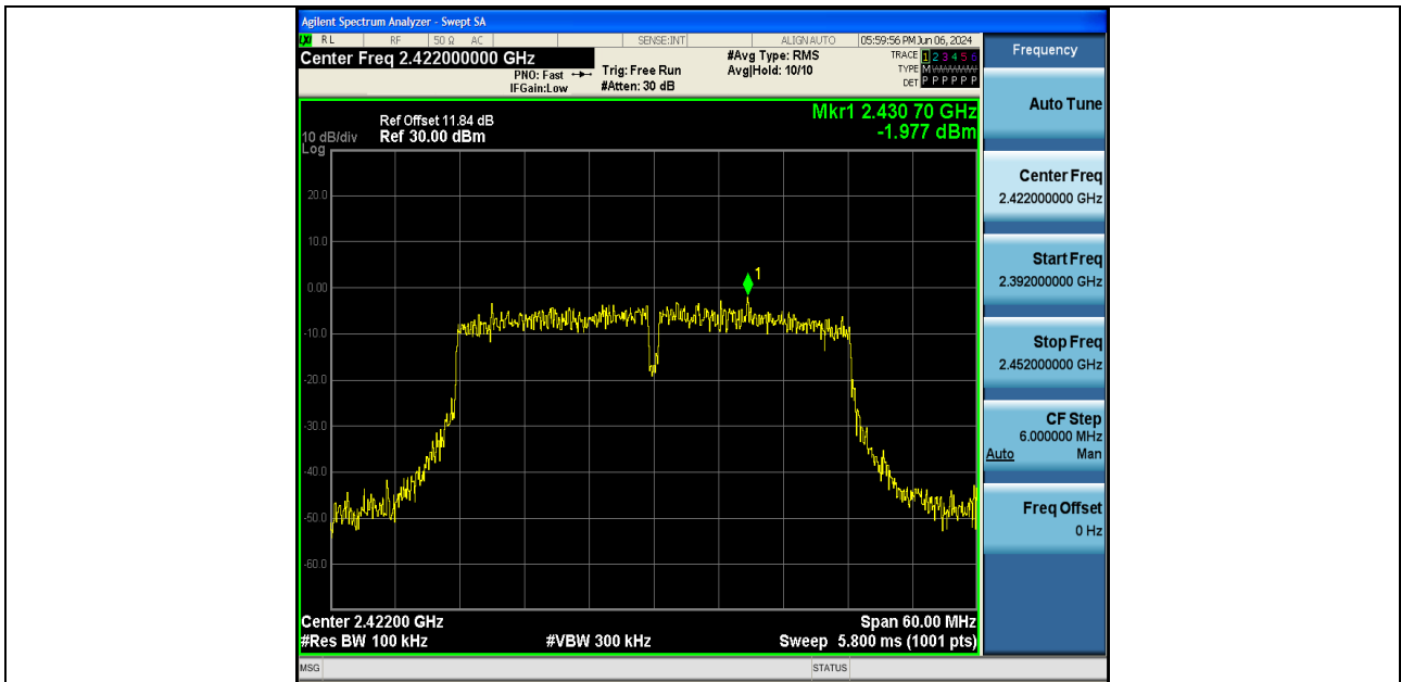
11AX40SISO-Ant1-2422-0~Reference-PASS
