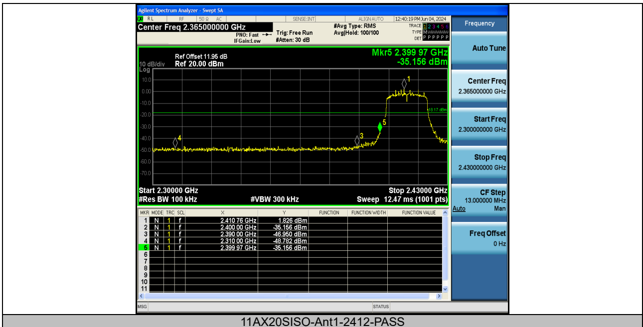
11AX20SISO-Ant1-2412-PASS
