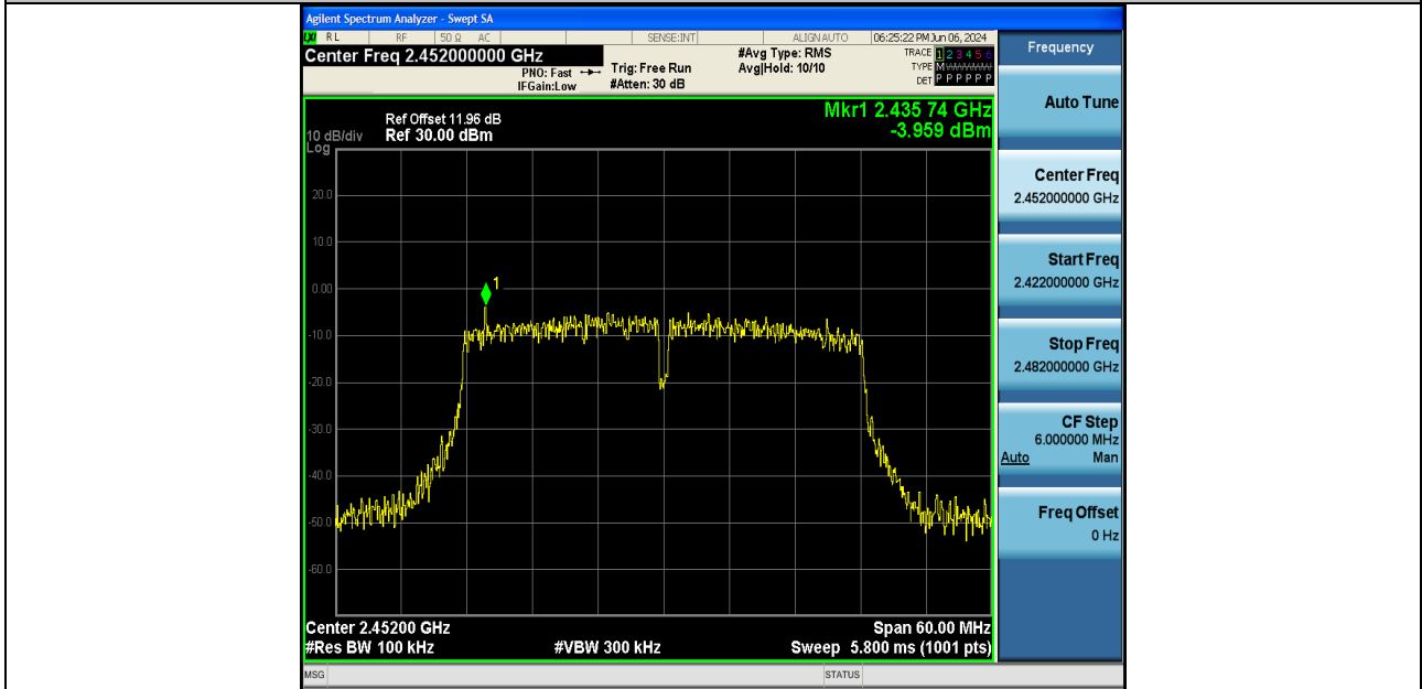
11AX40SISO-Ant2-2452-0~Reference-PASS
