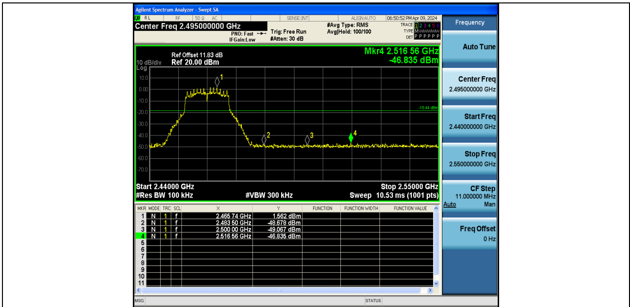
11G-Ant2-2462-PASS
