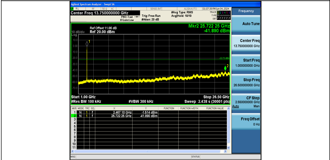
11AX20SISO-Ant2-2462-1000~26500-PASS
