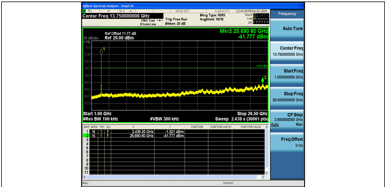
11AX20SISO-Ant1-2437-1000~26500-PASS
