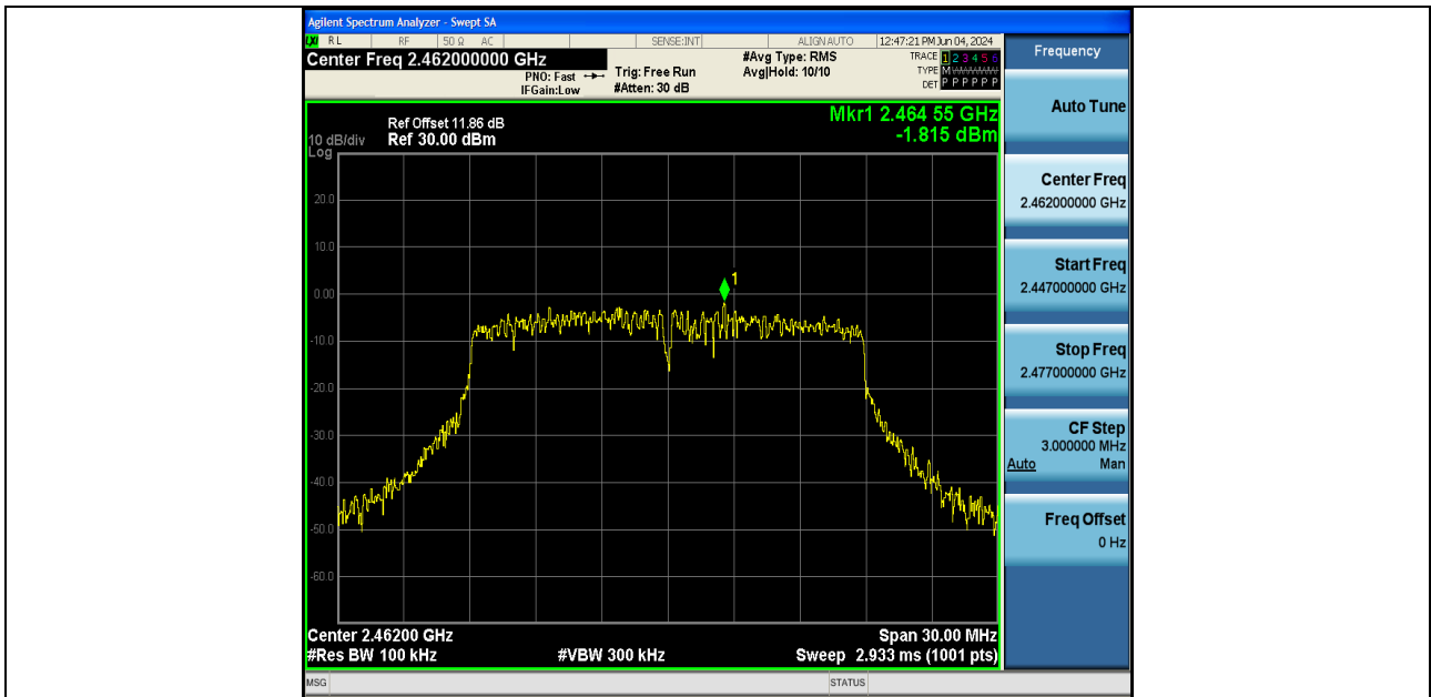
11AX20SISO-Ant1-2462-0~Reference-PASS
