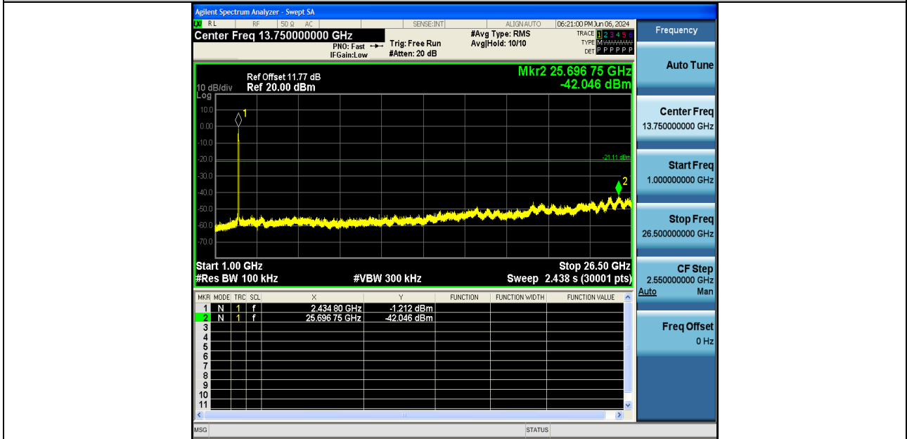
11AX40SISO-Ant2-2437-1000~26500-PASS
