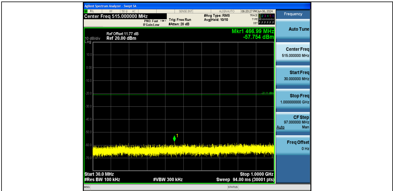
11AX40SISO-Ant2-2437-30~1000-PASS
