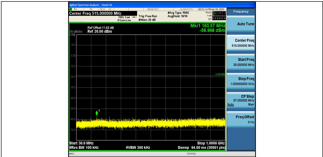
11G-Ant2-2462-30~1000-PASS
