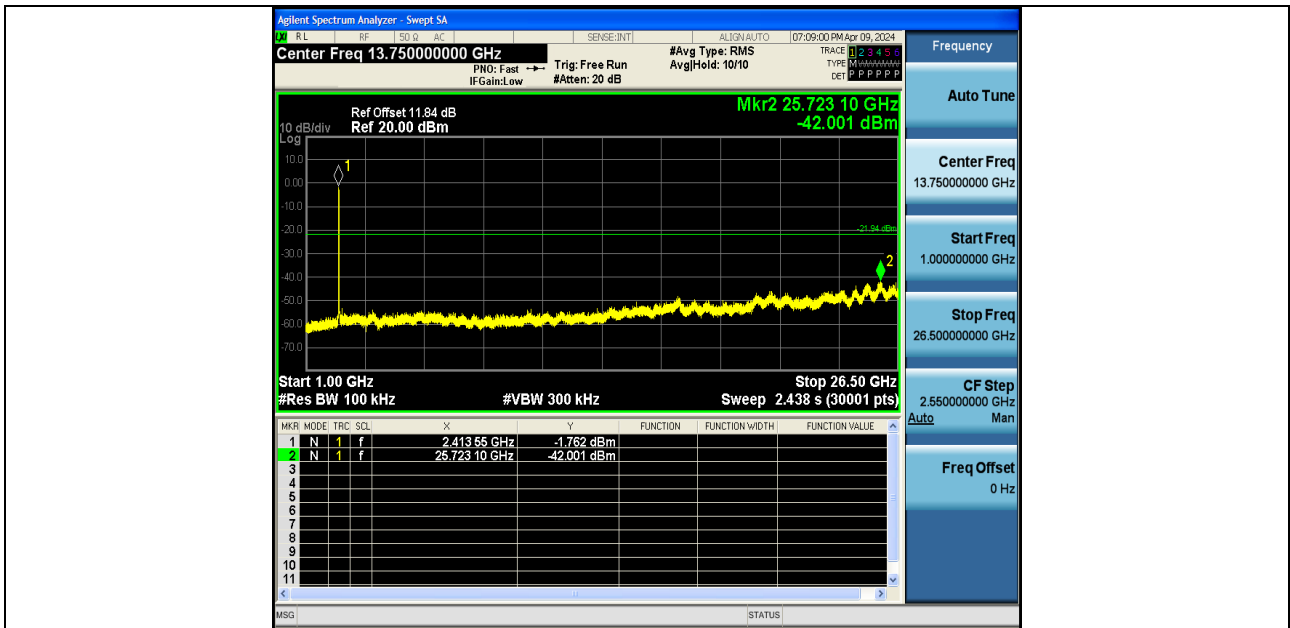
11N40SISO-Ant1-2422-1000~26500-PASS
