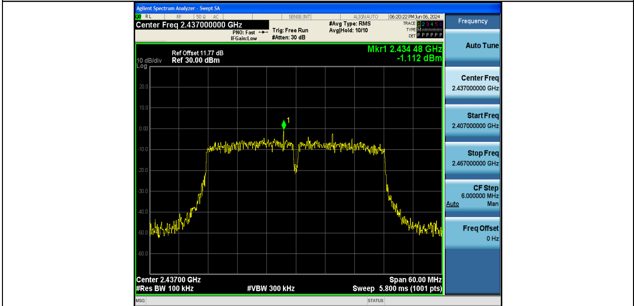
11AX40SISO-Ant2-2437-0~Reference-PASS
