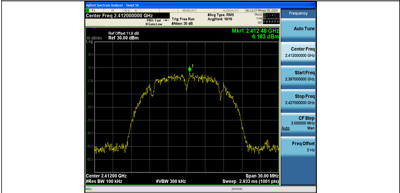
11B-Ant2-2412-0~Reference-PASS
