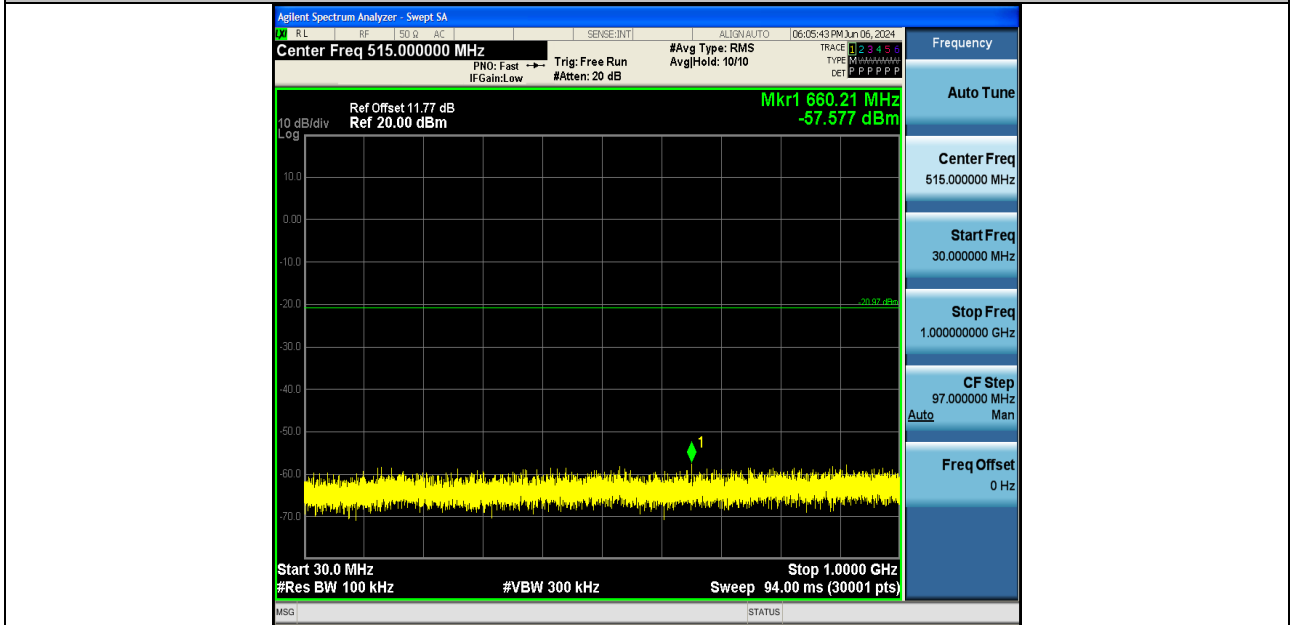
11AX40SISO-Ant1-2437-30~1000-PASS
