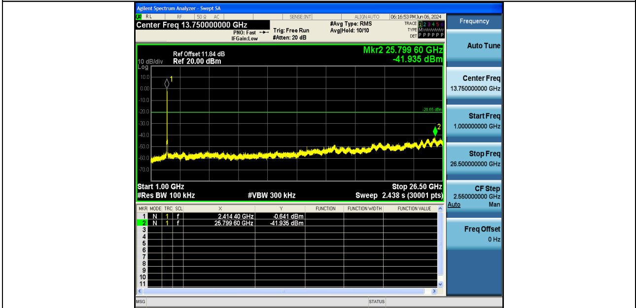
11AX40SISO-Ant2-2422-1000~26500-PASS
