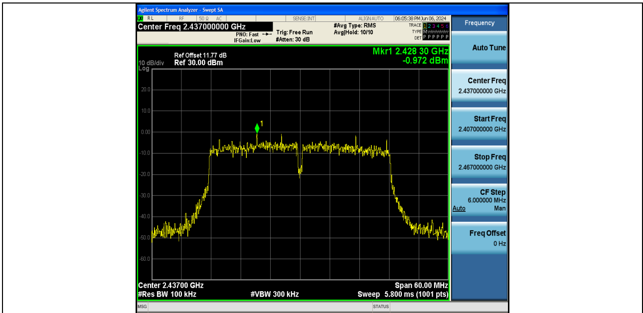
11AX40SISO-Ant1-2437-0~Reference-PASS
