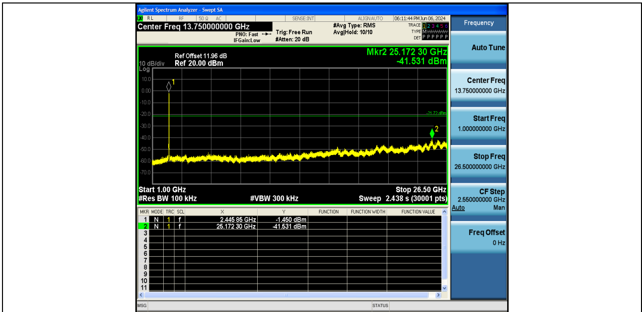
11AX40SISO-Ant1-2452-1000~26500-PASS
