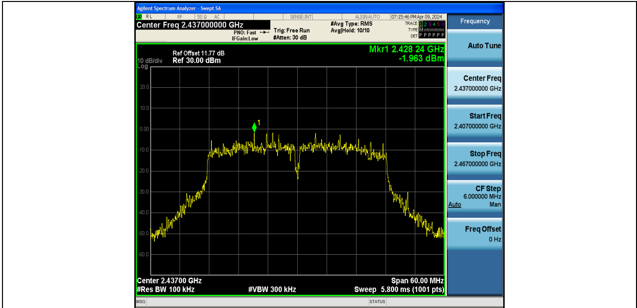
11N40SISO-Ant1-2437-0~Reference-PASS
