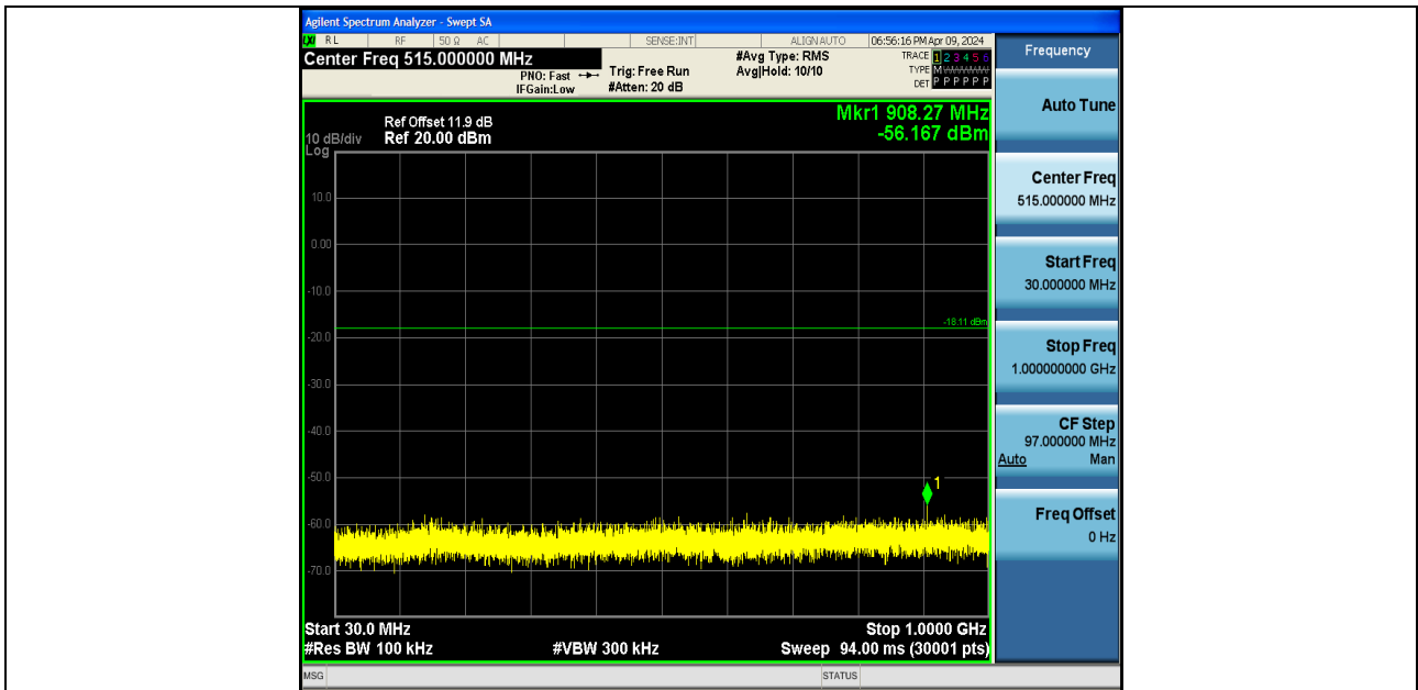
11N20SISO-Ant2-2412-30~1000-PASS
