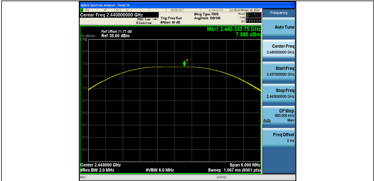
BLE_2M-Ant1-2440-PASS
