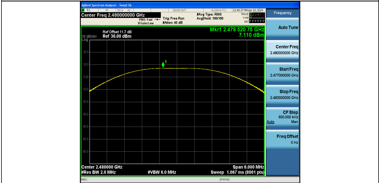
BLE_2M-Ant1-2480-PASS
