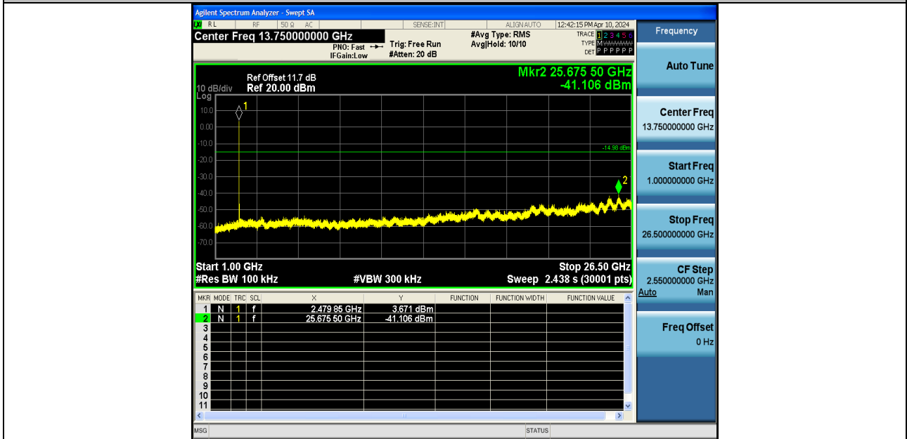
BLE_2M-Ant1-2480-1000~26500-PASS
