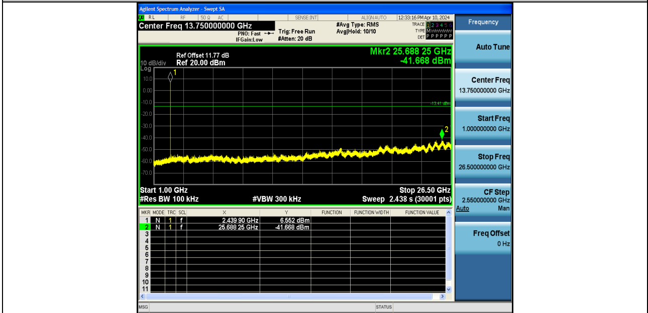
BLE_1M-Ant1-2440-1000~26500-PASS
