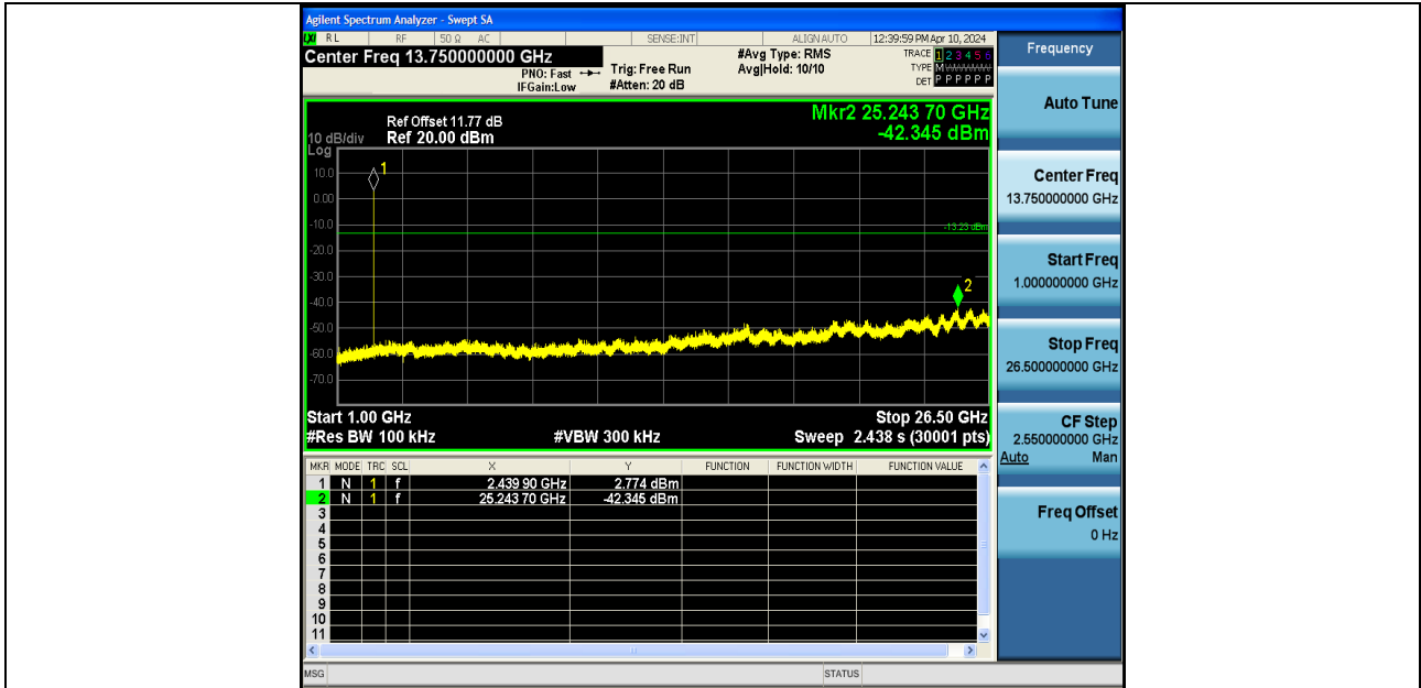
BLE_2M-Ant1-2440-1000~26500-PASS
