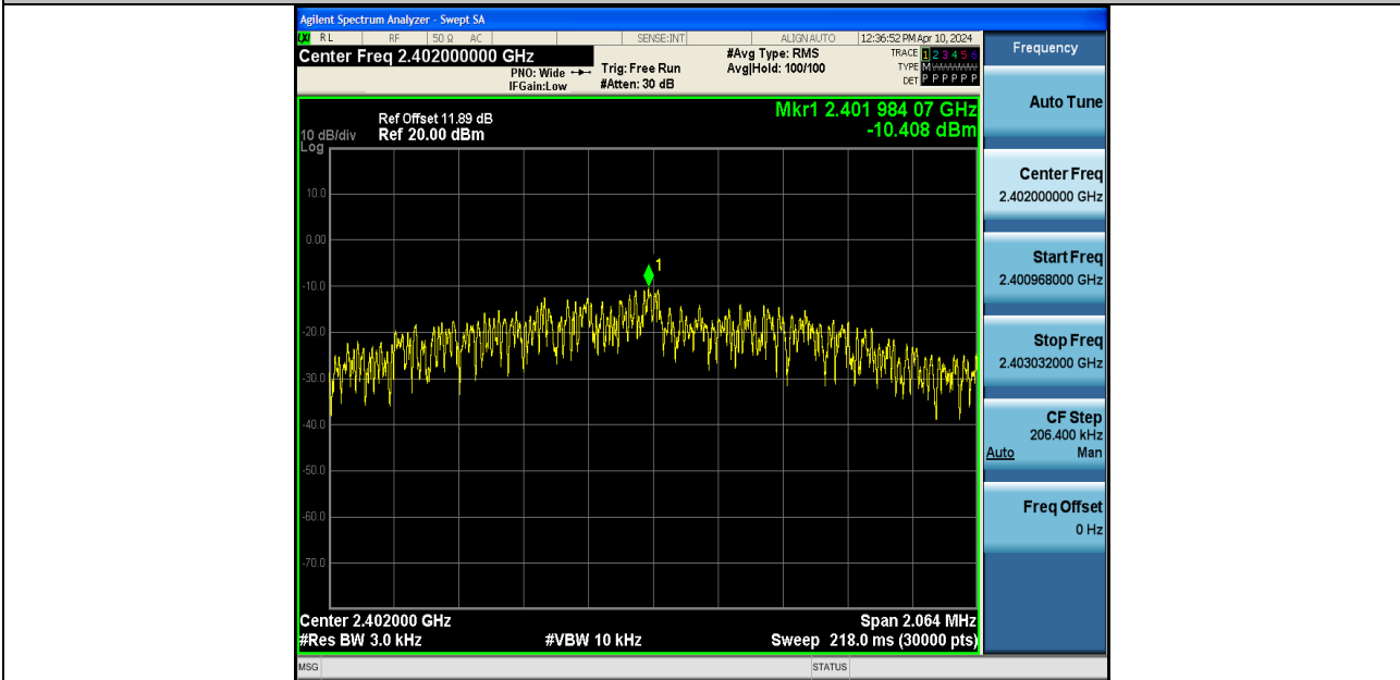
BLE_2M-Ant1-2402-PASS
