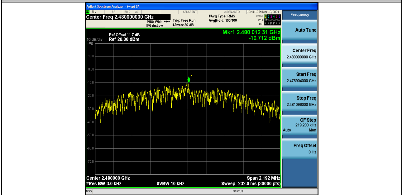
BLE_2M-Ant1-2480-PASS
