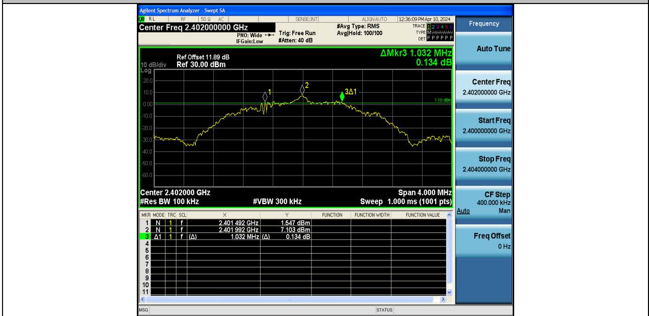
BLE_2M-Ant1-2402-PASS
