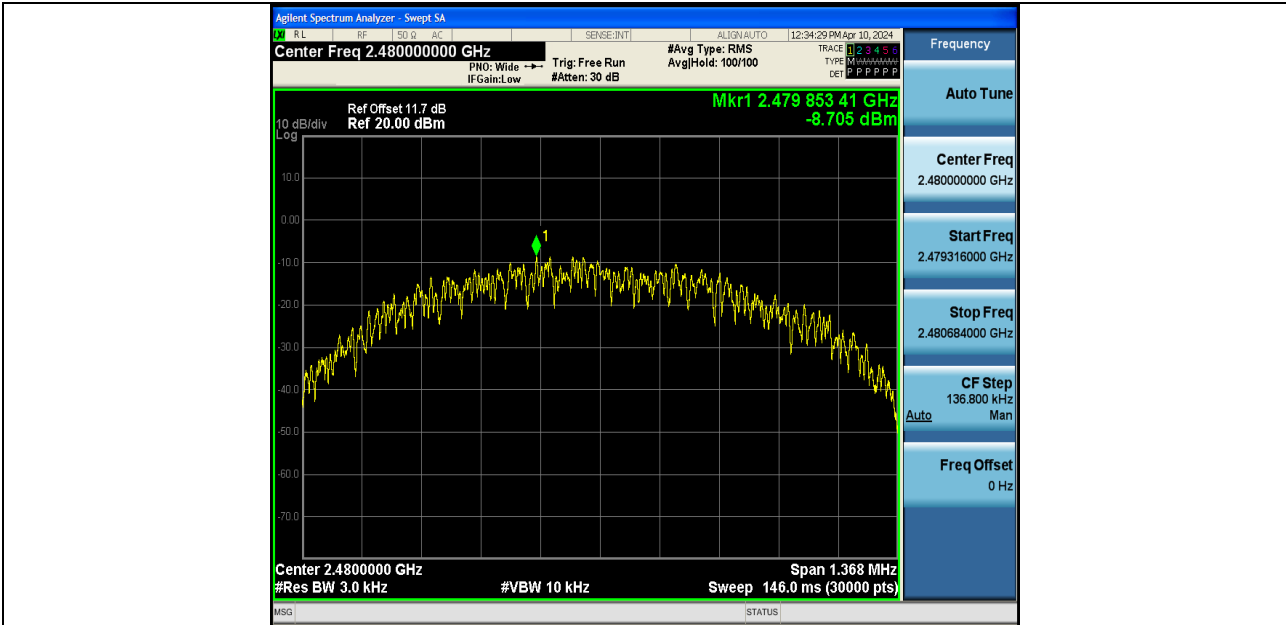
BLE_1M-Ant1-2480-PASS
