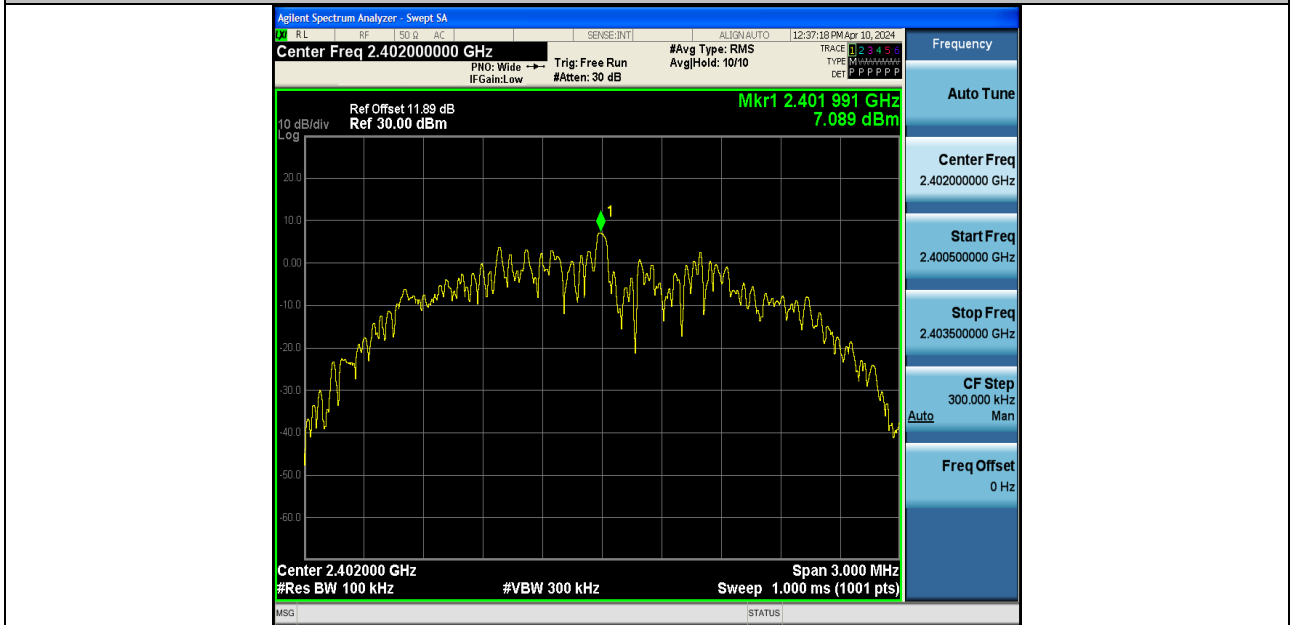
BLE_2M-Ant1-2402-0~Reference-PASS
