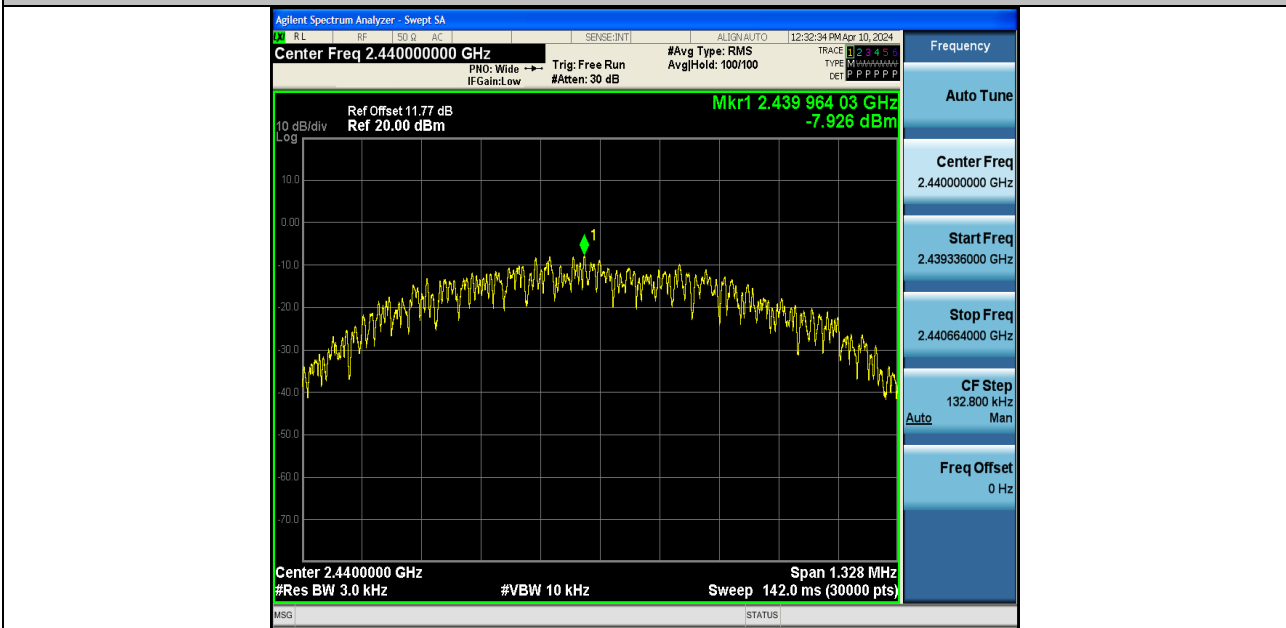
BLE_1M-Ant1-2440-PASS
