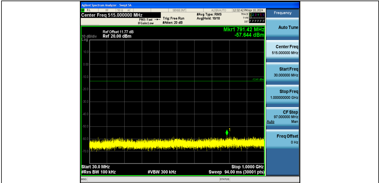
BLE_1M-Ant1-2440-30~1000-PASS
