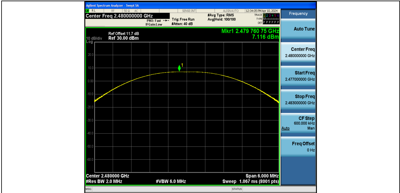
BLE_1M-Ant1-2480-PASS
