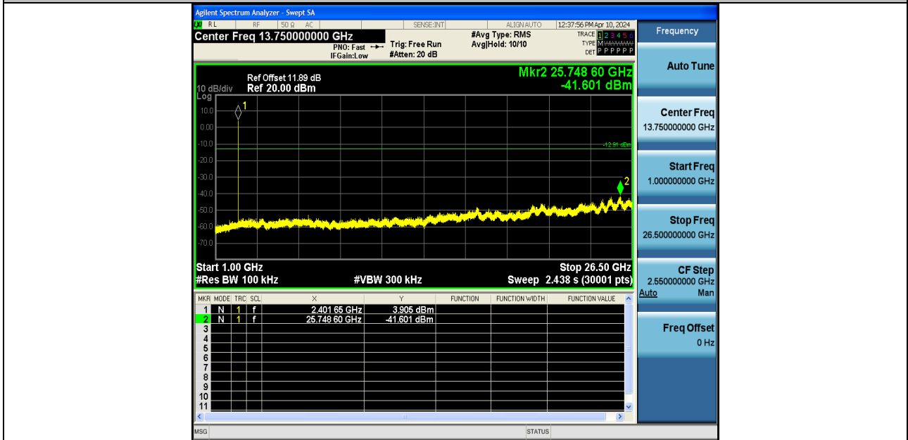
BLE_2M-Ant1-2402-1000~26500-PASS
