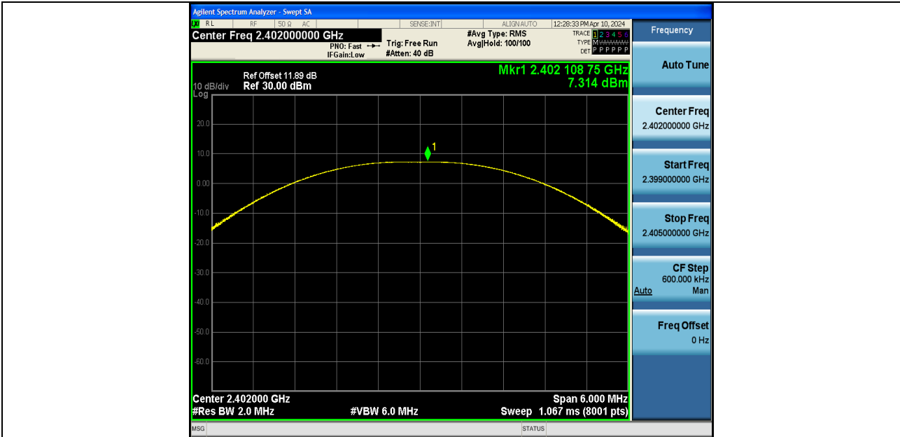
BLE_1M-Ant1-2402-PASS
