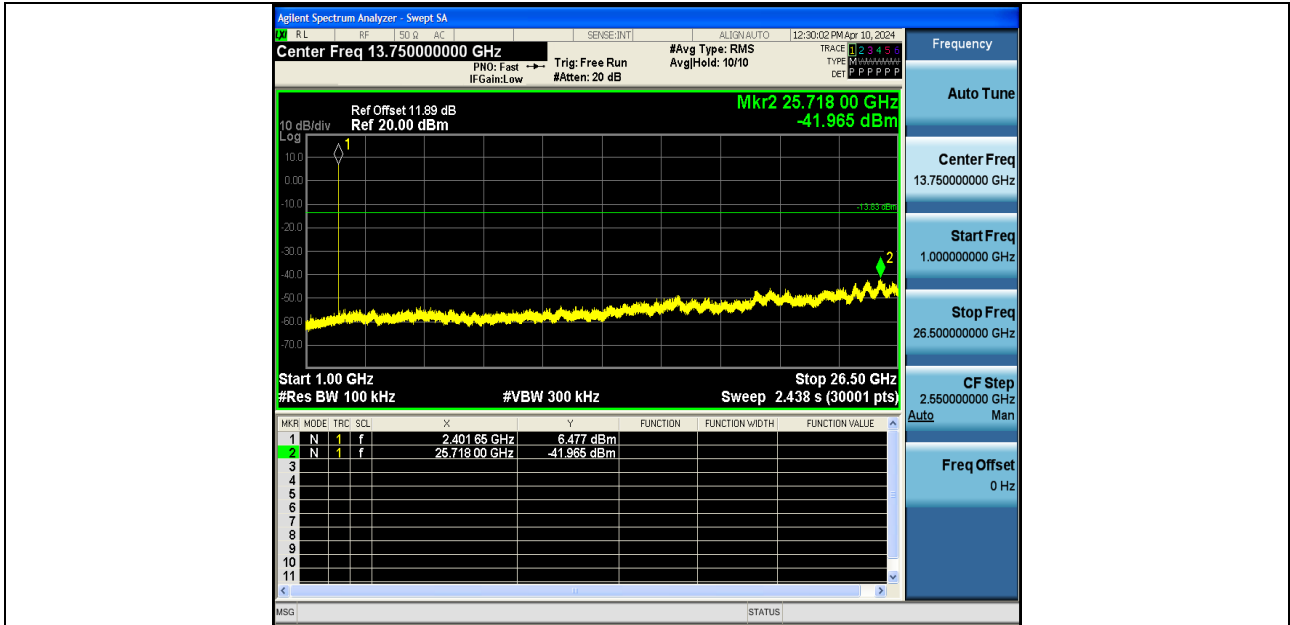
BLE_1M-Ant1-2402-1000~26500-PASS
