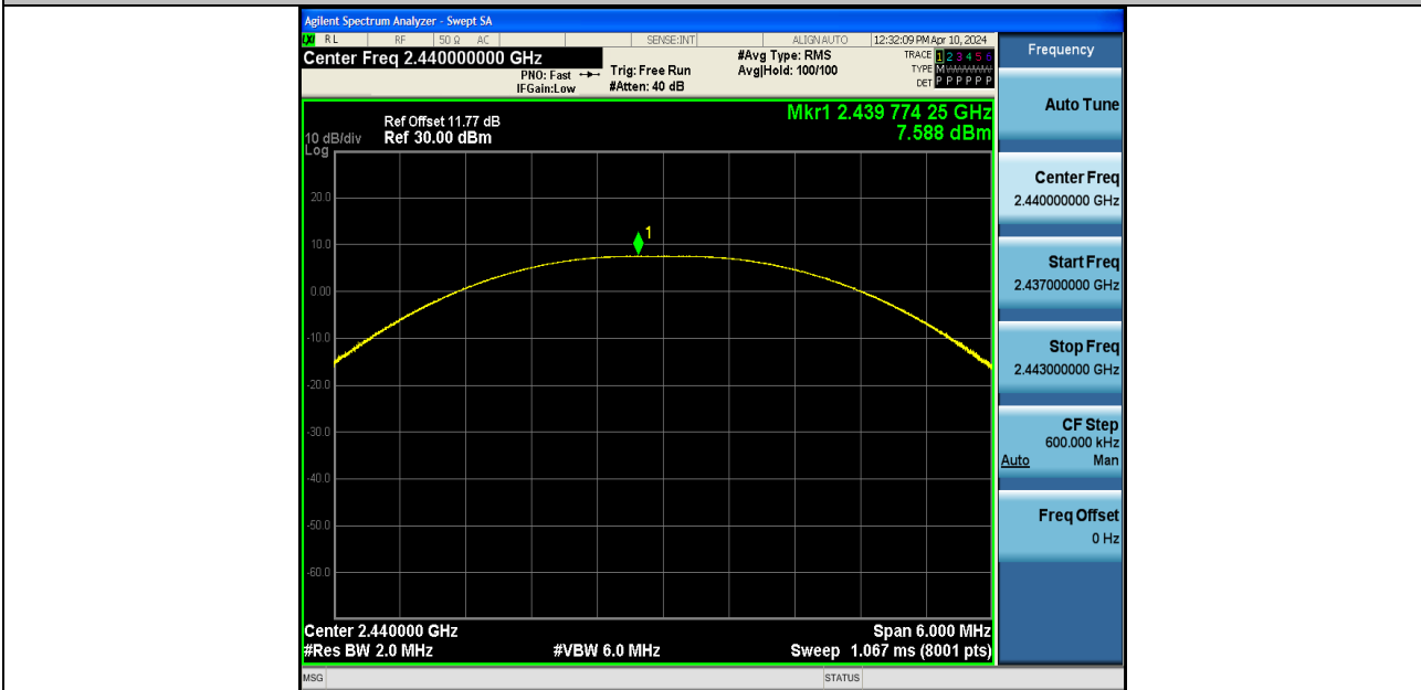
BLE_1M-Ant1-2440-PASS
