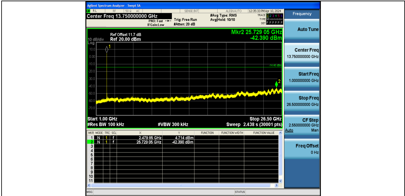
BLE_1M-Ant1-2480-1000~26500-PASS
