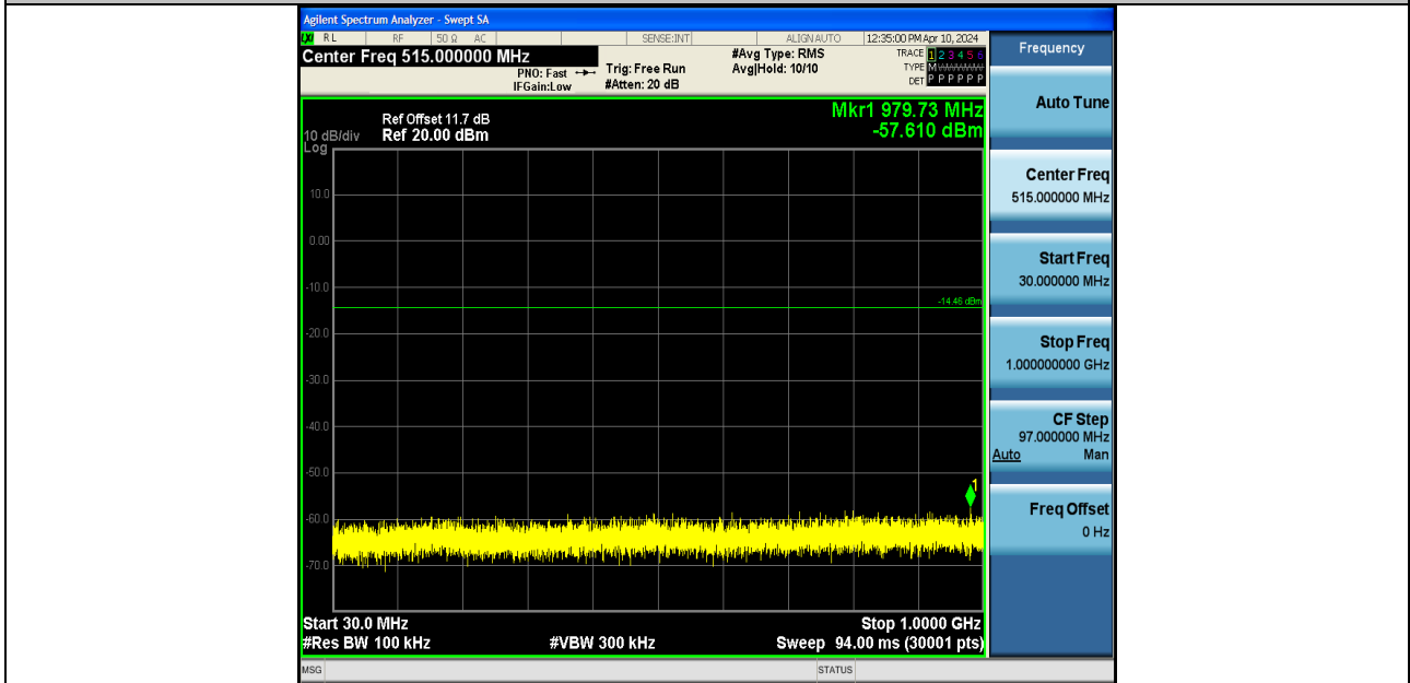
BLE_1M-Ant1-2480-30~1000-PASS
