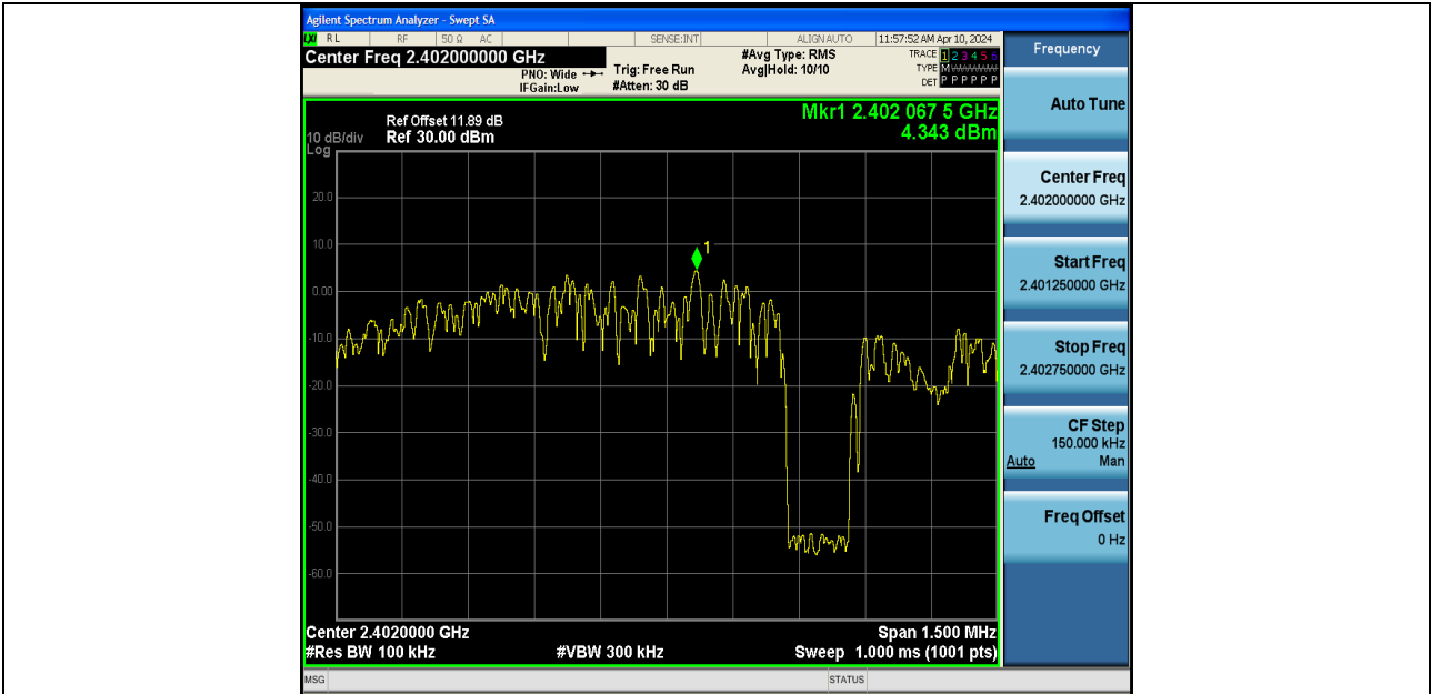
3DH5-Ant1-2402-0~Reference-PASS
