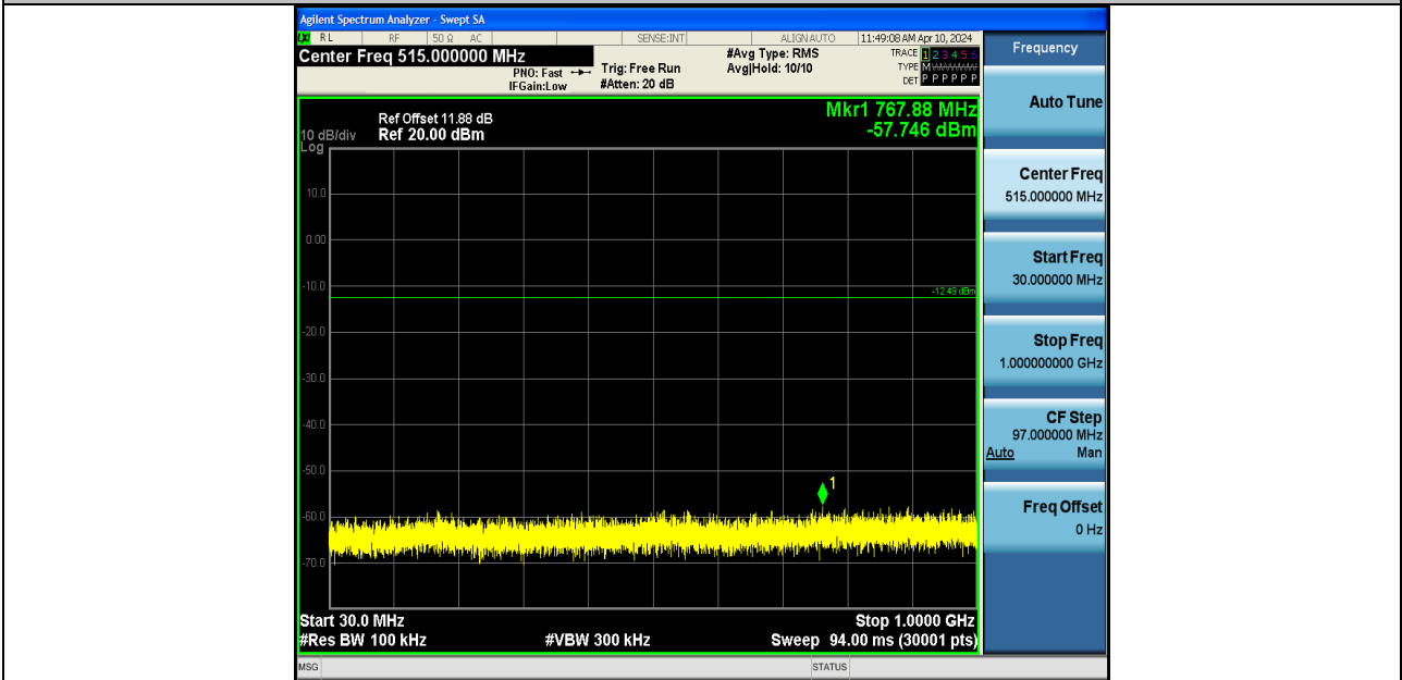
2DH5-Ant1-2441-30~1000-PASS
