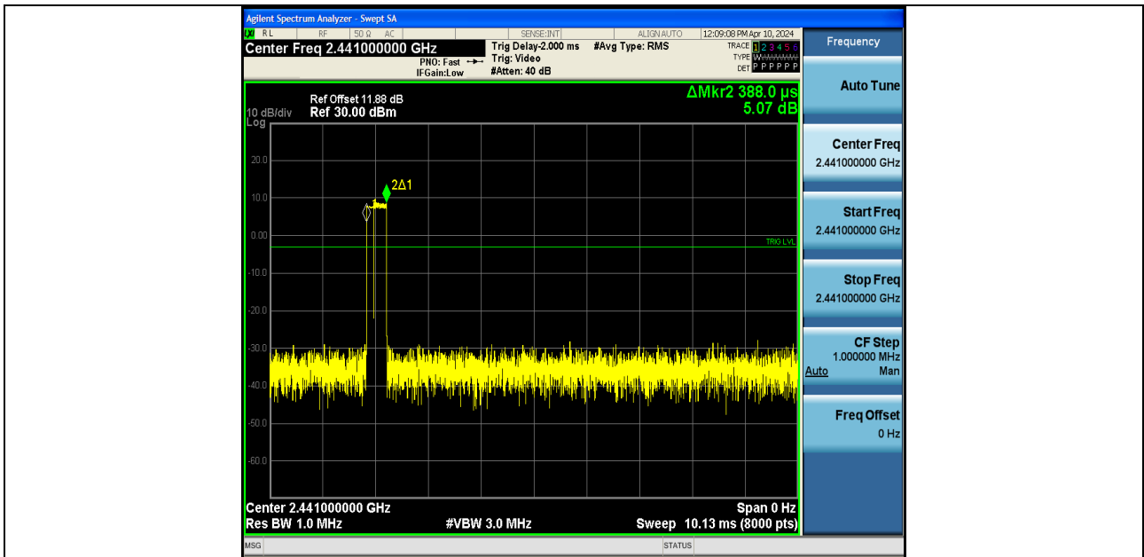
2DH1-Ant1-Hop-PASS
