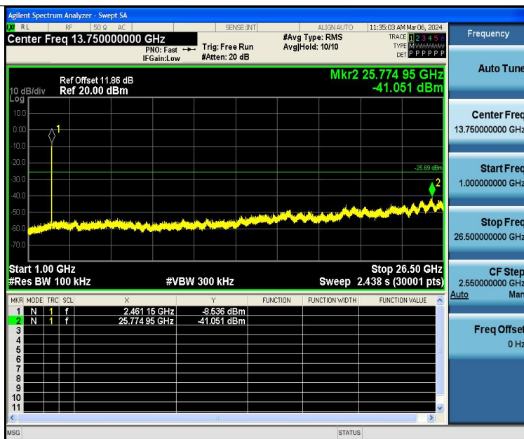
11G-Ant1-2462-1000~26500-PASS
