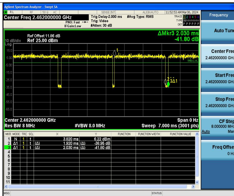
NTNV-11N20SISO-Ant1-2462
