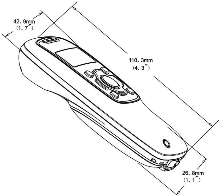
Figure 1-2. Dimensions of the scanner
