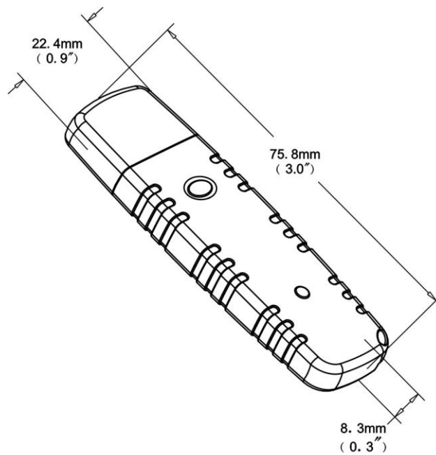
Figure 1-3. Dimensions of the Bluetooth USB adapter
