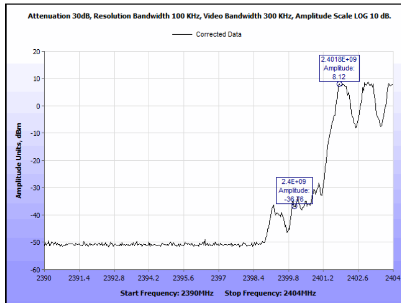
Conducted Band Edge, Low Hopping ON
