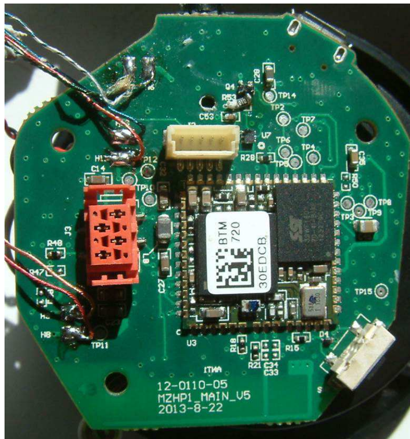
Main PCB view with Bluetooth module
