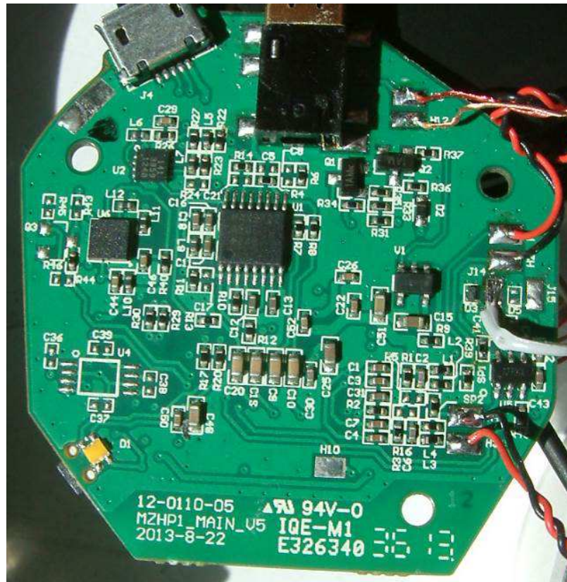
Main PCB view (Upper view)
