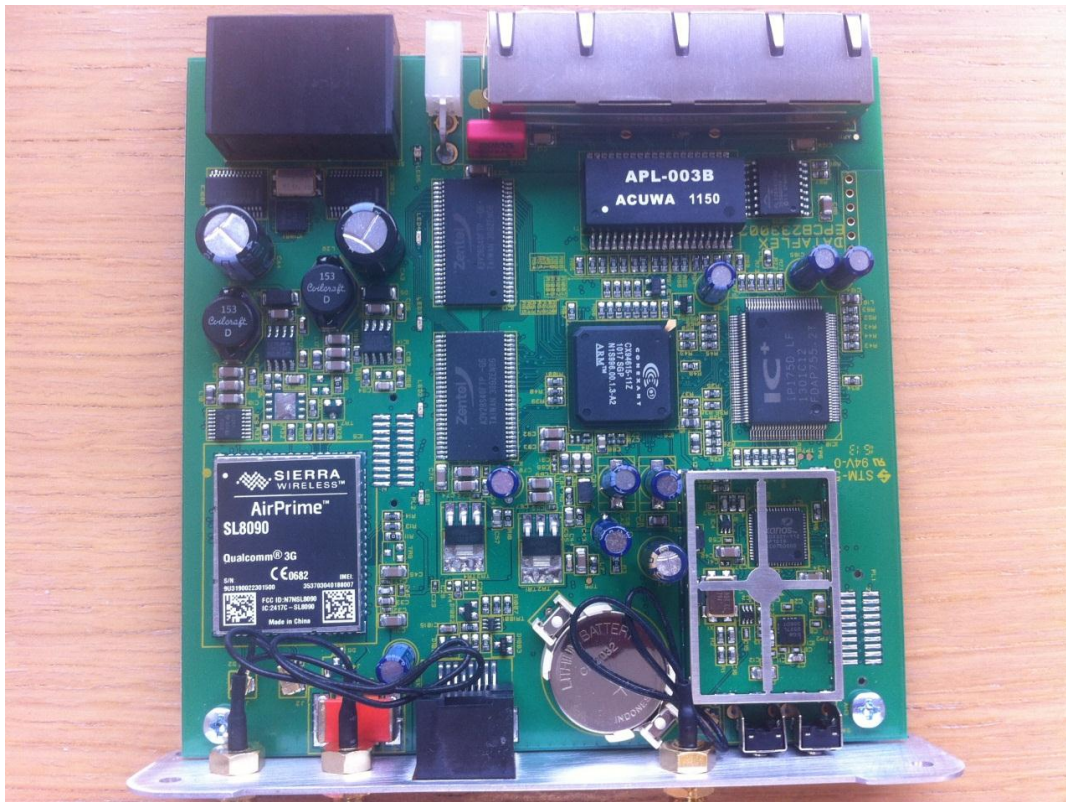
Figure 1: Hera601 PCB Top
