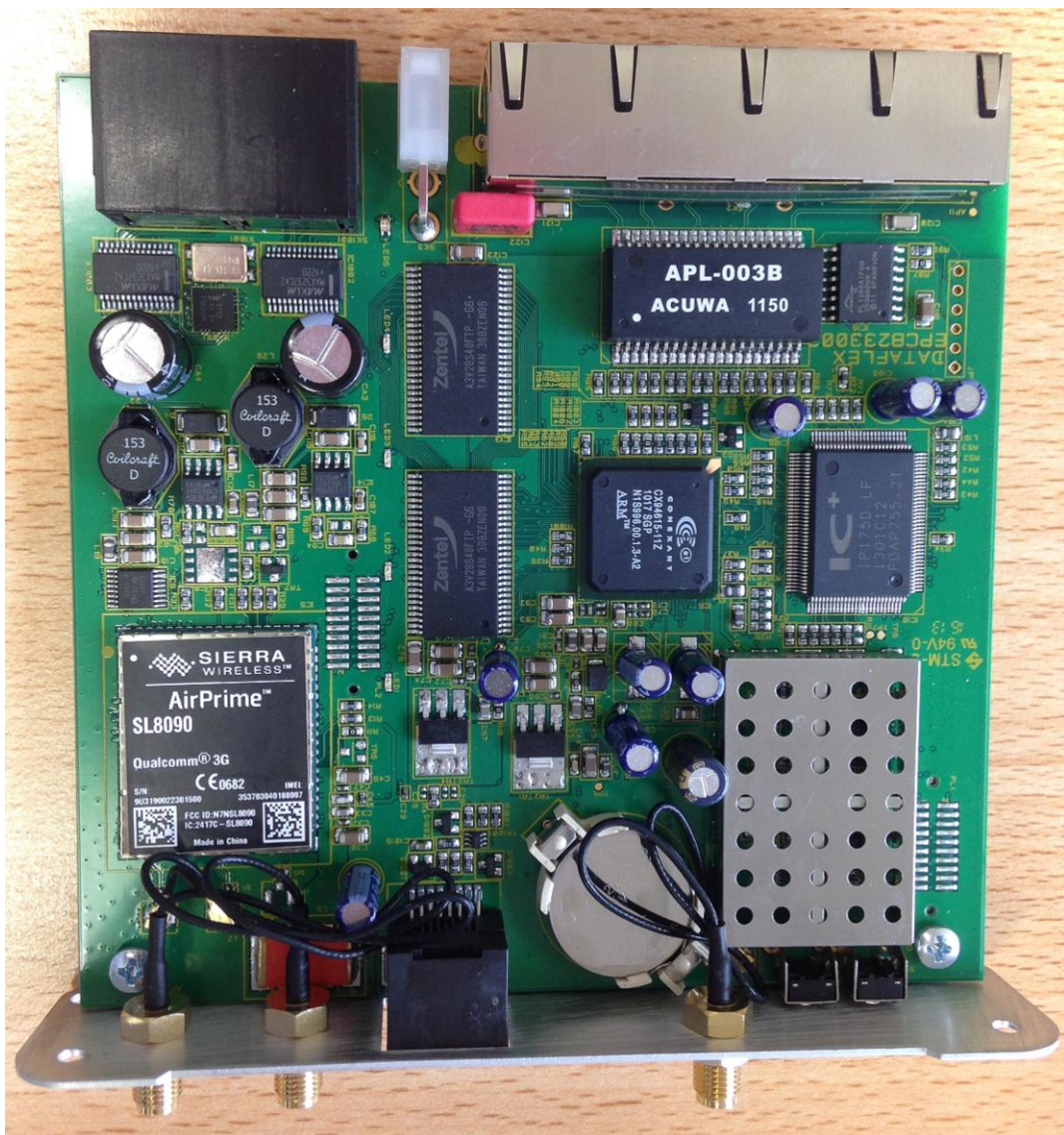
Figure 2: Hera601 PCB Top with WiFi Screen Fitted
