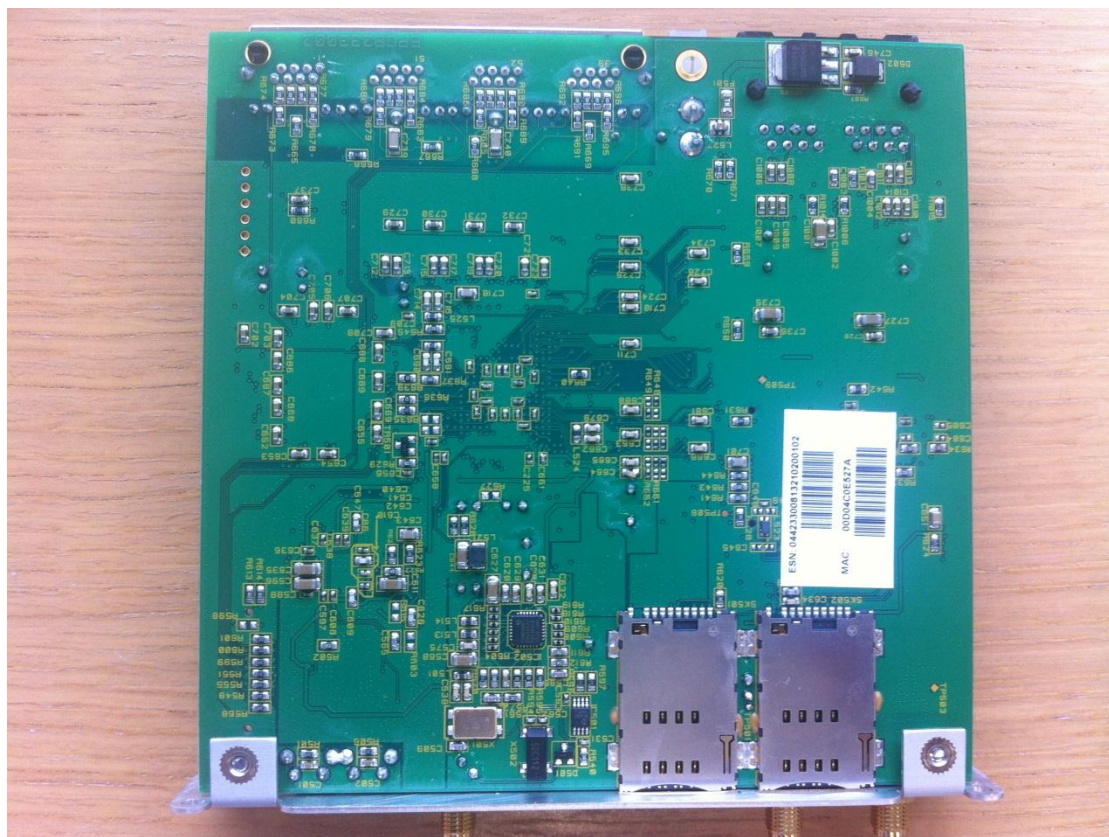
Figure 3: Hera601 PCB Bottom
