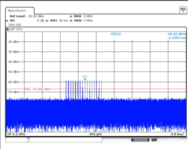
Radar #5 DFS detection threshold level
