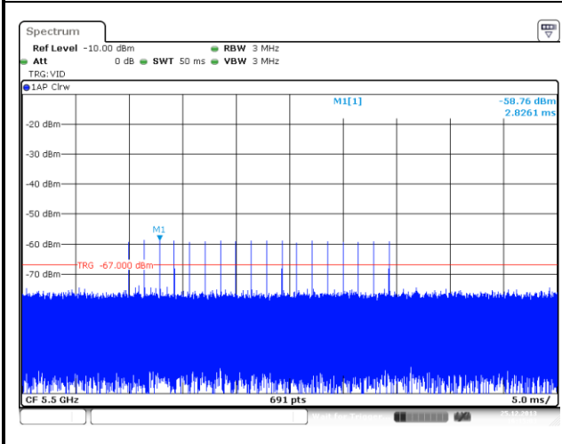
Radar #2 DFS detection threshold level
