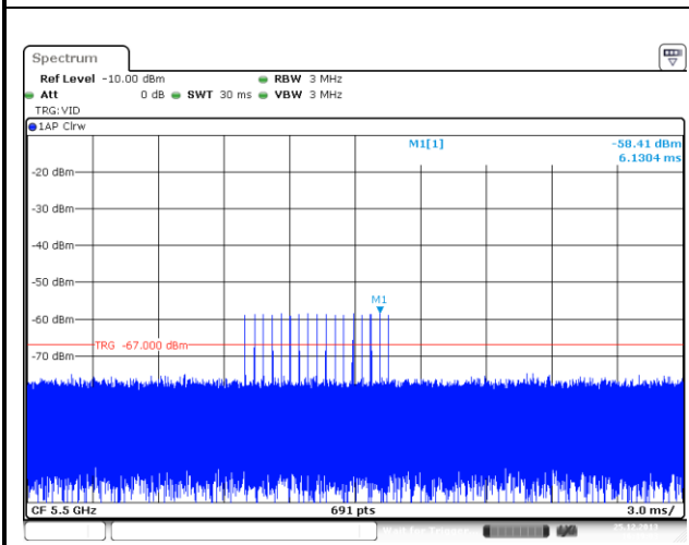
Radar #3 DFS detection threshold level
