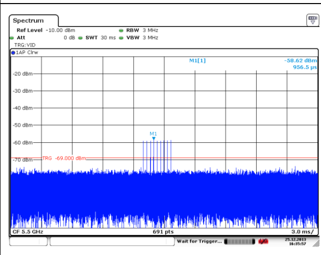
Radar #6 DFS detection threshold level
