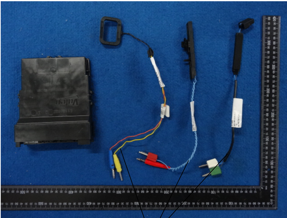
Antenna Location
