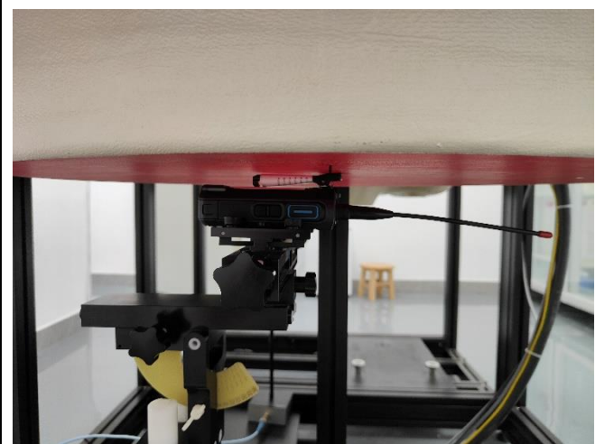
Body-worn(0mm)
