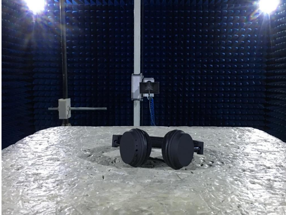
Photograph 3: Set-up for Spurious Emissions (1GHz-18GHz)
