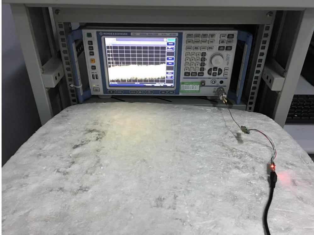
Photograph 5: Set-up for Radio Spetrum test
