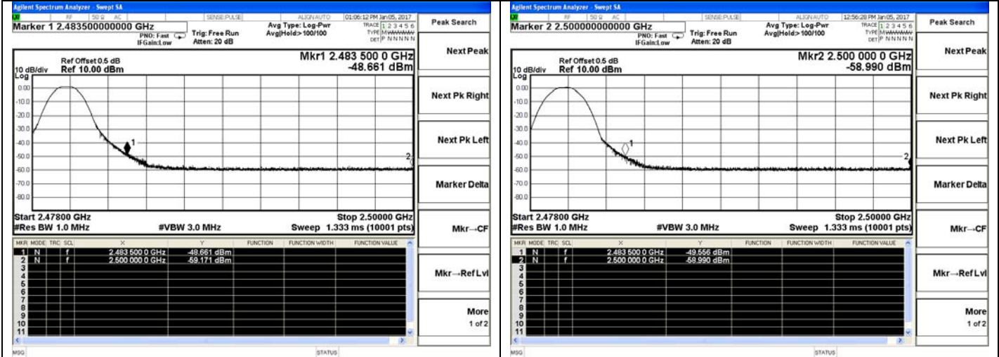
Channel 78 / 2480 MHz – Non-Hopping – Peak
