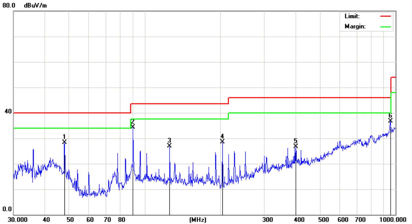
Quasi-peak measurement
