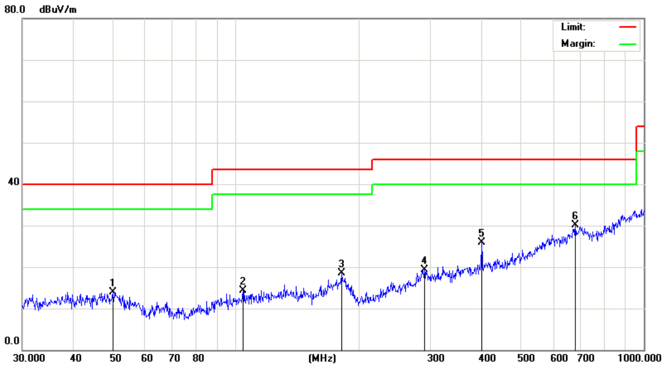
Quasi-peak measurement
