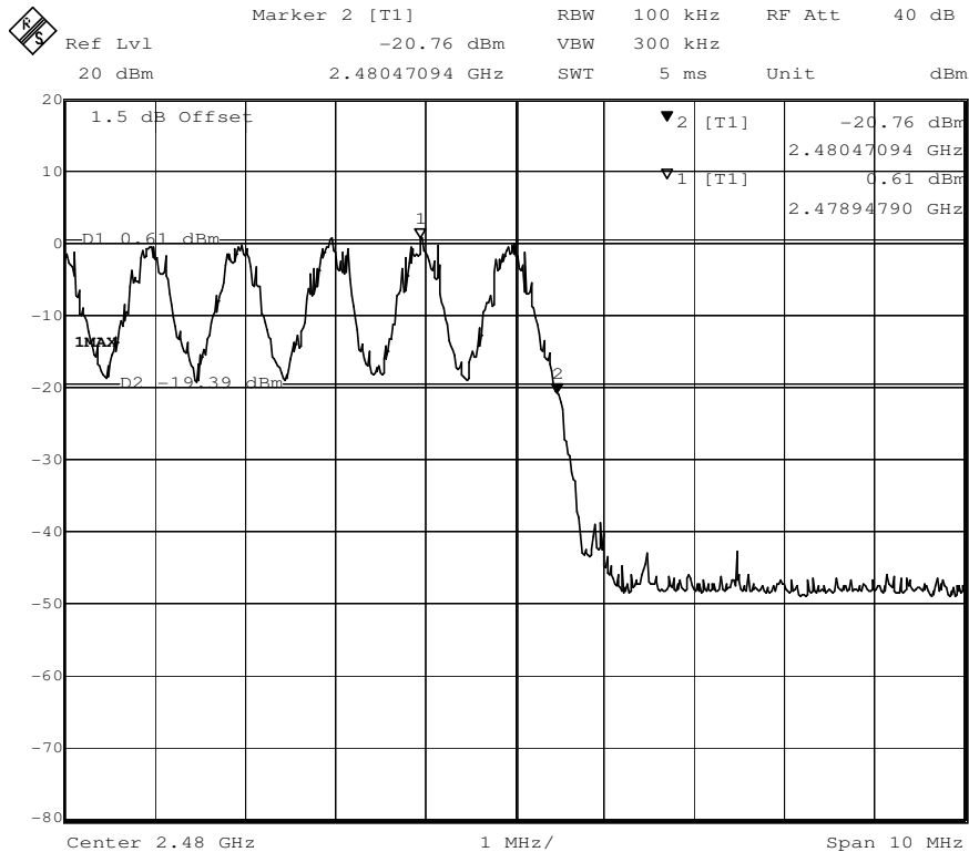
CH 78 (Upper) Data rate 1Mbps
