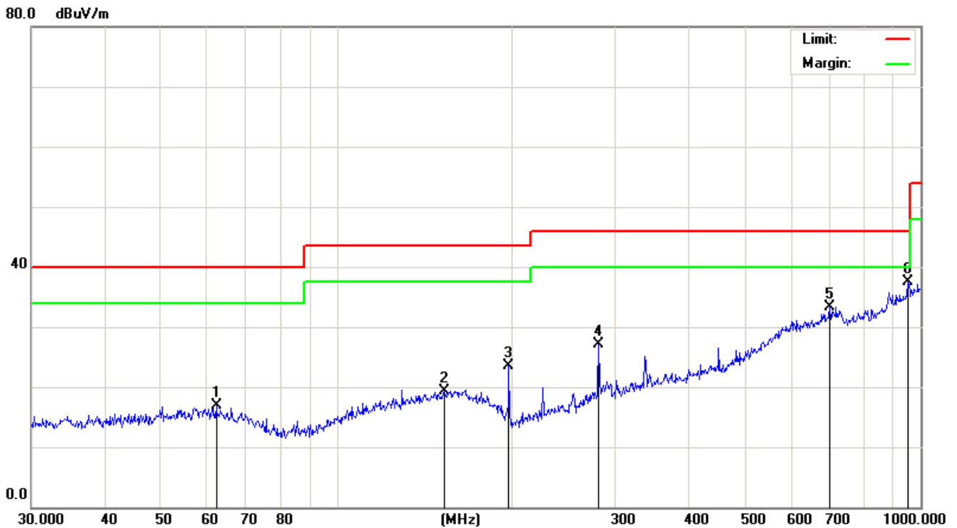
Quasi-peak measurement
