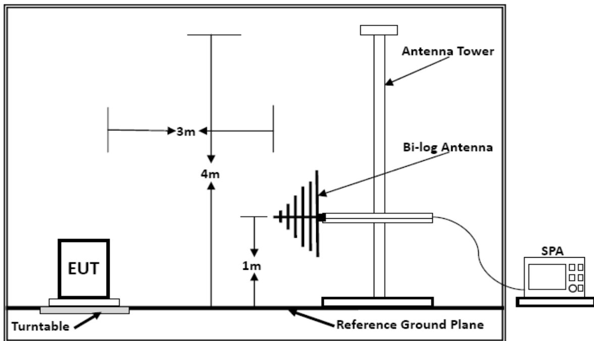
Below 1GHz
