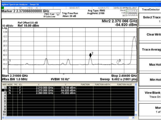
Channel 0 / 2402 MHz – Non-Hopping –AV
