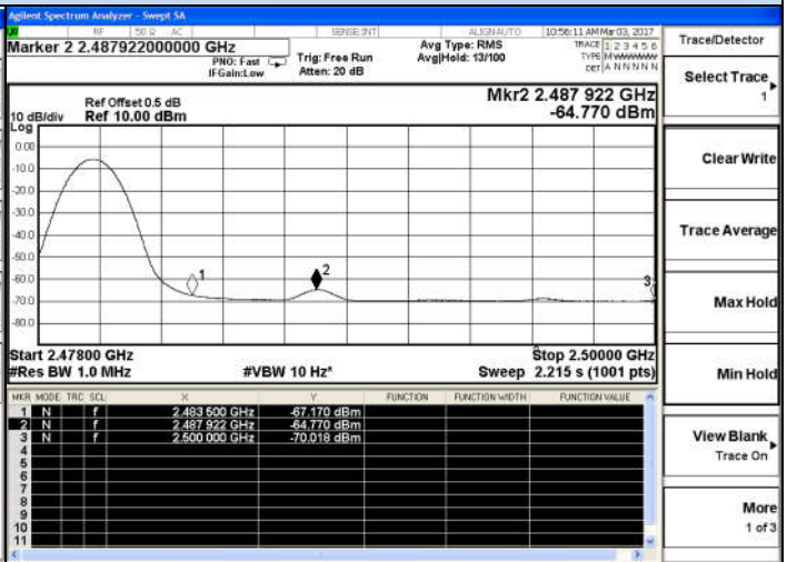
Channel 78 / 2480 MHz – Non-Hopping –AV
