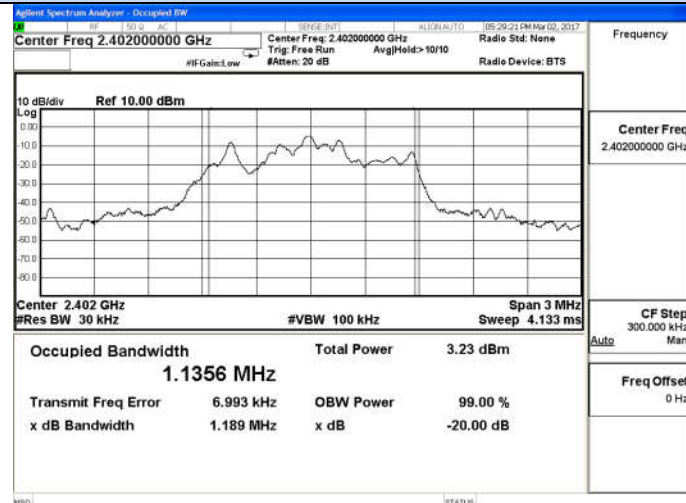
Channel 0 / 2402 MHz
