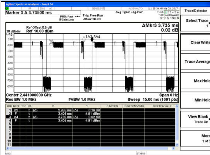
Channel 39 / 2441 MHz - 3DH5
