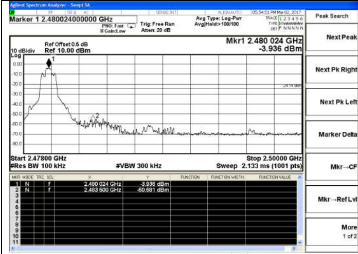
Channel 78 / 2480 MHz – Non-Hopping
