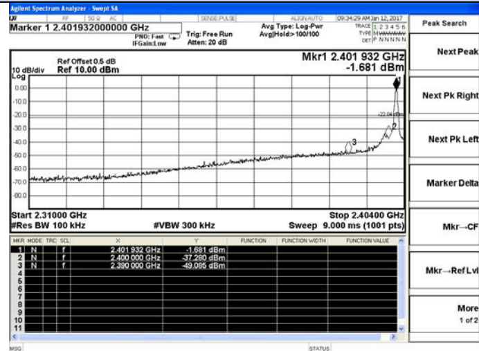
Channel 0 / 2401 MHz – Non-Hopping
